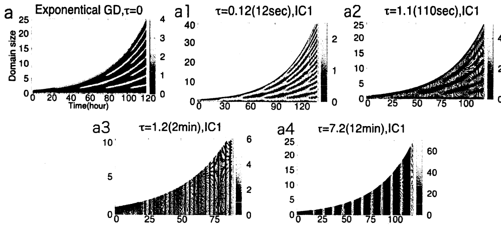
Figure 1: Model I-S. In the above plots results are presented for Model I-S, where morphogen-cell interactions are instigated on the cell surface via reversible ligand binding, with saturation of activator induced activator production. The horizontal axis in all plots represents time, in units of hours, and the vertical axis gives the domain size, in units of the initial domain length which corresponds to 10^{-2}\text{cm} or approximately 10 cell lengths. The label IC1 denotes the time-independent initial condition. The domain is exponentially growing with a growth parameter of \delta_{exp} = 0.0015 which corresponds to a doubling time of approximately 25 hours using the timescale T_s = 100 seconds. Finally note that the non-dimensionalised gene expression time delay, \tau , is given above each plot with its dimensional size in brackets.
