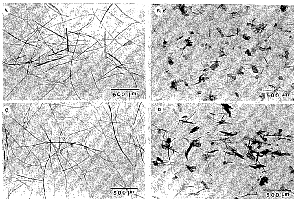
Fig. 4 Micrographs of holopulp fraction. Fraction retained on 100 mesh screen (A) and passed thorough (B) from stalk; fraction retained on 100 mesh screen (C) and passed thorough (D) from leaf stem.
