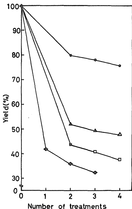
Fig. 2 Holopulp yield for chlorite (●), chlorite-sodium hydroxide (20 ml/g, ▲; 60 ml/g, ■), and peracetic (◆) methods. Solid symbols indicate that the insolubles were difficult to defibrate, and open symbols completely defibrated.
