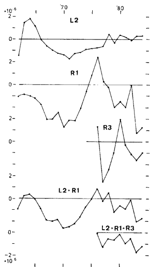
Fig. 4 (b) The curve of the yearly deviations from the linear changes of the extensions for the all periods. L2+R1 is the average for L2 and R1, and L2+R1+R3 is that of these three extensions.
