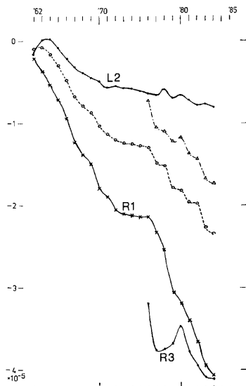
Fig. 4 (a) The curves of they early values of the extensions of L2, R1 and R3. L2+R1 and L2+R1+R3 are the average of the values of L2 and R1, and L2, R1 and R3, respectively.
