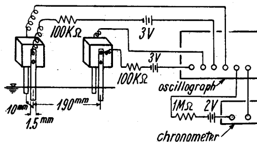
Fig. 2. Apparatus by which wave-trains were measured.
