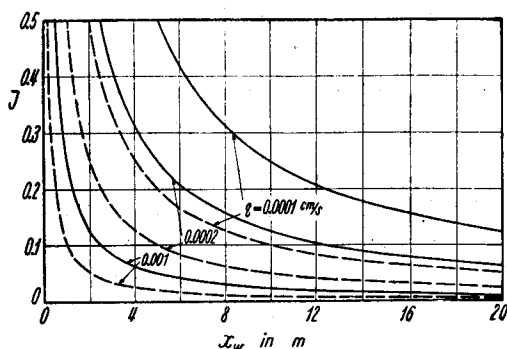
Fig. 8. Distance from the watershed to the place where wave-trains begin to appear.
