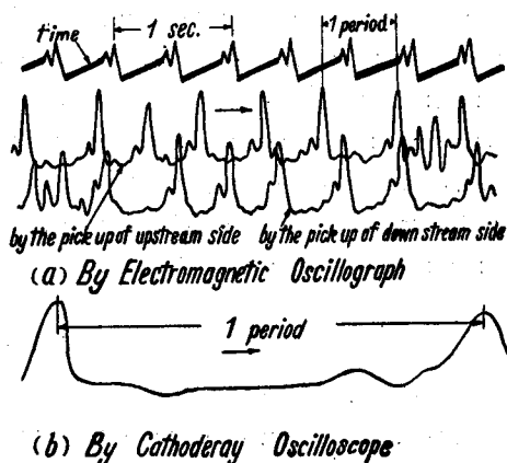
Fig. 3. Wave profiles of wave-trains recorded by an electromagnetic oscillograph and a cathodray oscilloscope.
