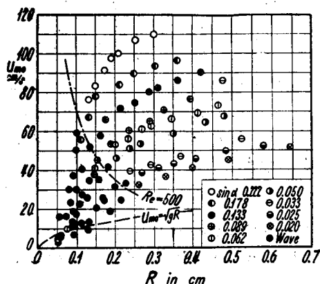
Fig. 1. Relation between mean velocity and hydraulic mean depth, and region where wave-trains appear, (plotted by black circles).
