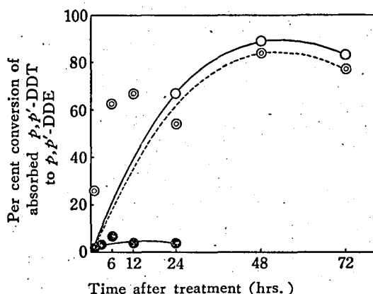
Fig. 2. Per cent of p,p' -DDT metabolized to p,p' -DDE in the DDT-resistant common cabbage worm which were administered 7.92 \mu g of p,p' -DDT per larva by sandwich method (—○—) or applied 396 \mu g of p,p' -DDT per larva topically (.....○.....) and the DDT-susceptible cabbage armyworm applied 19.8 \mu g of p,p' -DDT per larva topically (—●—) as the acetone solution.
