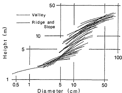
Fig. 5 Variation of D-H relation with the passage of time
