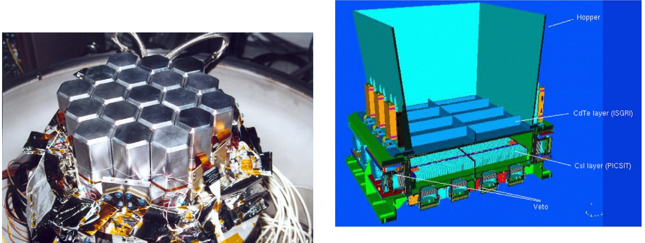
Figure 4.5: Schematic view of the SPI (left) and IBIS (right).
