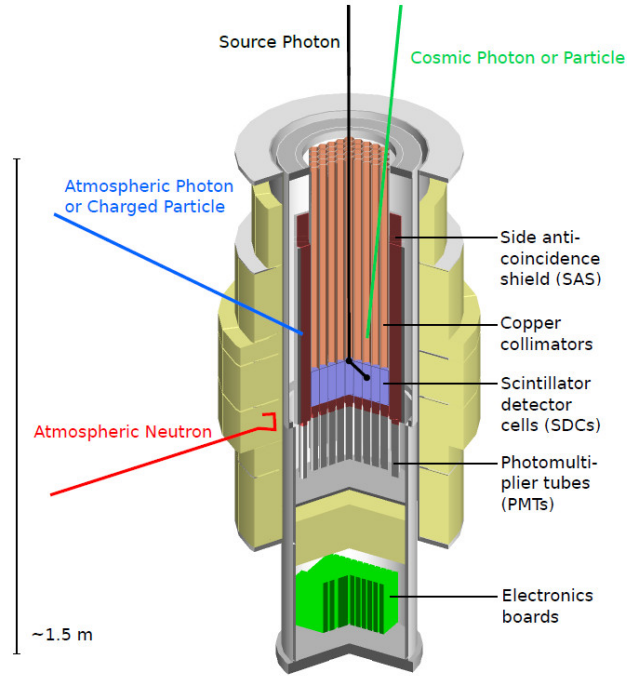
Figure 4.11: Schematic view of the PoGO+ polarimeter ( Chauvin et al., 2017 ).
