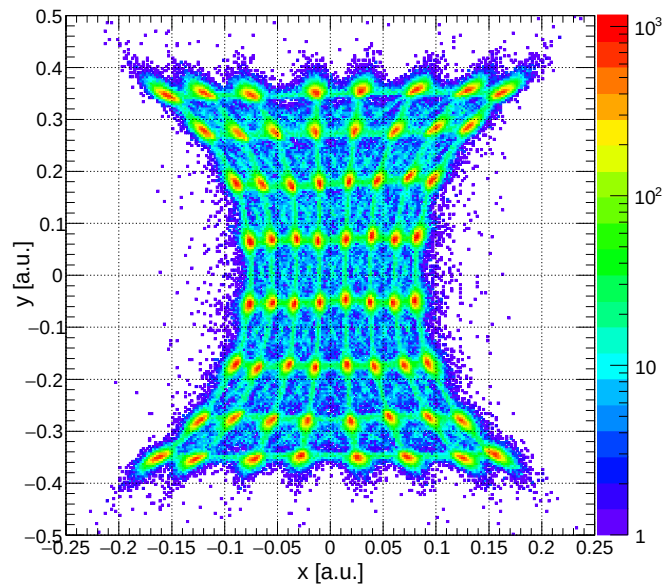
Figure 5.15: Reconstructed hit distribution image of the one unit of the PSA for the gamma rays with an energy of 662 keV ( Mizumoto et al., 2015 ).
