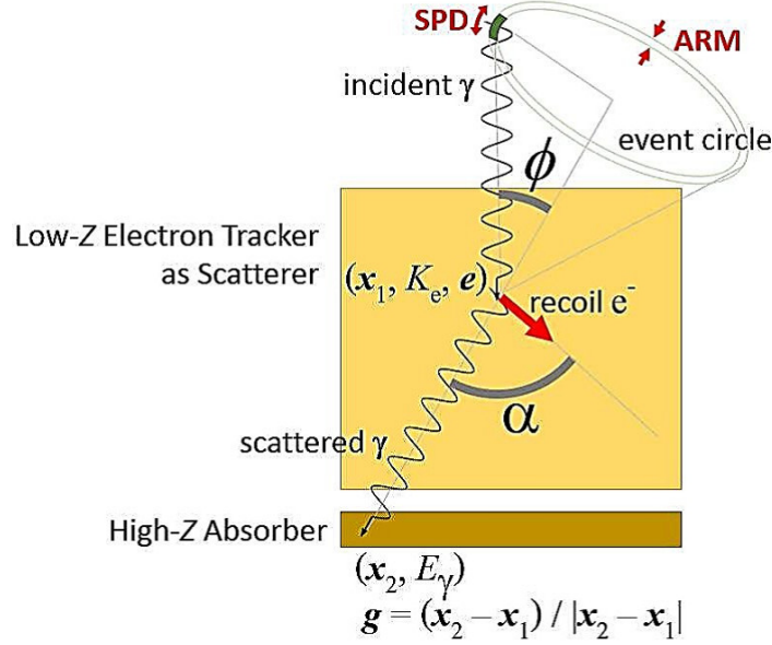
Figure 5.1: Schematic of an Electron-Tracking Compton Camera. It consists of an electron tracker as the scatterer made of low-Z material and an absorber made of high-Z material. The scatterer measures the scattering position \vec{x}_1 , and the kinematic energy and momentum unit vector of the recoil electron, \vec{e} and K_e , respectively. The absorber measures the absorption position \vec{x}_2 and energy of the scattered gamma ray E_\gamma . The momentum unit vector of the scattered gamma ray is obtained by calculating (\vec{x}_2 - \vec{x}_1)/|\vec{x}_2 - \vec{x}_1| Figure from Sawano (2017) .
