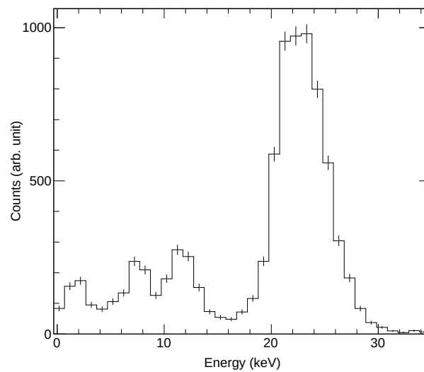
Figure 5.10: Spectrum obtained by irradiation of radioactive isotope source of ^{109}\text{Cd} . photoelectric peaks can be seen at \text{Ag K}\alpha ( 22.2 \text{ keV} ) from ^{109}\text{Cd} , and \text{Pb L}\alpha ( 10.6 \text{ keV} ), \text{Cu K}\alpha ( 8.0 \text{ keV} ) and possibly \text{Ar K}\alpha ( 3.0 \text{ keV} ) from the materials that are used for the TPC ( Sawano, 2017 ).
