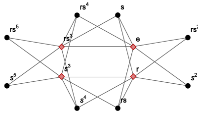
Figure 1: The pair-graph \mathcal{G}(G, H, S_1) .
