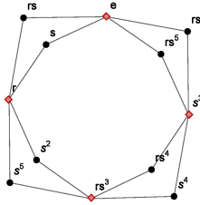
Figure 2: The pair-graph \mathcal{G}(G, H, S_2) .
