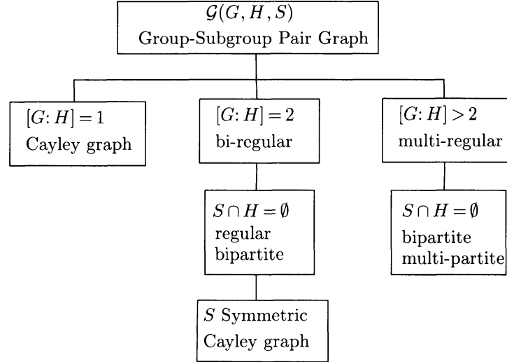
Figure 4: Characteristics of group-subgroup pair graphs.
