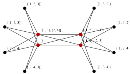
Figure 3: The bipartite pair-graph \mathcal{G}(G, H, S) .
