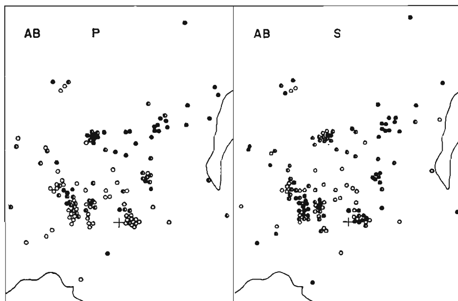
Fig. 5. Relations between epicenter locations and frequency contents of events observed at AB for P and S waves. Symbols are the same as those in Fig. 4.
