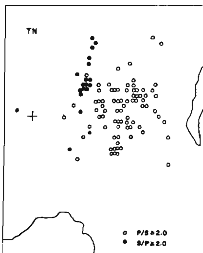
Fig. 15. Regional variation of the ratios of P - to S -maximum amplitude obtained from TN data. Symbols are the same as those in Fig. 12.
