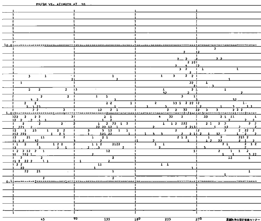
Fig. 19. Azimuthal distribution of the ratios of P - to S -maximum amplitude obtained from YG data.
