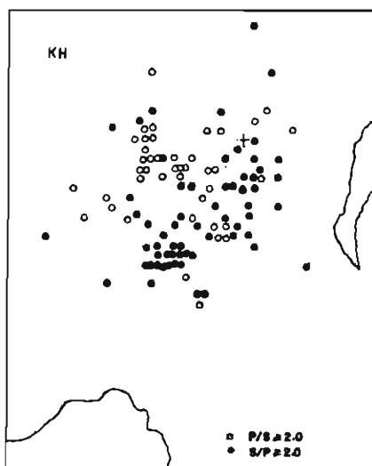
Fig. 14. Regional variation of the ratios of P - to S -maximum amplitude obtained from KH data. Symbols are the same as those in Fig. 12.
