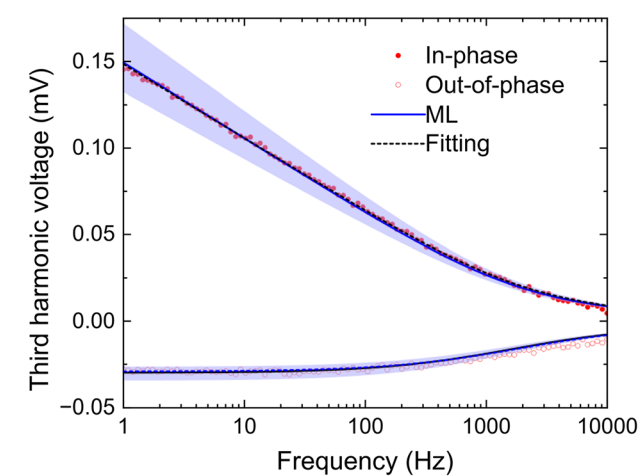
FIG. 3. Experimental signals of the third harmonic voltage. Filled markers represent in-phase component, and unfilled markers represent the out-of-phase component. The solid blue line represents the thermal model predictions based on the outputs from the ML model, while the dashed black line represents the fitting predictions. The shaded region around the solid blue line indicates the 95% confidence interval derived from prediction uncertainty.
