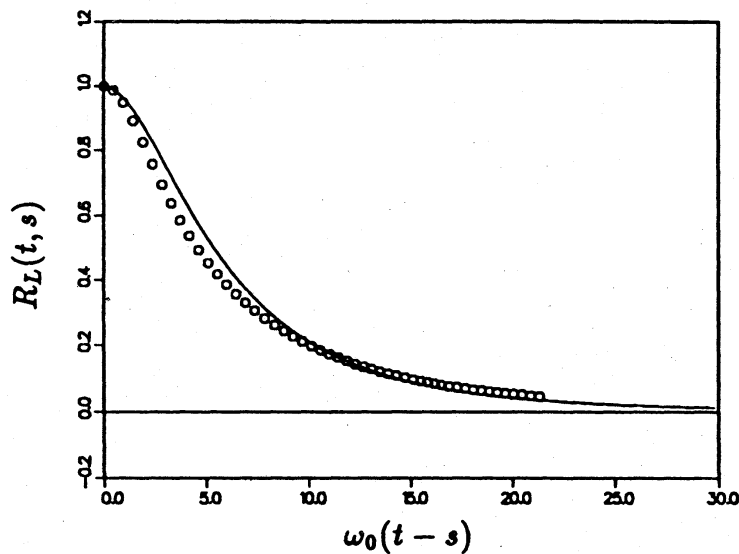
FIGURE 18. Comparison of R_L(t, s) for the MLRA and DNS. — MLRA, \circ DNS.
