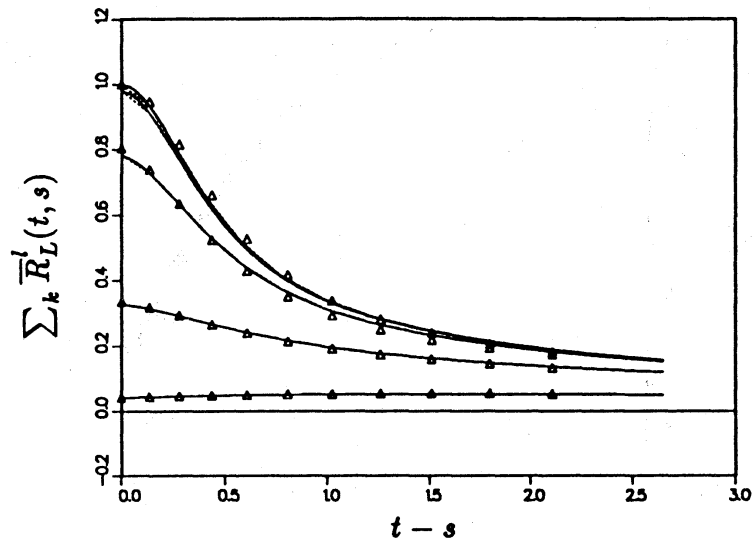
FIGURE 6. Contribution of octave bands to R_L(t, s) for different K_{maz} for run A. The lowermost curve corresponds to the lowest octave, and the partial sum increases monotonically with the addition of successive octaves.
