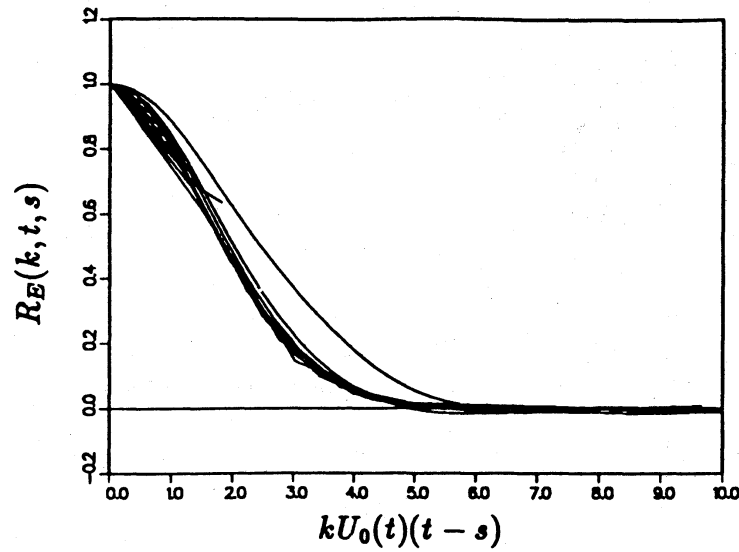
FIGURE 13. Time-scaled Eulerian correlations for bands k = 2 + 5n , n = 1, \dots, 11 for run SH. U_0 = \sqrt{E/3} .
