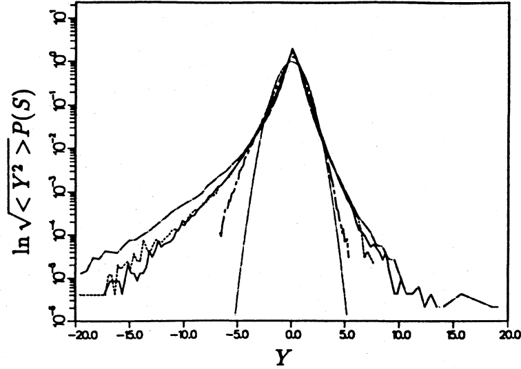
FIGURE 19. The PDF of Y = (u_{i,j})^2 - \langle (u_{i,j})^2 \rangle at t = s . — MLRA, --- run AH( t = \delta t ), ---- run BH, —·— run SH, ..... Gaussian.
