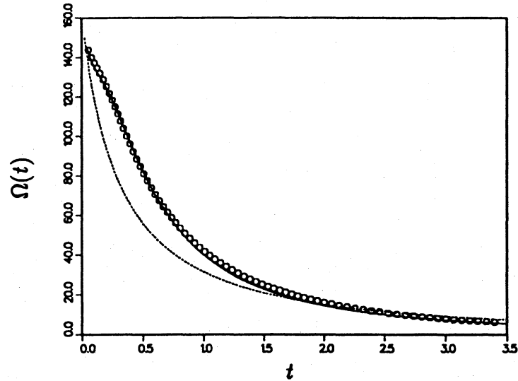
FIGURE 1. Evolution of the total enstrophy for run A. — MLRA, o DNS, ..... Linear decay.
