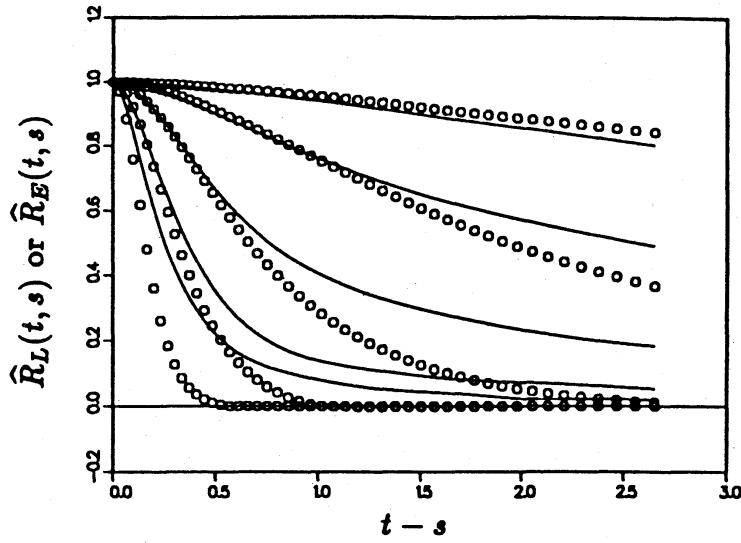
FIGURE 11. Comparison of decay of \hat{R}_L(t, s) and \hat{R}_E(t, s) for run A. Octave bands are 2^n < k < 2^{n+1} , n = 0, \dots, 4 and 32 < k < 60 from the uppermost line, respectively. — \hat{R}_L(t, s) , \circ \hat{R}_E(t, s) .
