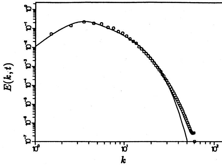
FIGURE 3. Comparison of the energy spectrum at s = 0.861 for run A. — MLRA, o DNS.
