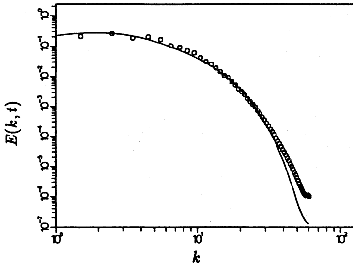
FIGURE 4. Comparison of the energy spectrum at s = 0.667 for run BH. — MLRA, o DNS.
