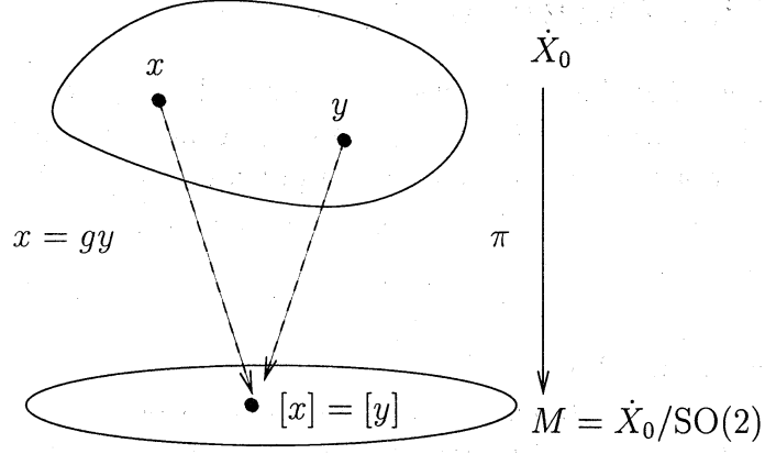
Figure 5: The projection \pi takes two equivalent configurations to the same equivalent class in M . In reality, x and y are on the same fiber.
