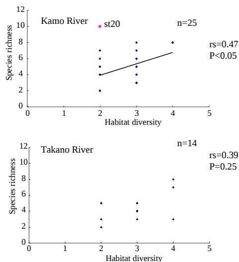
Fig.10 Relation of fish species richness to habitat diversity in the two rivers.
