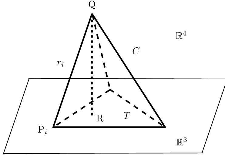
Figure 9. 4-dimensional cone C over the tetrahedron T
