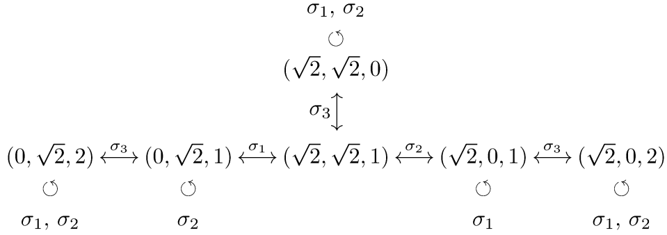
Figure 7. A finite orbit of degree 6 on the stratum of type A_1^{\oplus 2}
