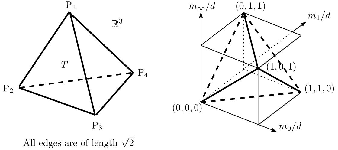
Figure 8. Tetrahedron for the Tetrahedral Theorem
