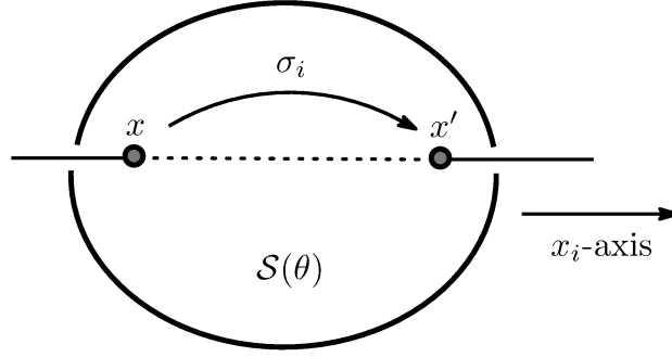
Figure 1. Involutions on the (2, 2, 2) -surface \mathcal{S}(\theta)
