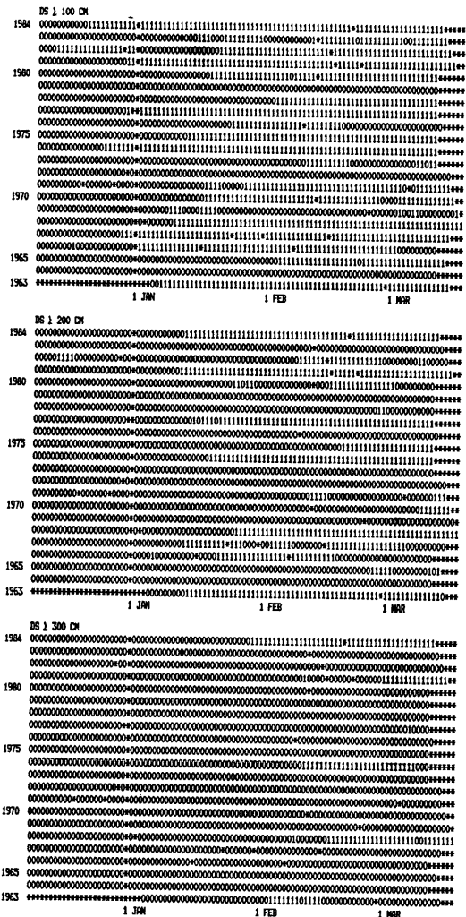
Fig. 4 The year to year change of daily snow depth at Hakodateyama. (1) shows the depth exceeds the standard level (100,200,300cm) otherwise (0).
