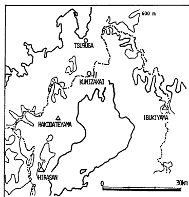
Fig. 3 Northern part of the Lake Biwa Basin and the mountain station for snow depth
