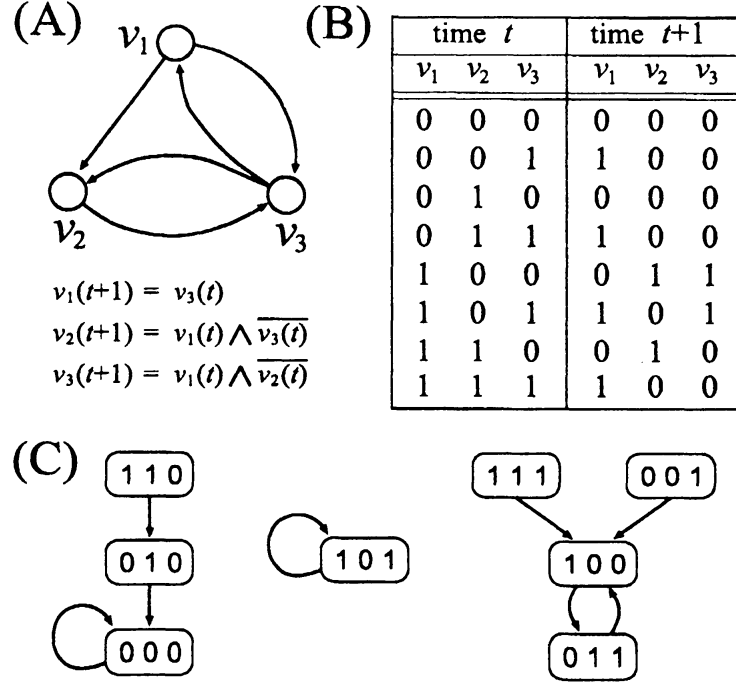
Figure 1: Example of a Boolean network. Dynamics of BN (A) is well-described by a state transition table (B) and by a state transition diagram (C).
