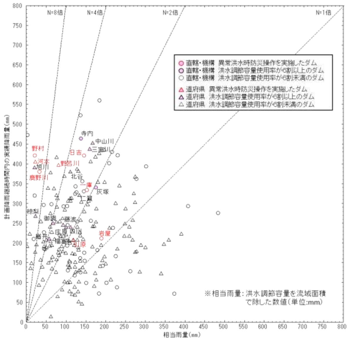
Fig. 6 Relationships between equivalent rainfall and observed rainfall over the duration time of the designed flood of dam reservoirs governed by the Japan Ministry of Land, Infrastructure, Transport and Tourism (異常豪雨の頻発化に備えたダムの洪水調節機能に関する検討会 (2018)).
