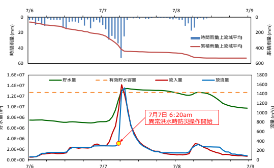
Fig. 2 Flood control operation by the Nomura Dam
