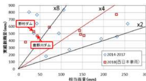
Fig. 4 Relationships between equivalent rainfall and observed rainfall of the dam reservoirs which carried out emergency spillway gate operation.
