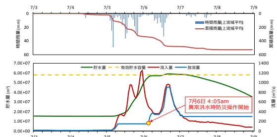
Fig. 3 Flood control operation by the Hiyoshi Dam
