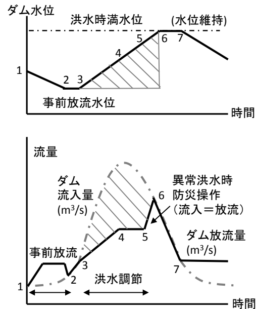
Fig. 1 Typical flood control operation of a dam
