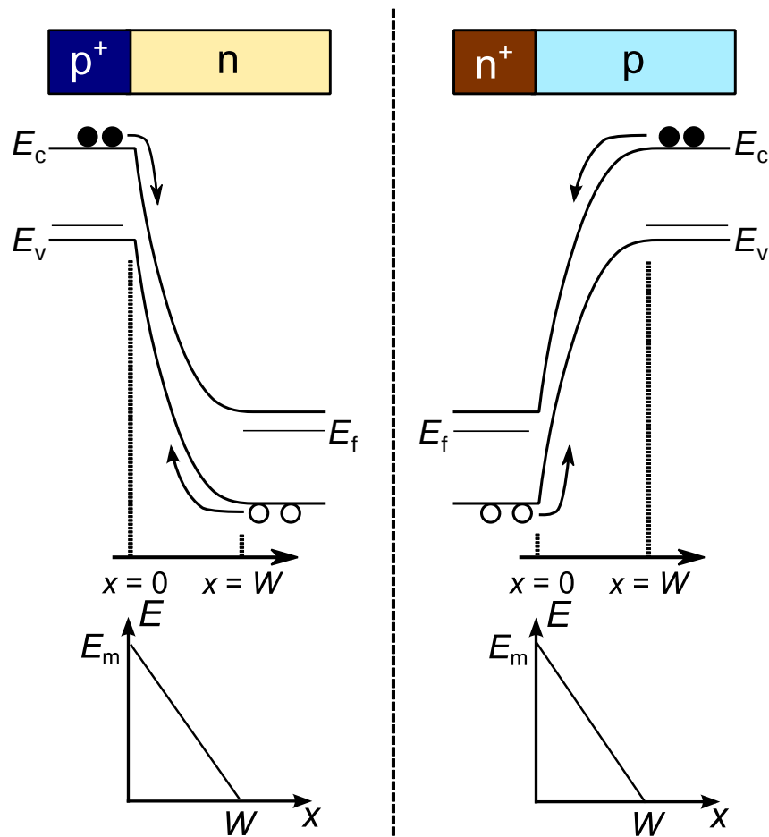
Figure 2.41: Schematic illustration of band diagram and electric field distribution at reverse bias for p^+n and n^+p diodes.
