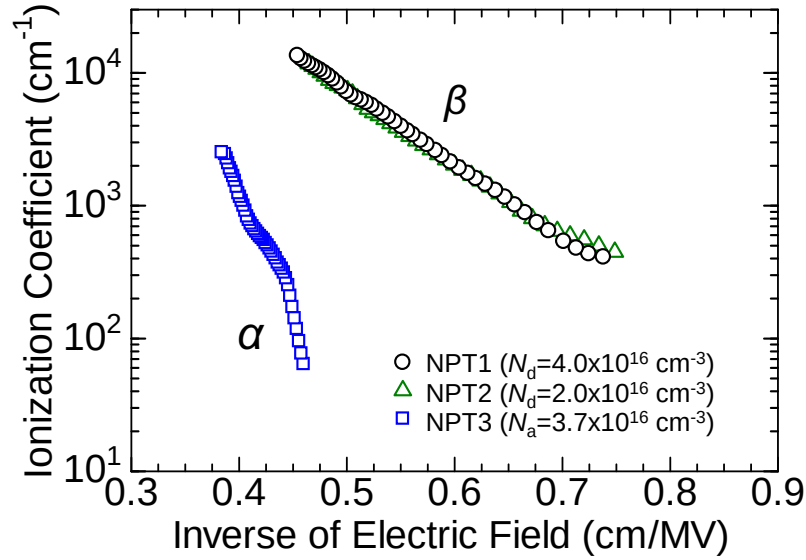
Figure 2.20: The extracted impact ionization coefficients from NPT1–3 at room temperature.
