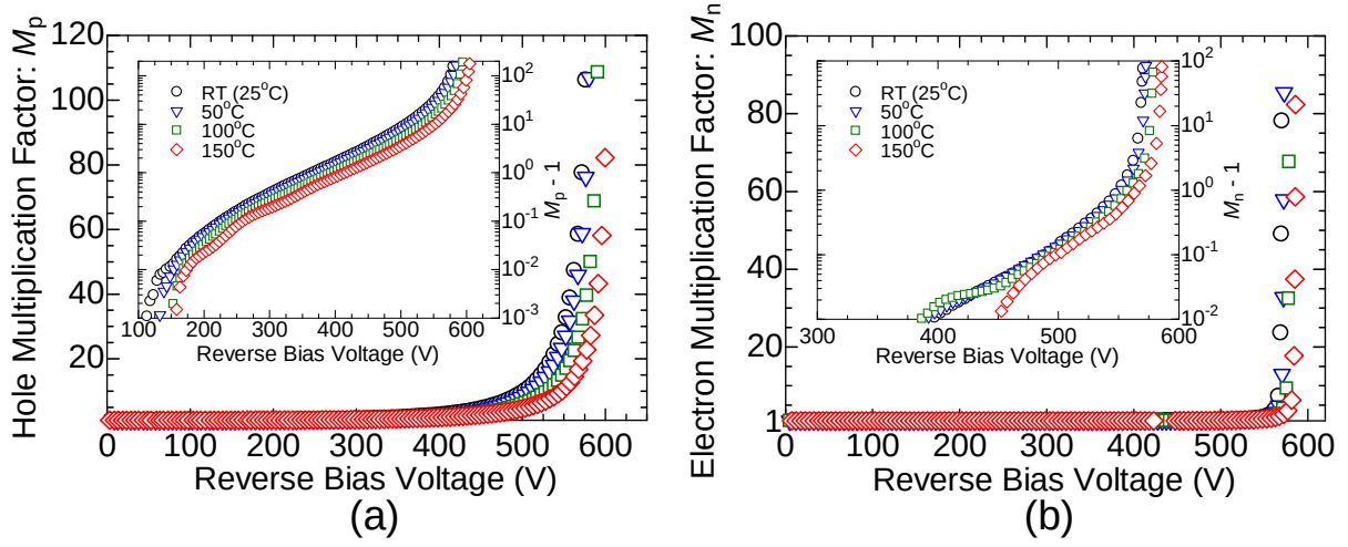
Figure 2.34: Reverse bias voltage dependence of multiplication factors at elevated temperatures up to 150°C. The inset shows the plot of M - 1 on a logarithmic scale. (a) NPT1: measurement of M_p . (b) NPT3: measurement of M_n .
