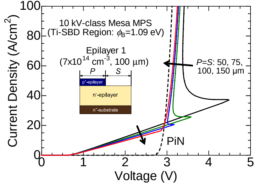
Figure 4.20: Simulated forward I - V characteristics of 10 kV-class MPS diodes (Epilayer 1) with various PiN diode region widths ( P ).
