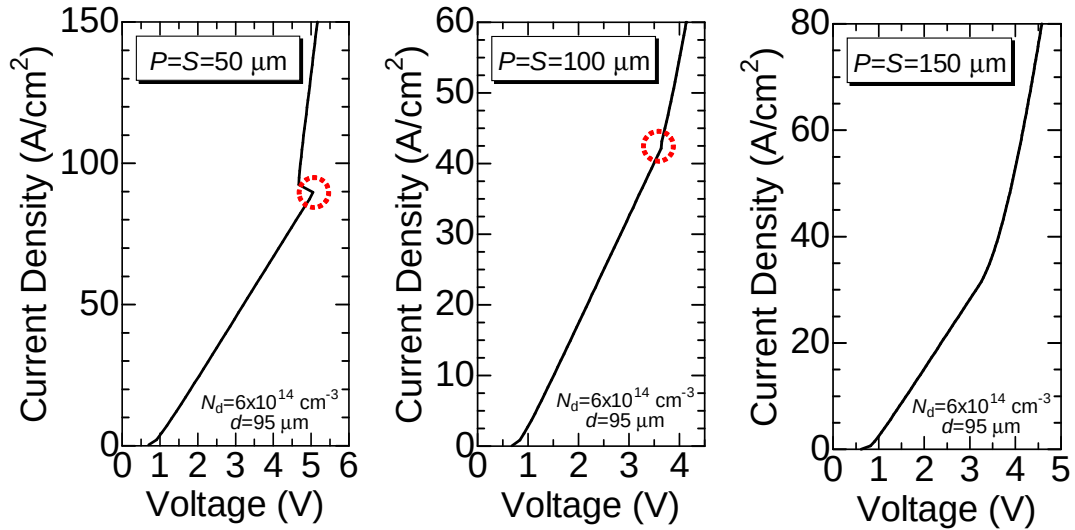
Figure 4.27: Forward I-V characteristics of MPS diodes with Type A epilayer for P -width of 50, 100, 150 \mu\text{m} .
