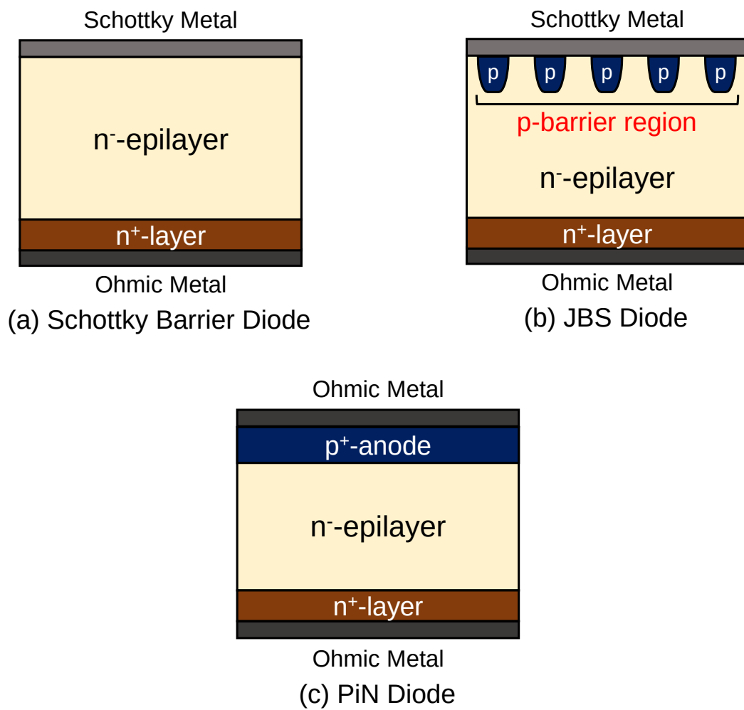
Figure 1.4: Schematic illustration of (a) SBD, (b) JBS, and (c) PiN diodes.
