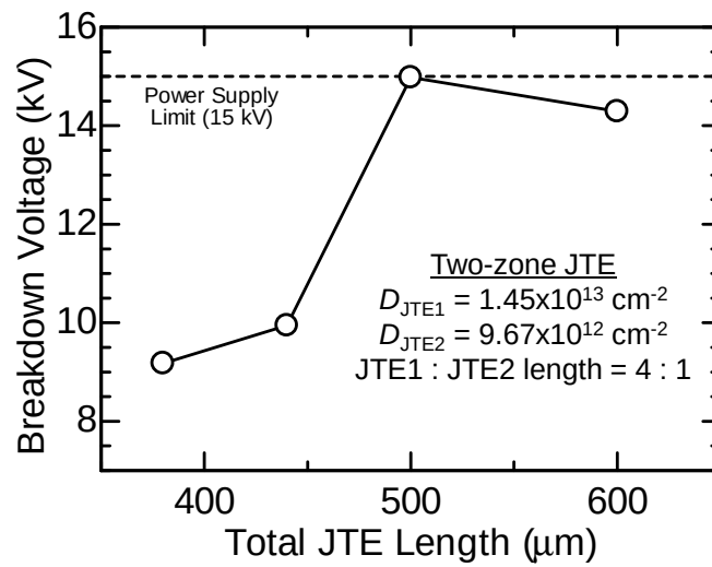
Figure 3.9: Total JTE-length dependence of the breakdown voltage for PiN diodes with two-zone JTE ( D_{\text{JTE1}} = 1.45 \times 10^{13} \text{ cm}^{-2} ).
