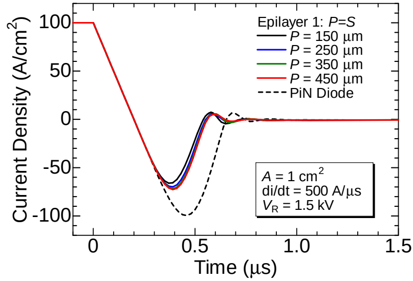
Figure 4.44: Simulated reverse recovery characteristics of MPS diode and PiN diode.
