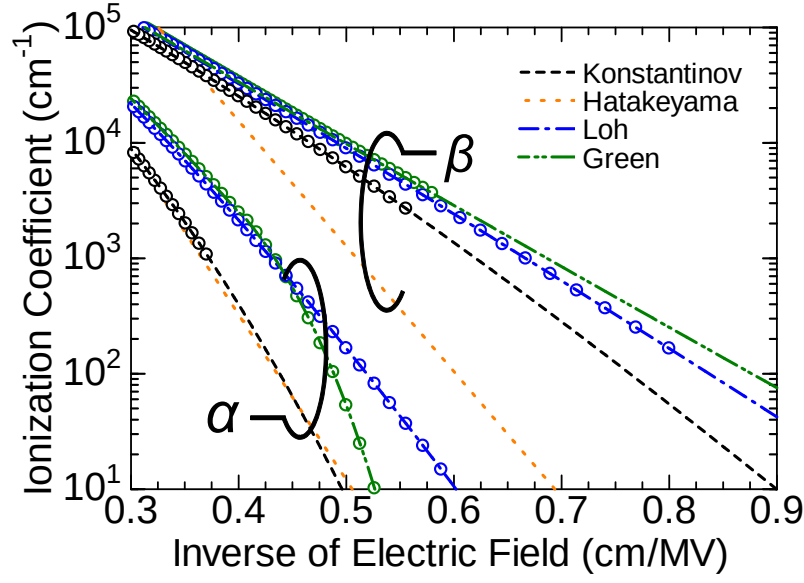
Figure 1.6: Some of the reported impact ionization coefficients in SiC [146, 148–150]. Here, \alpha and \beta are electron and hole impact ionization coefficients, respectively. Symbols: measured ionization coefficients. Lines: calculation result of the fitting equations.
