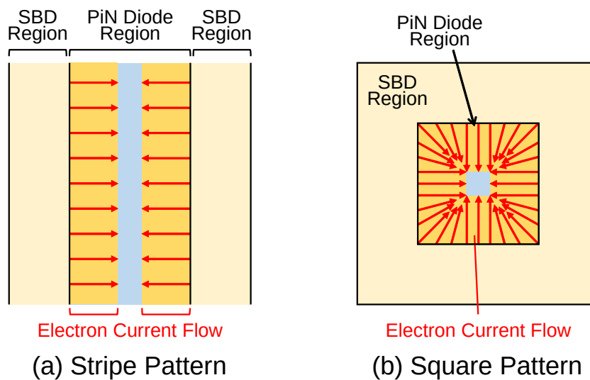
Figure 4.32: Schematic illustration of the unit cell structure and electron current flow for (a) stripe and (b) square patterns.
