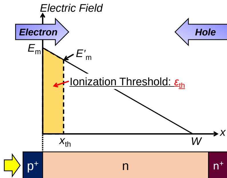
Figure 2.16: Schematic illustration of the dead space effect occurring in a p^+n NPT diode.
