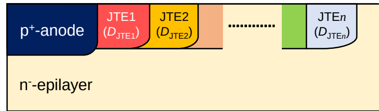
(c) Multi-zone JTE ( D_{\text{JTE1}} > D_{\text{JTE2}} > \dots > D_{\text{JTE}_n} )
