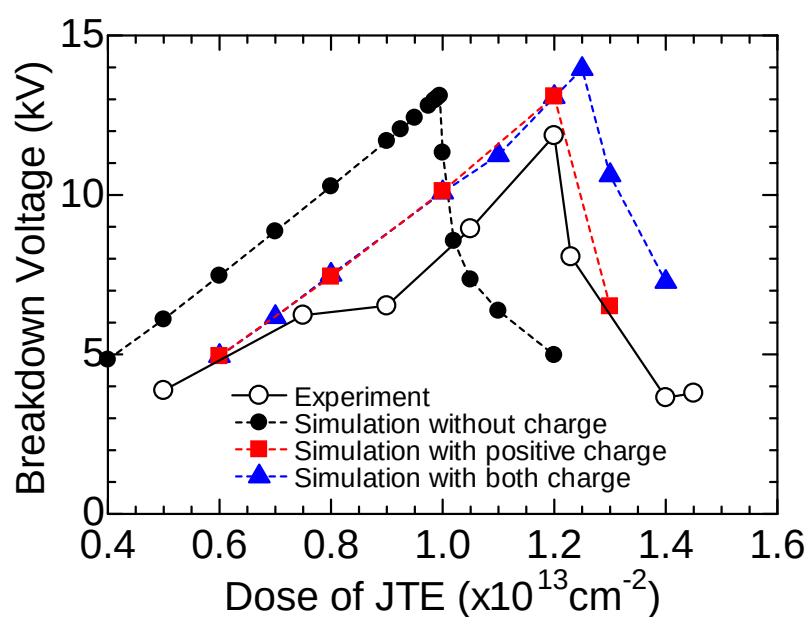
Figure 3.14: Experimental and simulated JTE dose dependence of breakdown voltage of PiN diodes with single-zone JTE. Positive charge ( +2 \times 10^{12} \text{ cm}^{-2} ) at the \text{SiO}_2/\text{p-SiC} interface, and/or negative charge ( -1.4 \times 10^{12} \text{ cm}^{-2} ) at the \text{SiO}_2/\text{n-SiC} interface were assumed in the simulation.
