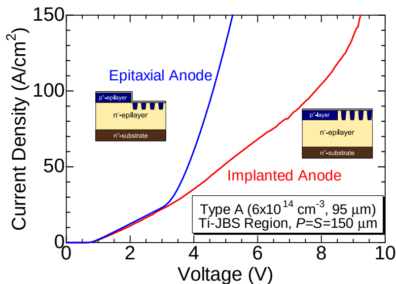
Figure 4.39: Measured forward I - V characteristics of MPS diodes with implanted and epitaxial p^+ -anode.
