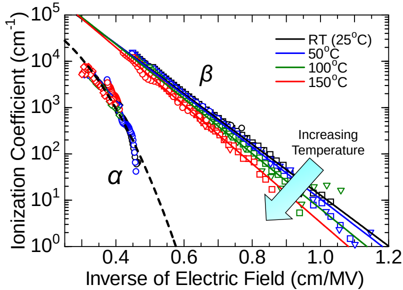
Figure 2.35: Measured ionization coefficients (symbols) and the modeled results using Okuto-Crowell model (lines) obtained at elevated temperatures.
