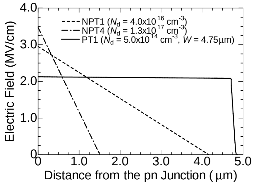
Figure 2.7: Electric field distribution inside the depletion layer of NPT1, NPT4, and PT1 at breakdown voltage.
