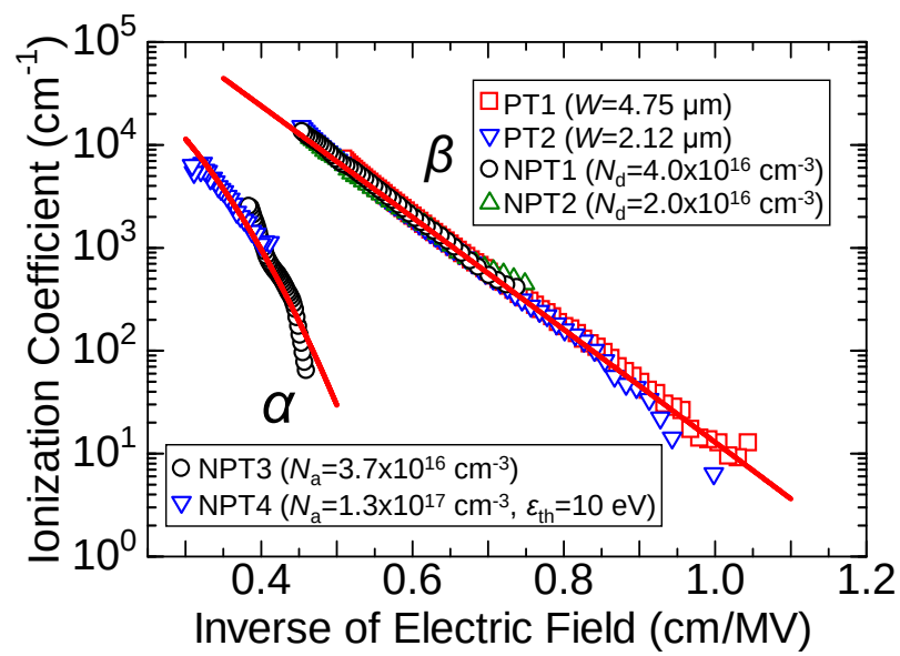
Figure 2.29: Fitting of ionization coefficients obtained in this work using modified Chynoweth's expression.
