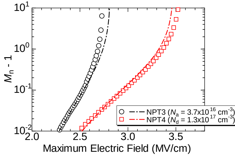
Figure 2.22: Maximum electric field dependence of M_n - 1 obtained from NPT3 and NPT4. Here, symbols show the measurement results, and lines show the simulated M_n - 1 using ionization coefficients obtained in this study.
