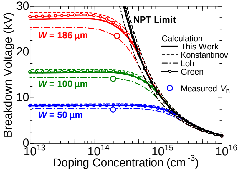
Figure 2.31: Simulated doping concentration dependence of ideal breakdown voltage and experimental results for PiN structures with various i-layer thicknesses. Experimental results were obtained from PiN diodes and BJT with appropriate edge termination, and calculation was done using ionization coefficients obtained from this study and [1, 5, 7, 8].
