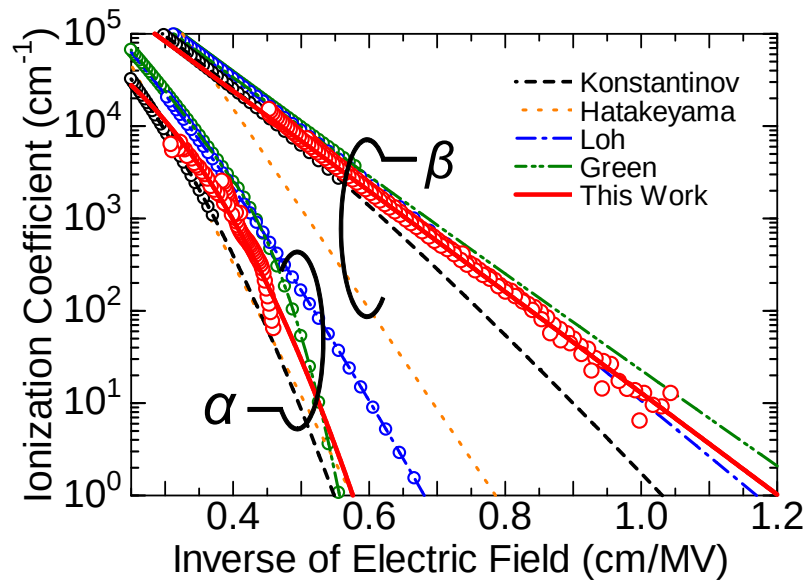
Figure 2.32: Ionization coefficients obtained in this study with results in [1, 5, 7, 8]. Symbols: extracted values from the experiment. Lines: calculation result of the fitting equations.
