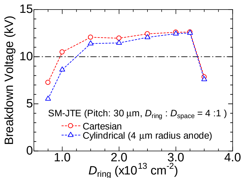
Figure 4.11: Simulated D_{\text{ring}} dependence of breakdown voltage in Cartesian and cylindrical coordinate.
