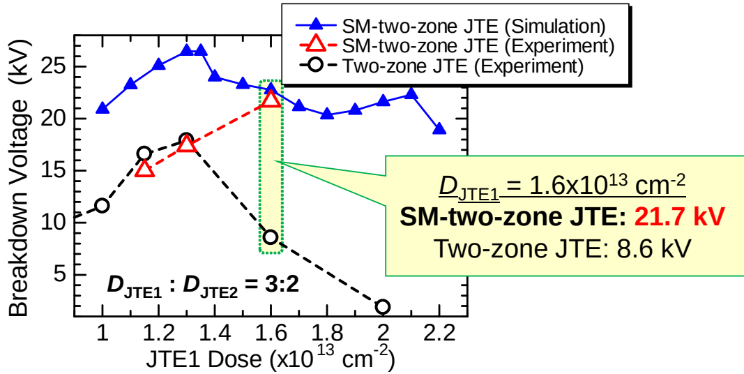
Figure 3.22: Experimental JTE1-dose dependence of breakdown voltage for SM-two-zone JTE and two-zone JTE, together with the simulation result of SM-two-zone JTE taking account of the interface charge.
