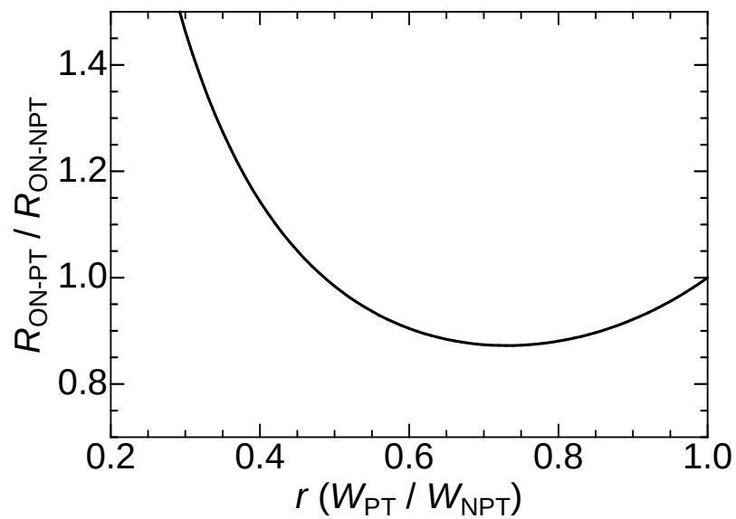
Figure 4.3: The ratio between on-resistance of PT and NPT as a function of ratio between the thickness of PT and NPT ( r ).
