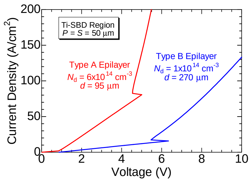
Figure 4.25: Measured forward I - V characteristics from fabricated MPS diodes with P = S = 50 \mu\text{m} for Type A and B epilayers.
