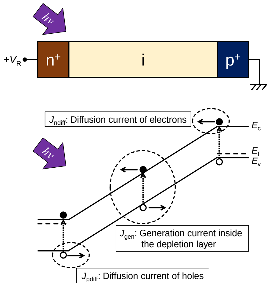
Figure 2.1: Schematic illustration of different current components of the measured photocurrent in a reverse biased photodiode.
