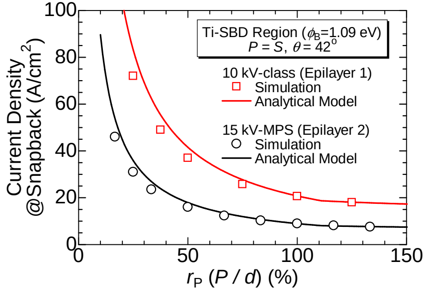
Figure 4.23: Simulated and analytical r_P dependence of snapback current ( J_{\text{snap}} ).
