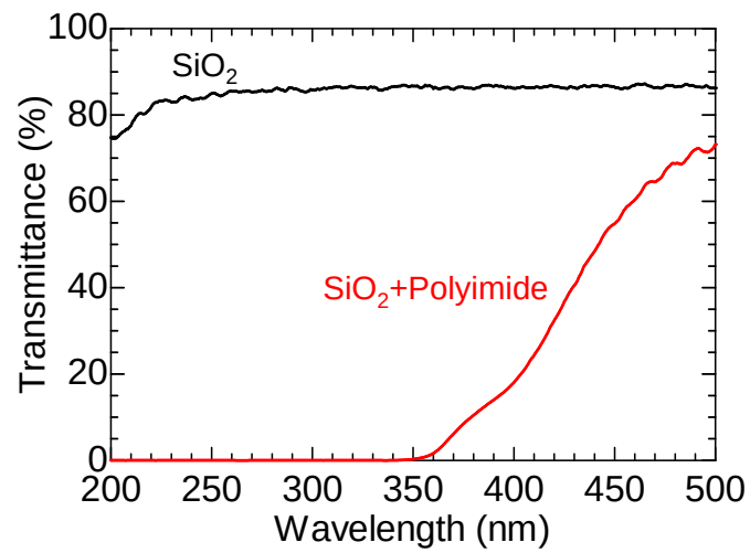
Figure 2.8: Transmittance characteristics of a polyimide used in this study.
