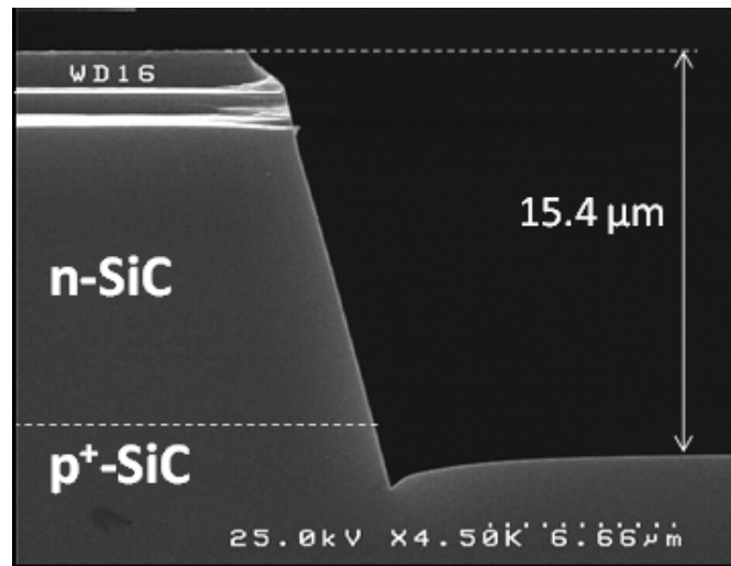
Figure 2.10: SEM image of a fabricated deep mesa by Cl 2 -based ICP-RIE.
