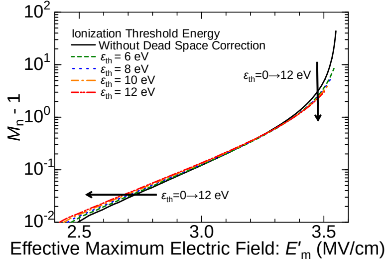
Figure 2.23: Effective maximum electric field ( E'_m ) dependence of “actual” multiplication factor M_{ni} calculated with various values of electron ionization threshold energy ( \epsilon_{th} ).
