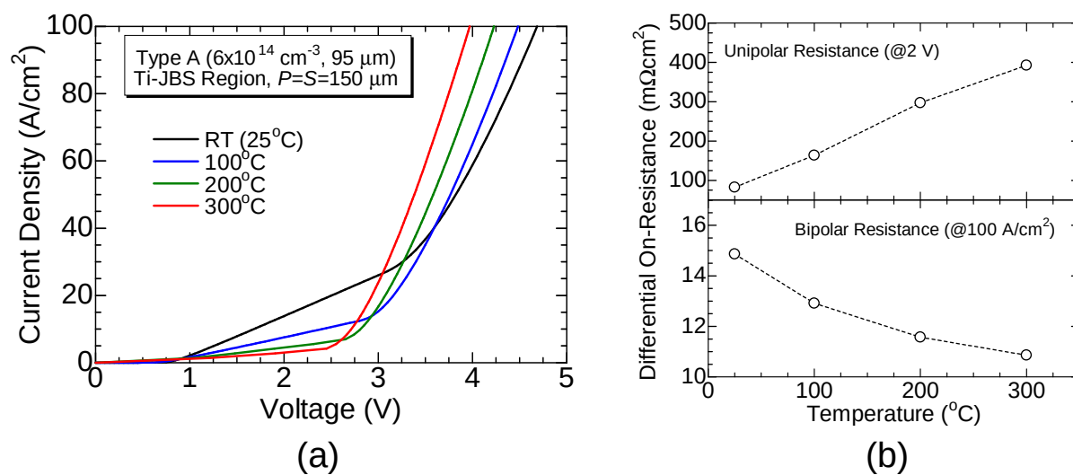
Figure 4.40: (a) Temperature dependence of forward I - V characteristics of an MPS diode with P and S -width of 150\ \mu\text{m} experimentally measured. (b) Temperature dependence of unipolar ( V = 2\ \text{V} ) and bipolar ( J = 100\ \text{A}/\text{cm}^2 ) on-resistance.
