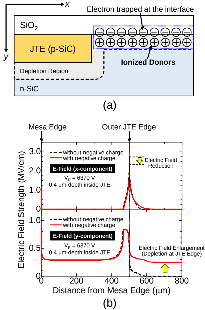
Figure 3.16: (a) Schematic illustration of the effect of negative charge near the \text{SiO}_2/\text{n-SiC} interface. (b) Simulated electric field distribution at 0.4\text{-}\mu\text{m} -depth inside the JTE for single-zone JTE with and without the negative charge near \text{SiO}_2/\text{n-SiC} interface. The reverse bias voltage is 6370\text{ V} , which is the breakdown voltage for a single-zone JTE without negative charge. Here, x - and y - direction are shown in (a).
