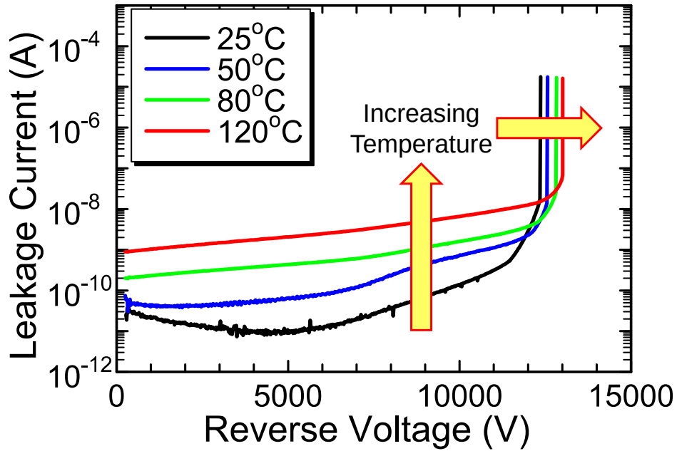
Figure 3.13: Reverse I - V characteristics of a PiN diode with two-zone JTE + SM2 ( D_{\text{JTE1}} = 1.2 \times 10^{13} \text{ cm}^{-2} ) at room temperature (25°C), 50°C, 80°C, and 120°C.
