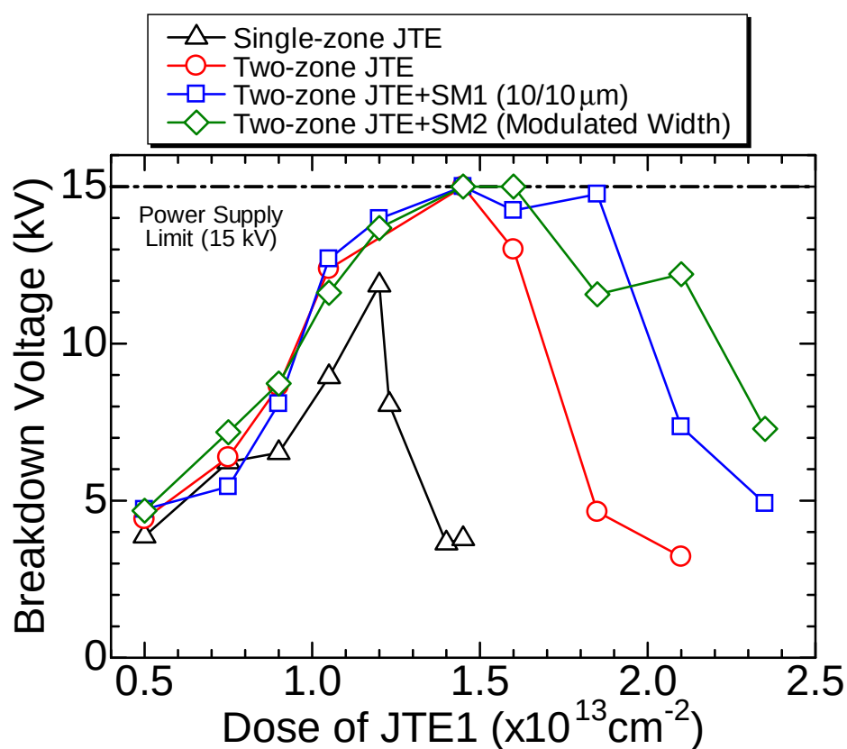
Figure 3.11: Experimental breakdown voltage vs. JTE dose for SiC PiN diodes with single-zone JTE ( \Delta ), two-zone JTE ( \bigcirc ), and SM-JTE combined to two-zone JTE ( \square, \diamond ).
