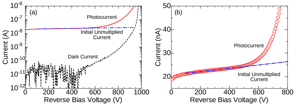
Figure 2.26: Reverse I - V characteristics of PT1 at RT. Here, a BPF of 254 nm was used for the measurement of photocurrent. The initial unmultiplied current was obtained by a linear extrapolation.
