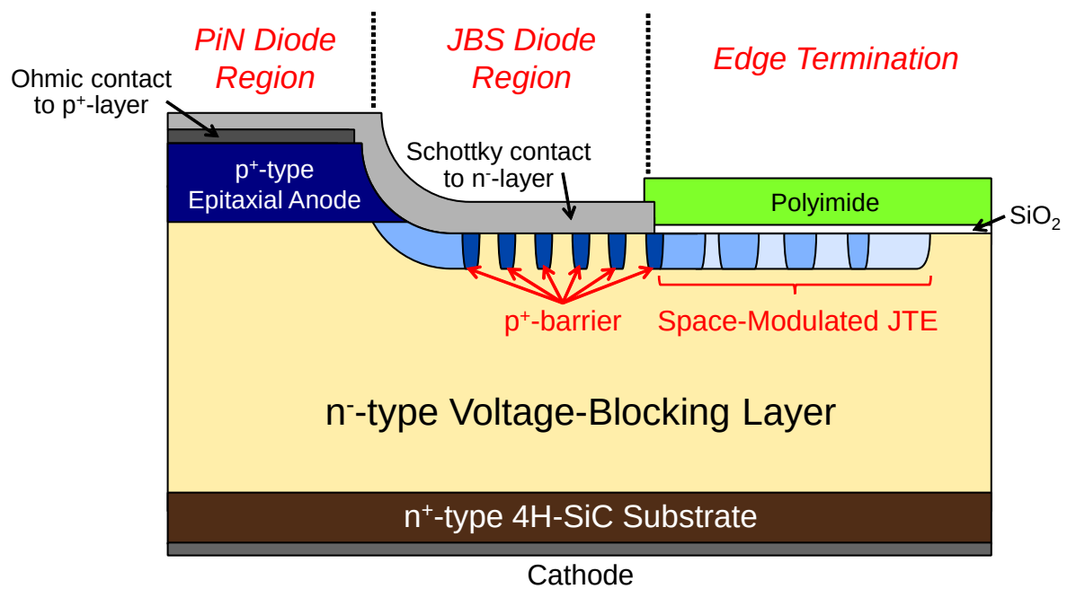
Figure 4.2: Schematic cross section of the mesa-type MPS diode using an epitaxial p + -anode and JBS structure.
