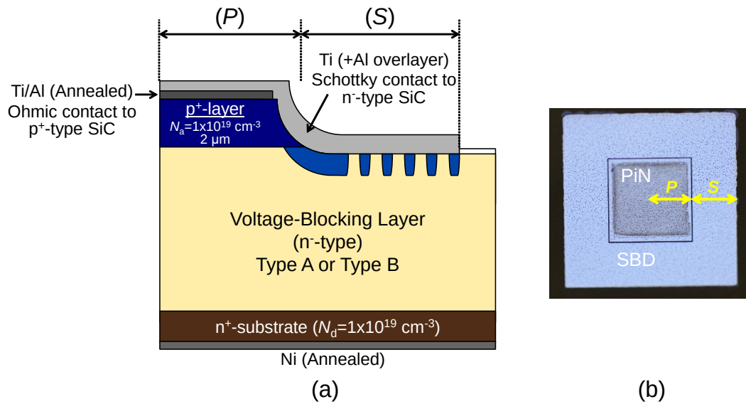
Figure 4.24: (a) Schematic structure of the fabricated MPS diode for analysis of forward characteristics. (b) Optical picture of a fabricated MPS diode.
