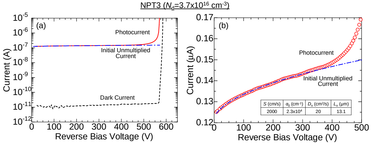
Figure 2.18: Reverse I - V characteristics of NPT3 at RT. Here, a BPF of 260 nm was used for the measurement of photocurrent. The initial unmultiplied current was obtained using equation (2.16).
