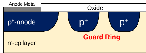
(b) Guard Ring Structure
