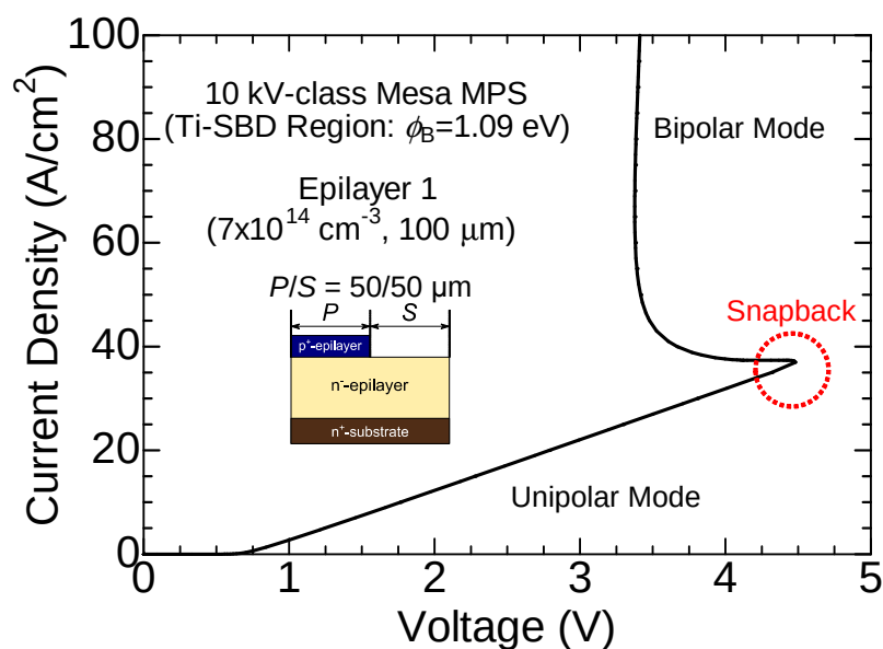
Figure 4.16: Simulated forward I - V characteristics of an unoptimized mesa-type MPS diode.
