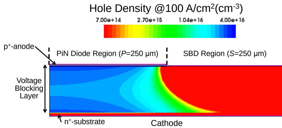
Figure 4.43: Simulated hole density at 100 A/cm 2 for an MPS diode with P and S -width of 250 μm.
