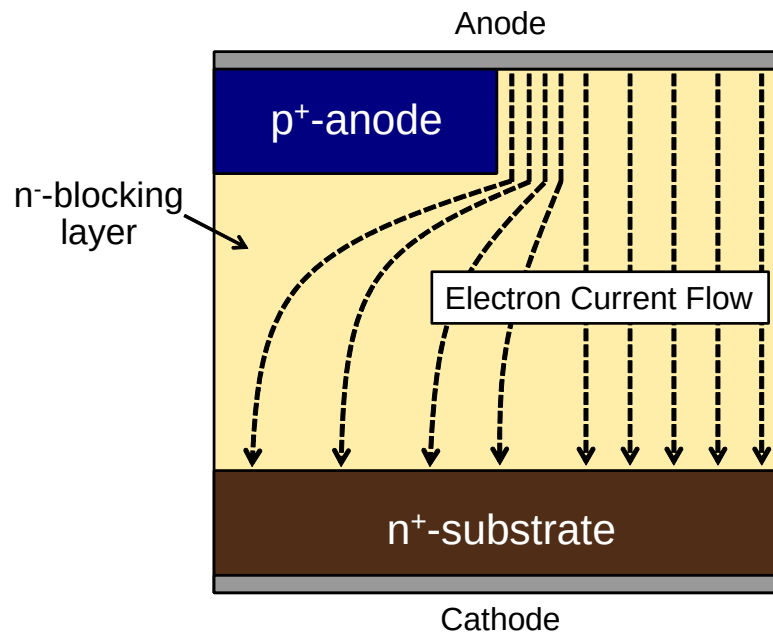
Figure 4.17: Schematic figure of an electron current flow in the unipolar operation mode for a planar MPS diode.
