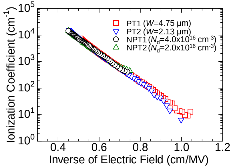
Figure 2.28: Extracted hole ionization coefficient \beta at RT from PT1–2 and NPT1–2.
