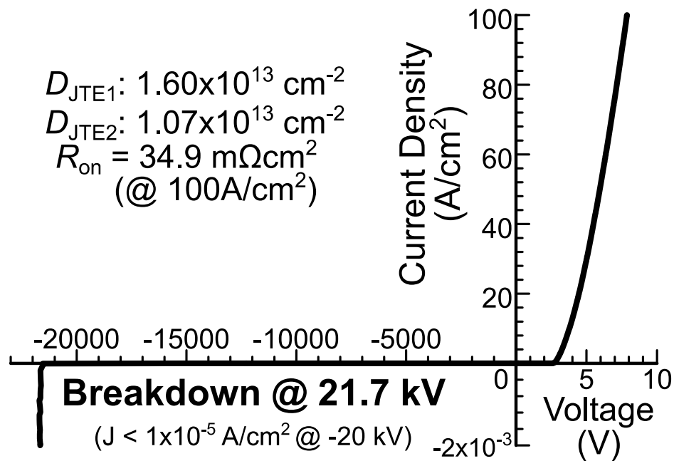
Figure 3.23: I - V characteristics of a fabricated 21.7 kV SiC PiN diode.
