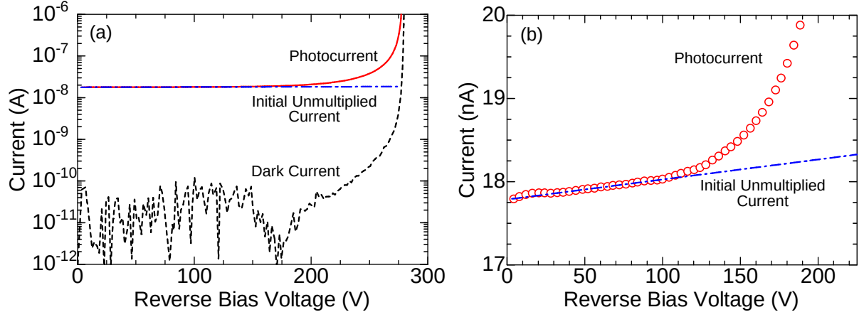
Figure 2.21: Reverse I - V characteristics of NPT4 at RT. Here, a BPF of 260 nm was used for the measurement of photocurrent. The initial unmultiplied current was obtained by a linear extrapolation.
