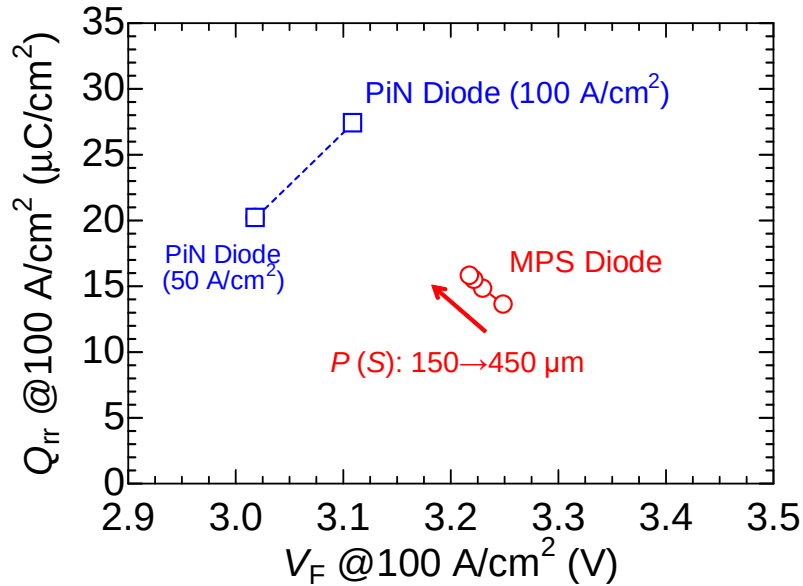
Figure 4.45: Relationship of reverse recovery charge ( Q_{rr} ) and forward voltage drop at 100 \text{ A/cm}^2 ( V_F ) simulated for 10 kV-class SiC MPS and PiN diodes (Epilayer 1).
