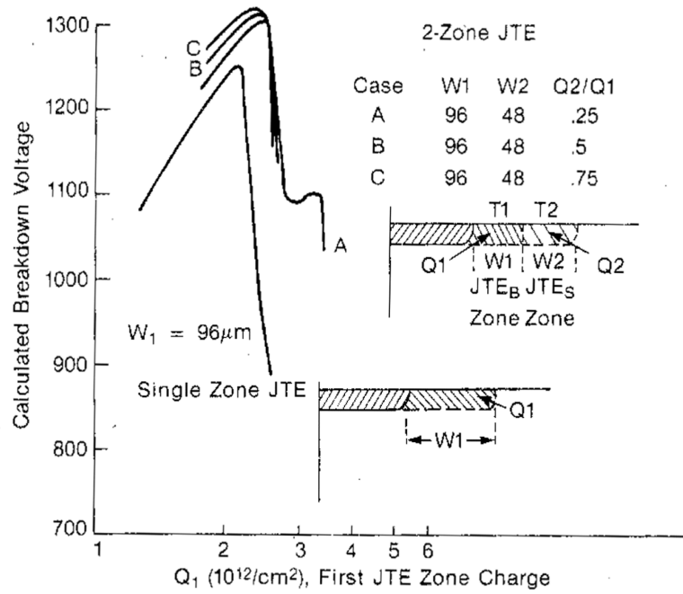
Figure 3.2: Simulated JTE-dose dependence of breakdown voltage for a single-zone and two-zone JTE summarized from [19].
