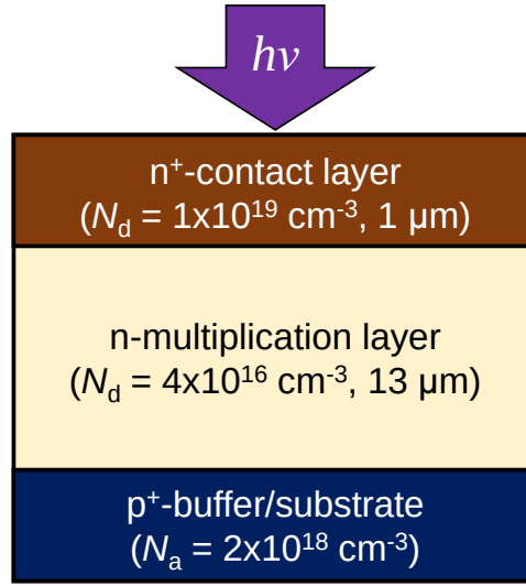
Figure 2.3: Schematic structure of the one-dimensional model assumed here for the simulation of photocurrent component by the change of illumination wavelength.
