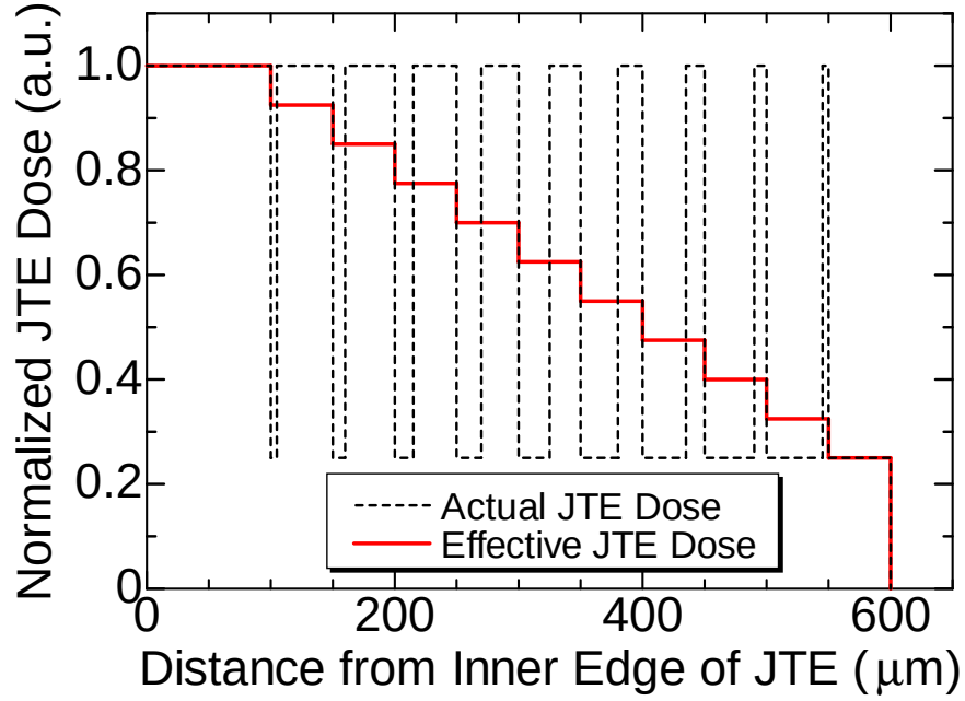
Figure 3.26: Effective JTE-dose distribution inside the improved SM-JTE together with the actual JTE dose distribution.
