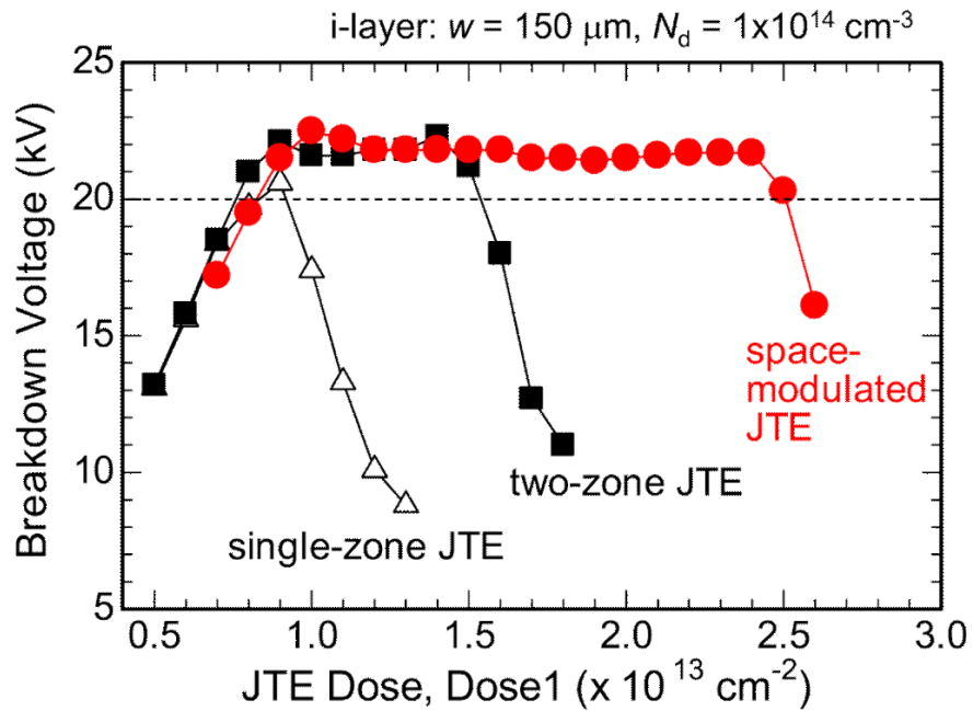
Figure 3.27: JTE1-dose dependence of breakdown voltage for SiC PiN diode with single-zone JTE, two-zone JTE, and the improved SM-JTE. Doping concentration and thickness of the voltage blocking layer assumed here was 1 \times 10^{14} \text{ cm}^{-3} , 150 \text{ } \mu\text{m} .
