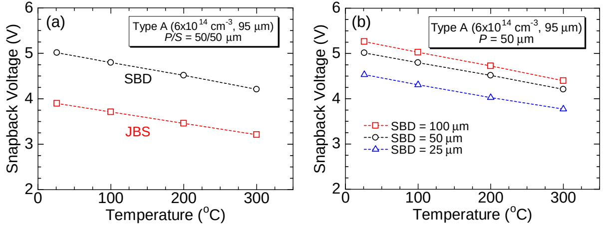
Figure 4.30: Temperature dependence of V_{\text{snap}} experimentally obtained. (a) MPS diodes with SBD or JBS region. (b) MPS diodes with different S -width at given P -width of 50 \mu\text{m} .
