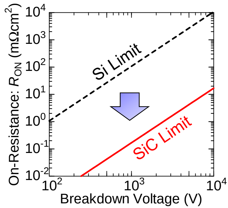
Figure 1.2: Relationship between on-resistance and breakdown voltage for Si and SiC unipolar devices.
