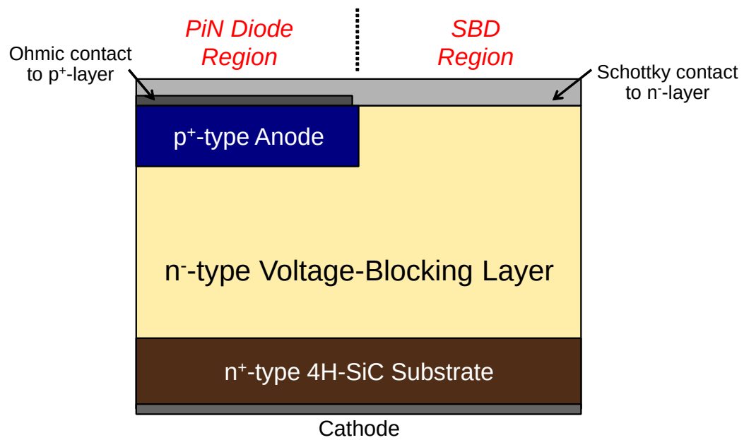
Figure 4.1: Schematic cross section of a planar MPS diode.
