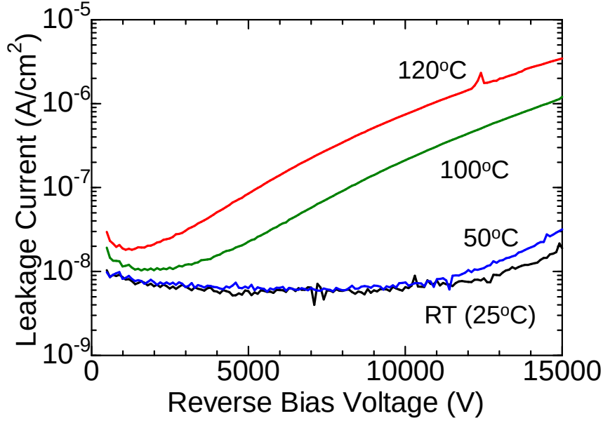
Figure 3.24: Temperature dependence of leakage current for a 20 kV-class PiN diode. A clear positive temperature coefficient of leakage current is observed.
