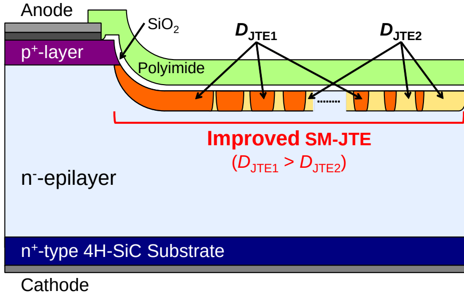
Figure 3.25: Improved SM-JTE structure proposed in this study where a VLD (Variation of Lateral Doping)-like dopant profile was realized in horizontal direction.
