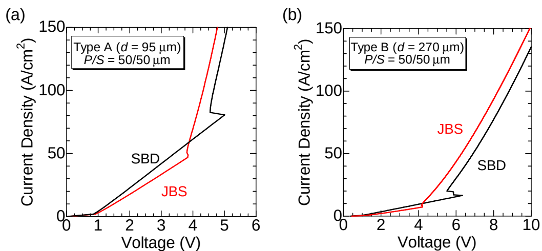
Figure 4.29: Forward I - V characteristics of MPS diodes with (JBS) and without (SBD) p^+ -barriers for P -width of 50 \mu\text{m} .
