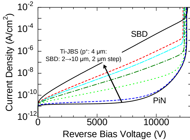
Figure 4.7: SBD-region width dependence of reverse I - V characteristics while assuming a constant p^+ -region width of 4 \mu\text{m} .
