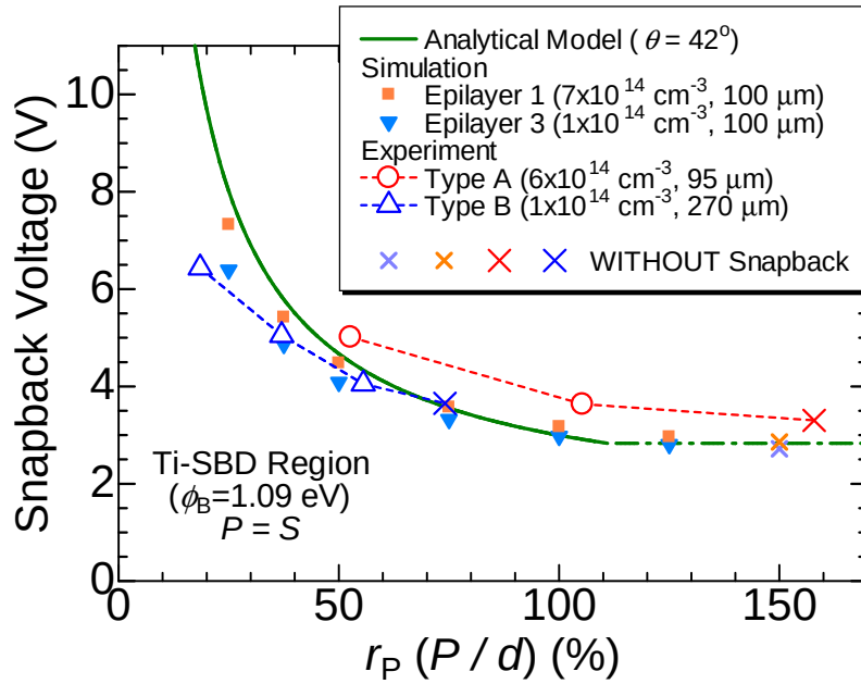
Figure 4.31: r_P dependence of V_{\text{snap}} for the analytical model (solid line), device simulation (closed symbols), and experiment (open symbols).
