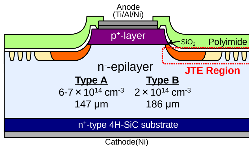
Figure 3.5: Schematic structure of a fabricated SiC PiN diode. Type A epilayer was used to fabricate 10 kV-class diodes, and type B epilayer was used to fabricate 20 kV-class diodes.
