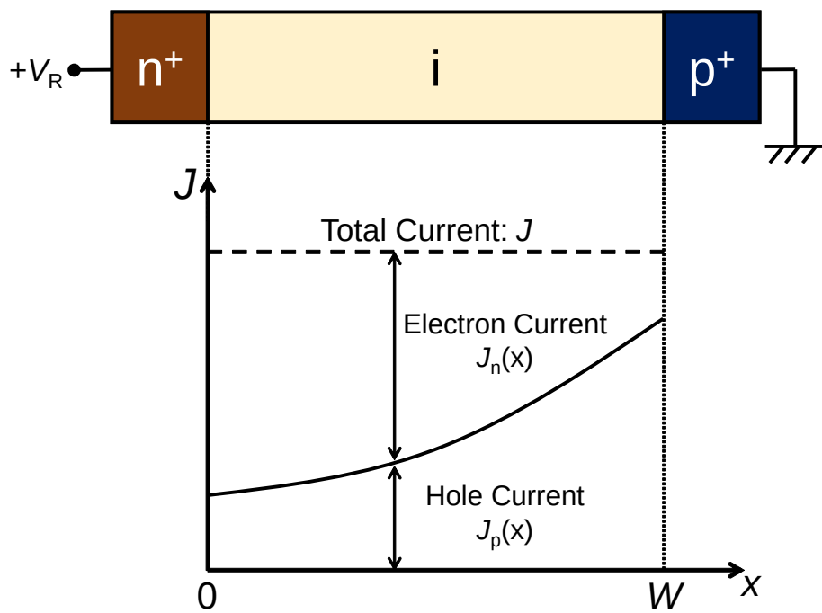
Figure 2.2: Schematic illustration of the quantities of hole and electron currents inside the depletion layer.
