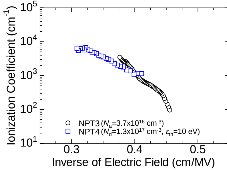
Figure 2.25: Extracted electron ionization coefficient \alpha at room temperature from NPT3 and NPT4. For NPT4, \varepsilon_{th} = 10 eV was used for the dead space correction.
