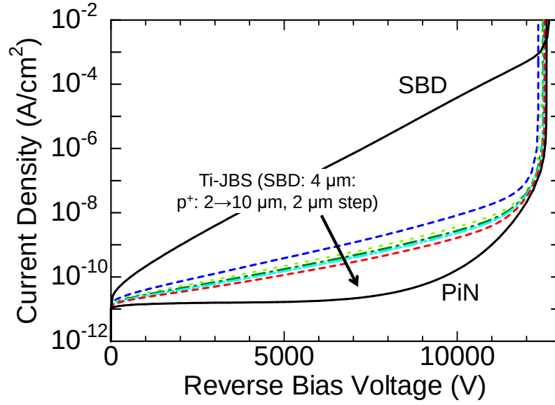
Figure 4.6: p^+ -region width dependence of reverse I - V characteristics while assuming a constant SBD region width of 4 \mu\text{m} .
