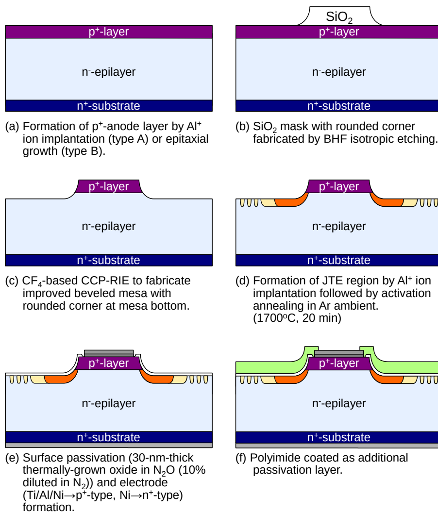
Figure 3.6: Schematic illustrations of the fabrication process of SiC PiN diodes.
