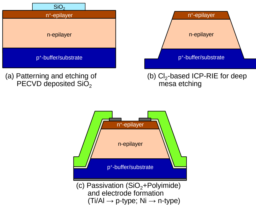
Figure 2.9: Schematic figure of the fabrication process of NPT1, NPT2, and NPT3.
