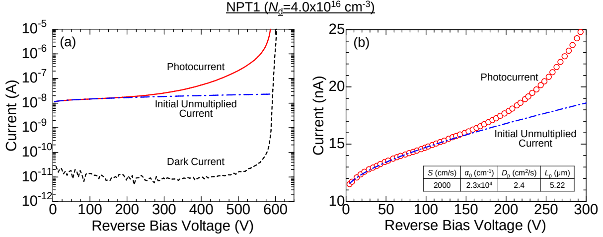
Figure 2.17: Reverse I - V characteristics of NPT1 at RT. Here, a BPF of 260 nm was used for the measurement of photocurrent. The initial unmultiplied current was obtained using equation (2.16).
