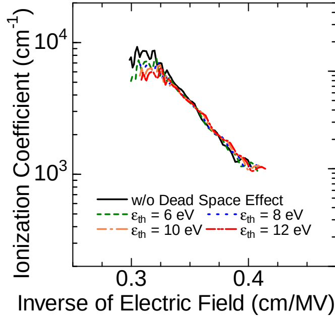
Figure 2.24: Extracted electron ionization coefficient \alpha from NPT4, where M_{ni} calculated at various values of \epsilon_{th} was used.
