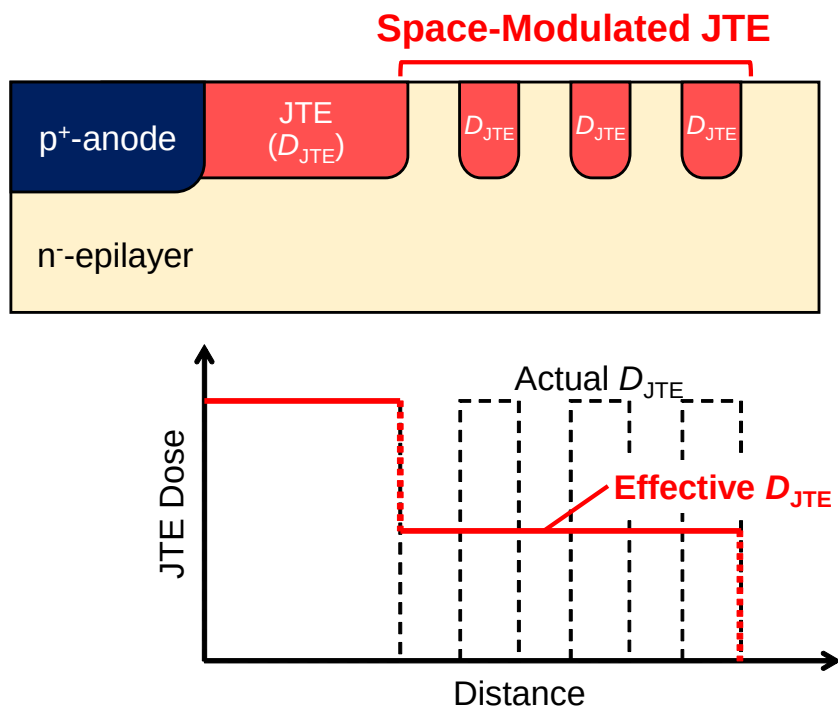
Figure 3.3: Schematic illustration of space-modulated JTE combined with single-zone JTE, together with the concept of “ effective ” JTE dose.
