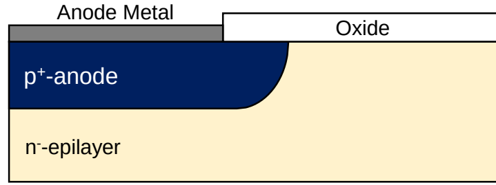
Figure 1.8: Schematic cross section near the edge of p^+n region in a real planar PiN diode structure.
