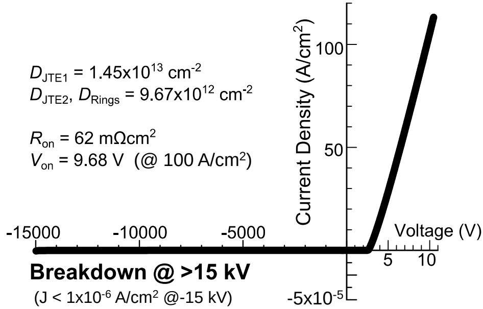
Figure 3.12: I - V characteristics of a 15 kV-class SiC PiN diode with two-zone JTE and SM-JTE [Fig. 3.8 (c)].
