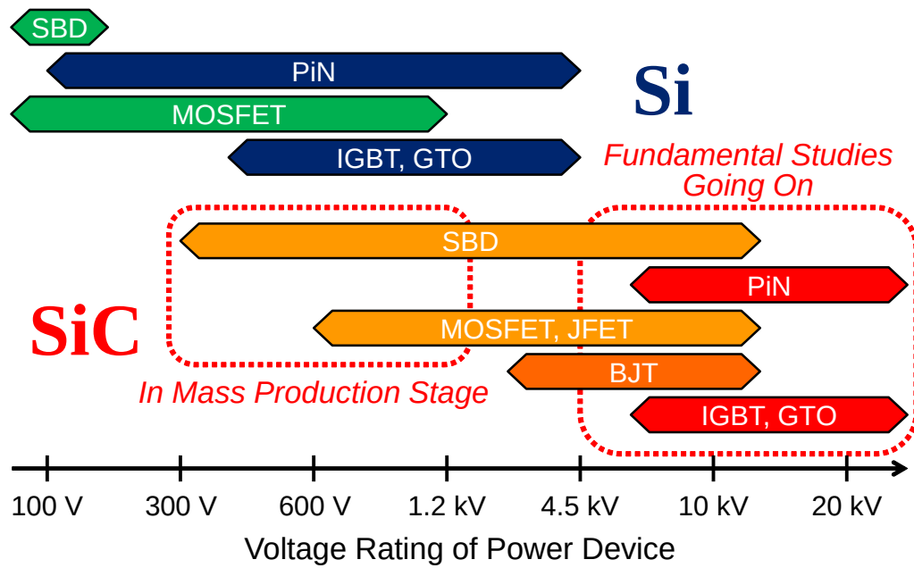
Figure 1.3: Voltage rating of Si and SiC power devices.
