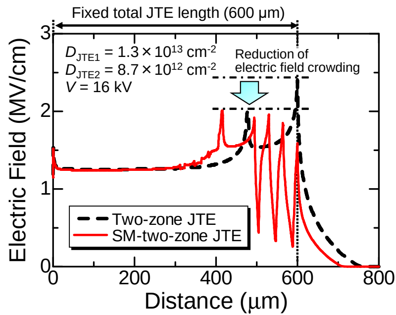
Figure 3.20: Electric field profile inside the JTE at 0.8- \mu\text{m} -depth for two-zone JTE and SM-two-zone JTE at a reverse bias voltage of 16 kV, which is the breakdown voltage for two-zone JTE.
