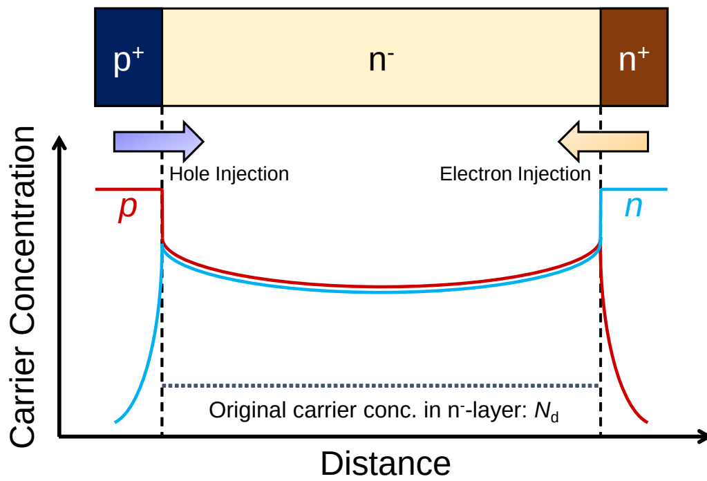
Figure 1.5: Schematic illustration of conductivity modulation effect in a PiN diode.
