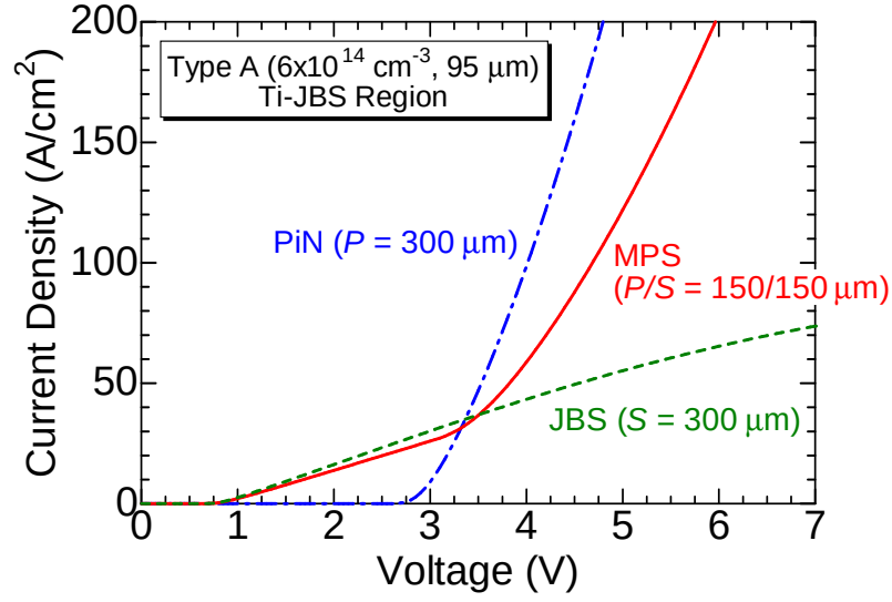
Figure 4.35: Measured forward I - V characteristics of an MPS diode with P = S = 150 \mu\text{m} . In the same figure, measurement results of PiN diode and JBS diode with the same area are also shown.
