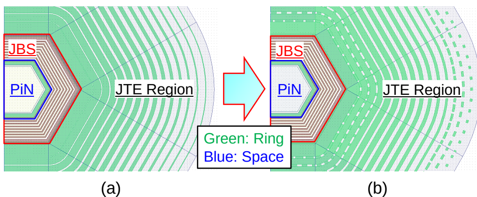
Figure 4.12: Mask layout design for (a) conventional SM-JTE used in Chapter 3 and (b) improved SM-JTE with two-dimensionally modulated structure.
