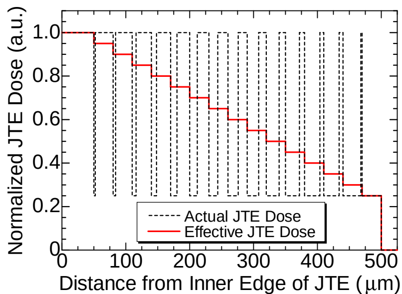
Figure 4.10: Lateral distribution of actual and effective JTE dose inside the SM-JTE.
