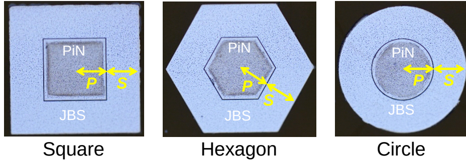
Figure 4.38: Optical picture of different anode geometries measured in this study. These MPS diodes have P - and S -widths of 150\ \mu\text{m} .
