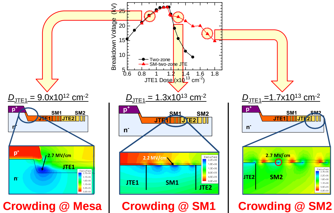
Figure 3.19: Electric field distribution in the region of electric field crowding occurring for various JTE doses at breakdown voltage.
