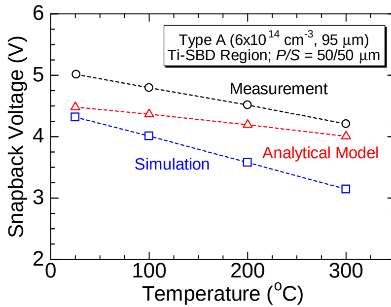
Figure 4.34: Temperature dependence of V_{\text{snap}} for the analytical model, device simulation, and experiment.
