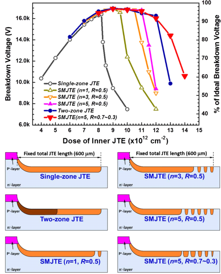
Figure 3.4: JTE-dose dependence of the simulated breakdown voltage for SiC PiN diodes with various JTE structures taken from [15]. The thickness and doping concentration of n^- -epilayer used are 120 \mu\text{m} and 1 \times 10^{14} \text{ cm}^{-3} , respectively. Schematic illustration of each JTE structure is shown at the bottom.
