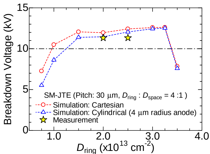
Figure 4.48: D_{\text{ring}} dependence of breakdown voltage by simulation and experiment.
