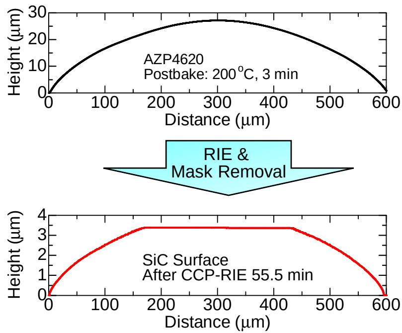
Figure 2.15: Surface profile of lens-like photoresist mask and the transferred small-beveled mesa of SiC.
