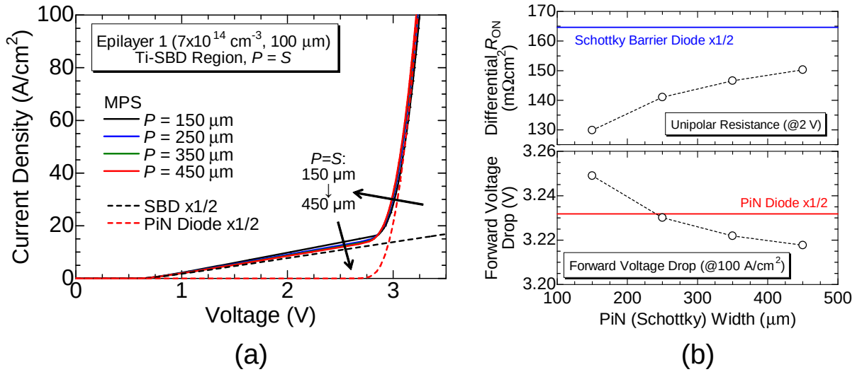
Figure 4.42: (a) Simulated forward I - V characteristics of MPS diodes (Epilayer 1) with P -width larger than 150 \mu\text{m} . (b) P -width dependence of unipolar on-resistance ( V = 2 \text{ V} ) and forward voltage drop at J = 100 \text{ A/cm}^2 .
