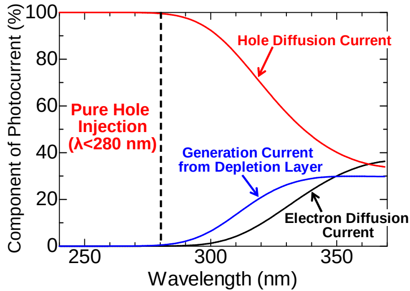
Figure 2.4: Simulated percentages of photocurrent components at different illumination wavelength.
