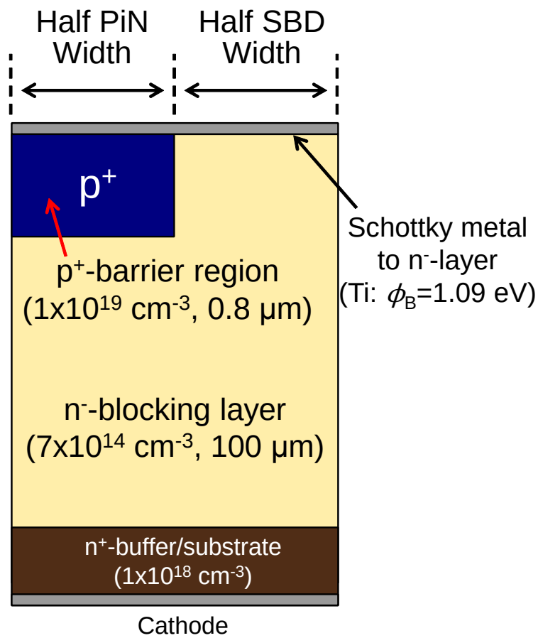
Figure 4.5: Schematic cross section of a planar JBS diode for the simulation of anode layout design.
