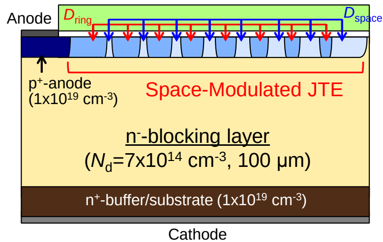
Figure 4.9: Schematic structure of a planar PiN diode with SM-JTE assumed for the simulation of breakdown voltage.
