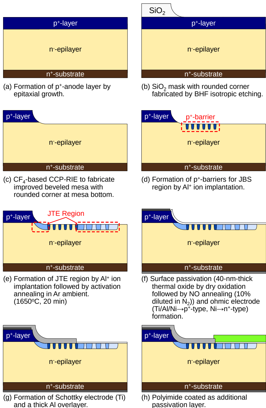
Figure 4.15: Schematic illustrations of the fabrication process of SiC MPS diodes.
