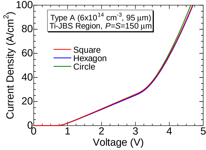
Figure 4.37: Measured forward I - V characteristics of MPS diodes with different anode geometries. Here, P and S -widths were kept to 150\ \mu\text{m} .
