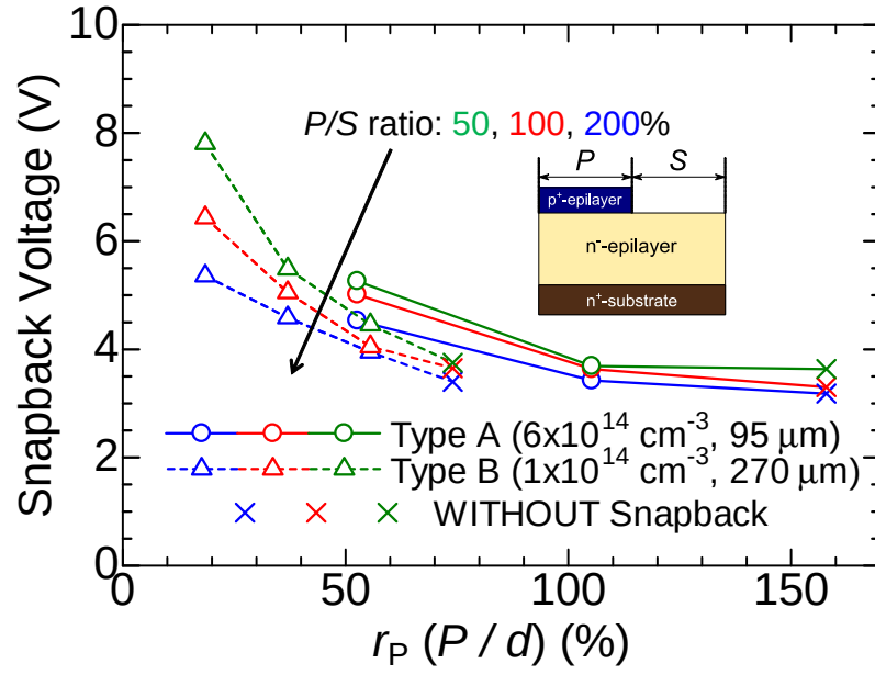
Figure 4.26: Experimentally obtained r_P dependence of V_{snap} for MPS diodes with different P/S ratios.
