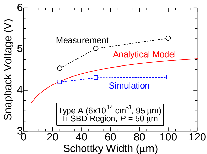
Figure 4.33: S -width dependence of V_{\text{snap}} for the analytical model, device simulation, and experiment.
