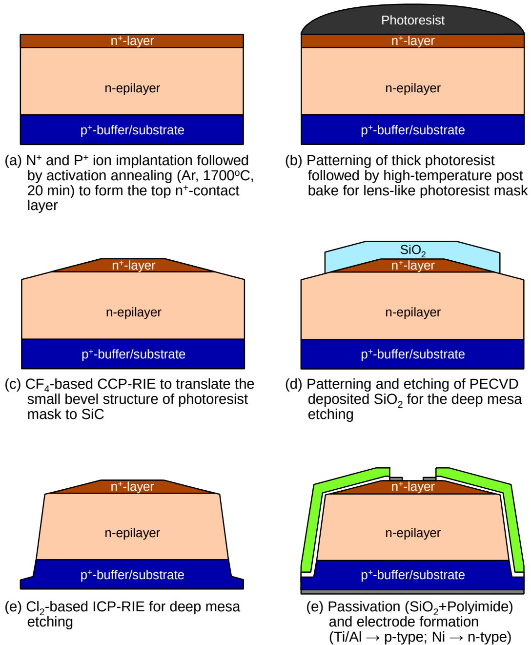
Figure 2.14: Schematic figure of the fabrication process of PT1 and PT2.
