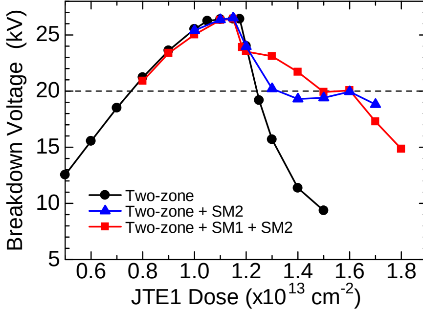
Figure 3.18: Simulated JTE1-dose dependence of breakdown voltage for PiN diode for two-zone JTE, two-zone JTE combined with SM2, and two-zone JTE combined with SM1 and SM2 (SM-two-zone JTE).
