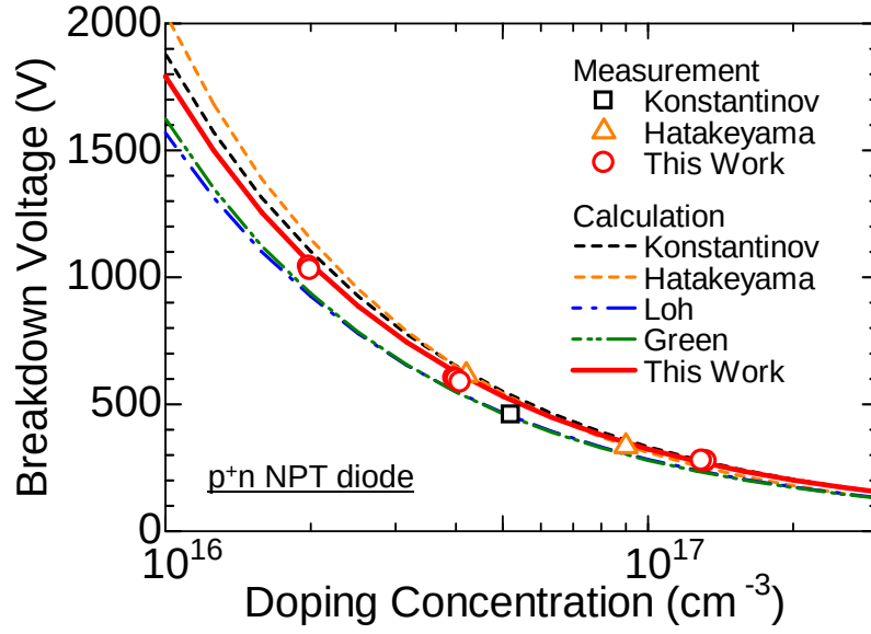
Figure 2.30: Simulated doping concentration dependence of ideal breakdown voltage and experimental results for p^+n NPT diodes. Calculation was done using ionization coefficients obtained from [1, 5, 7, 8] and values obtained in this study.
