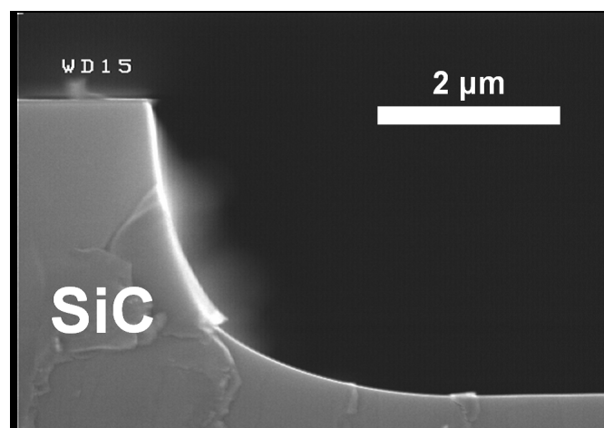
Figure 3.7: SEM image of the improved beveled mesa used in this study.
