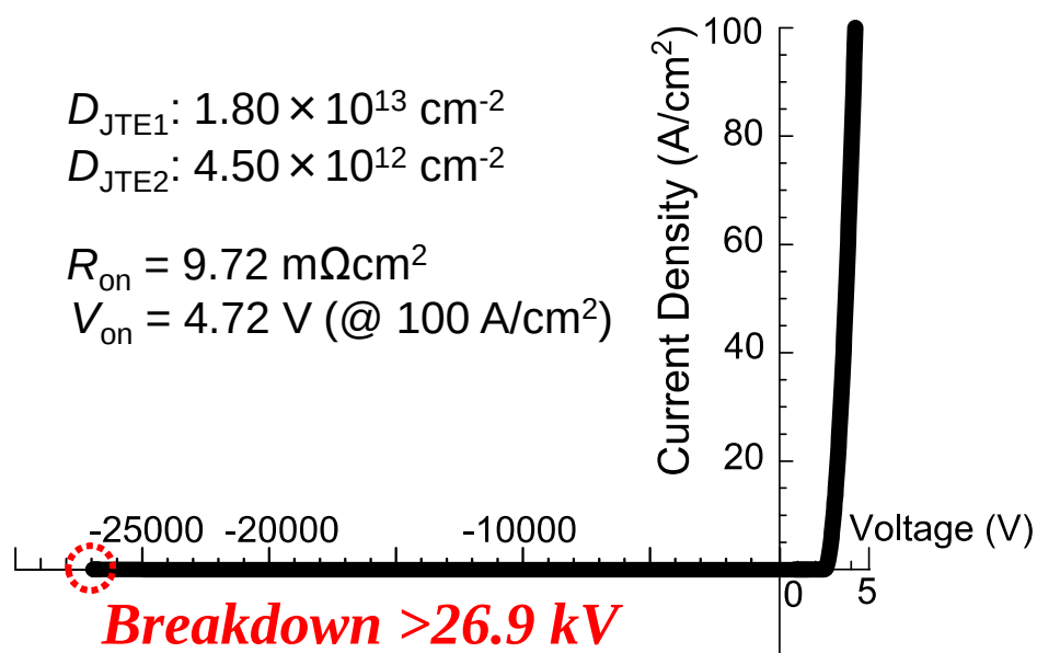
Figure 3.28: I - V characteristics of an UHV SiC PiN diode with voltage blocking layer thickness of 268 \mu\text{m} . Using the improved SM-JTE, breakdown voltage over 26.9 \text{ kV} was achieved.
