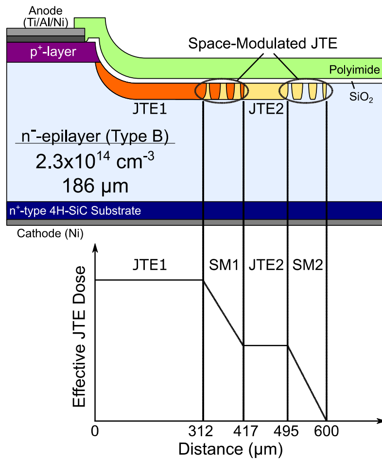
Figure 3.17: Schematic illustration of a fabricated SiC PiN diode with space-modulated two-zone JTE and its effective JTE-dose distribution.
