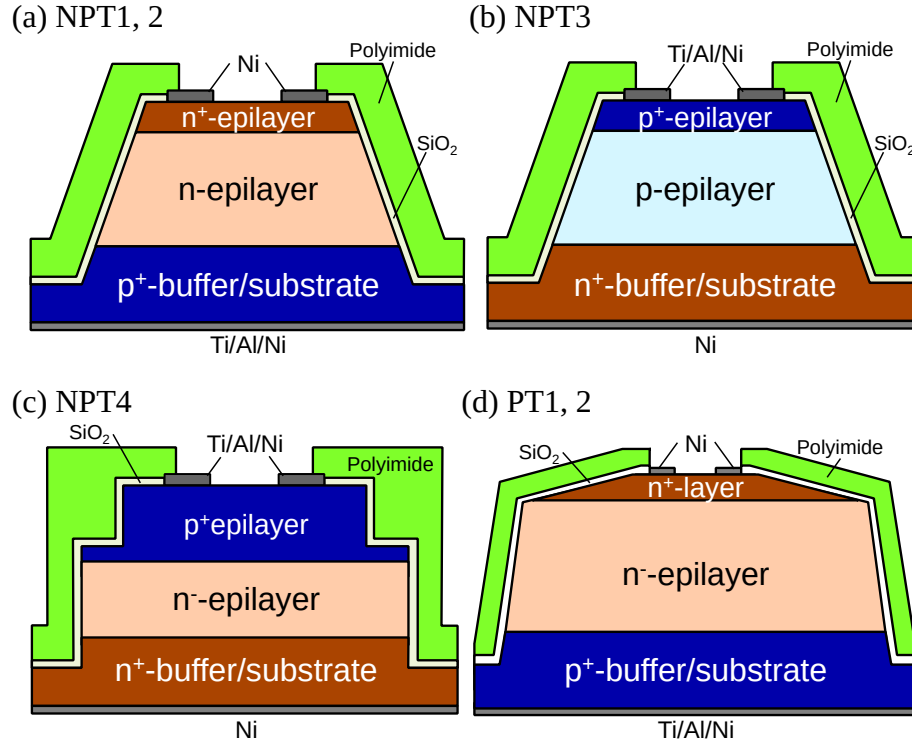
Figure 2.6: Schematic cross section of the fabricated PDs. Structures of the individual layers are summarized in Table 2.1.
