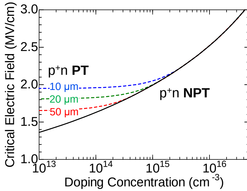
Figure 2.38: Doping concentration dependence of critical electric field for p + n NPT structure and PT structure with various blocking layer thickness.
