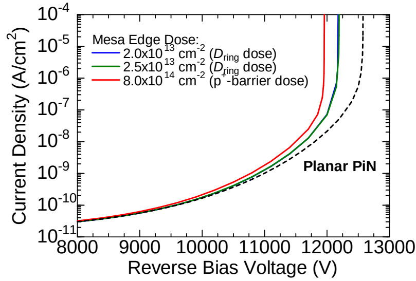
Figure 4.14: Reverse I - V characteristics of mesa structure with various implanted mesa dose.
