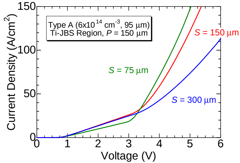
Figure 4.36: Measured forward I - V characteristics of MPS diodes with different S -widths while keeping P -width to 150 \mu\text{m} .
