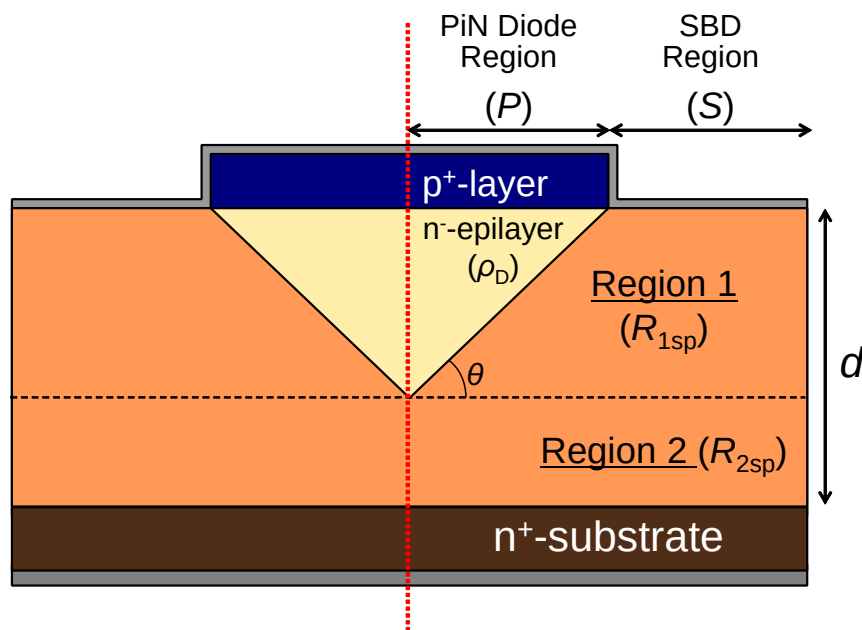
Figure 4.18: Schematic illustration of the approximated electron current flow in the JBS current-distribution model.
