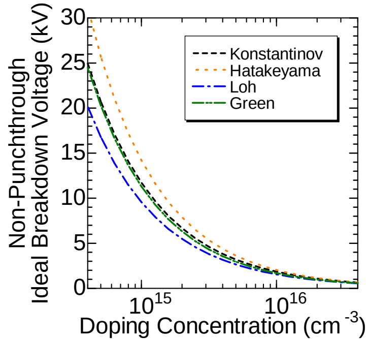
Figure 1.7: Doping concentration dependence of ideal breakdown voltage for non-punchthrough SiC p + n structure, calculated by using impact ionization coefficients from [146, 148–150].
