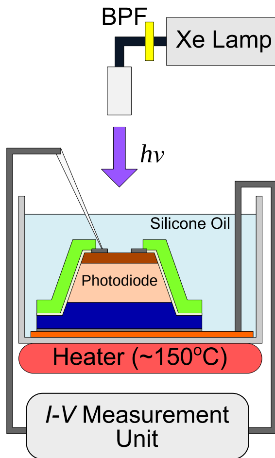
Figure 2.5: Schematic illustration of the measurement setup used for the photomultiplier measurement in this study.
