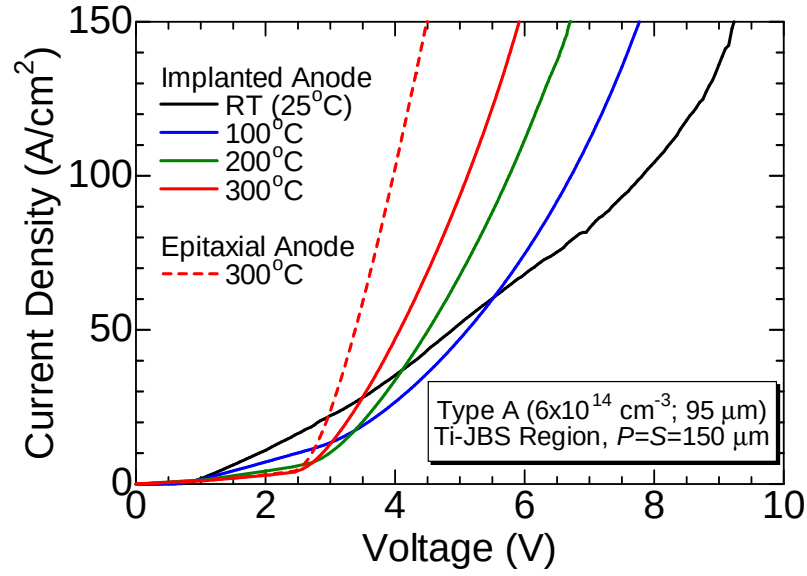
Figure 4.41: Temperature dependence of forward I - V characteristics of MPS diodes with implanted and epitaxial p^+ -anode.
