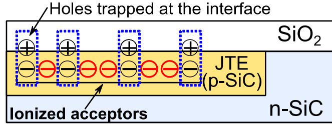
Figure 3.15: Schematic illustration of the effect of positive charge near the \text{SiO}_2/\text{p-SiC} interface.
