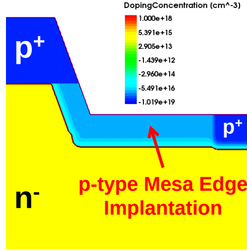
Figure 4.13: The simulated structure of a mesa MPS diode to investigate the influence of mesa structure to the breakdown voltage.
