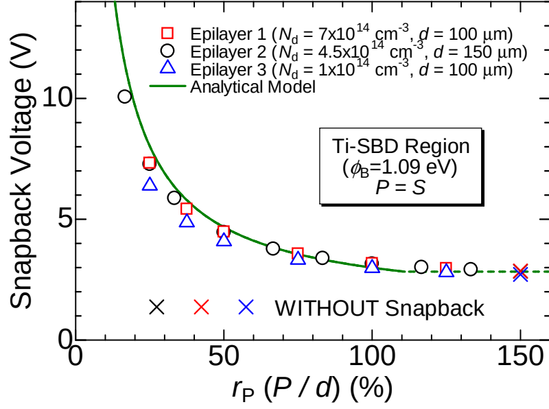
Figure 4.22: Simulated and analytical r_P dependence of V_{\text{snap}} . Analytical results best fits the simulation at a current spreading angle \theta of 42^\circ .
