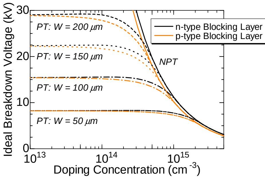
Figure 2.40: Doping concentration dependence of ideal breakdown voltage for PT structure with different blocking layer thickness for n-type and p-type blocking layer.
