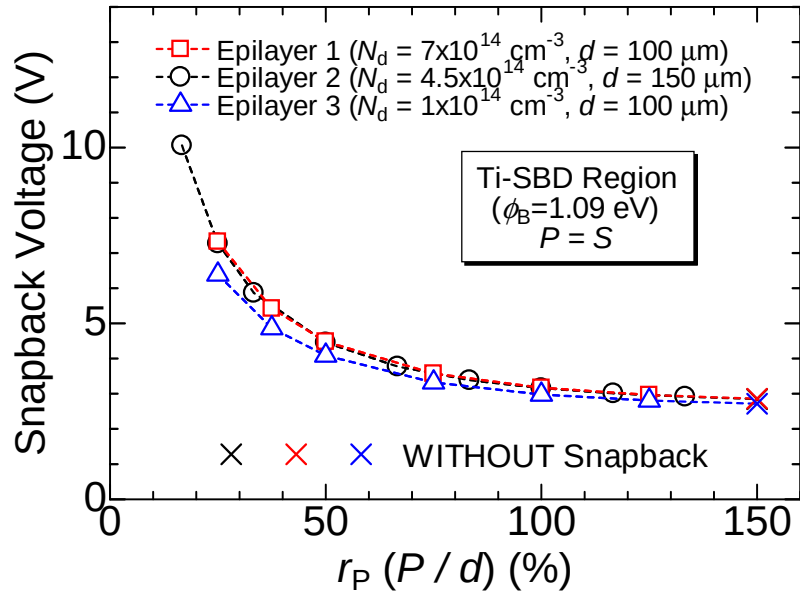
Figure 4.21: Simulated r_P ( P/d ) dependence of snapback voltage ( V_{\text{snap}} ) for MPS diodes with different voltage-blocking layer structures.
