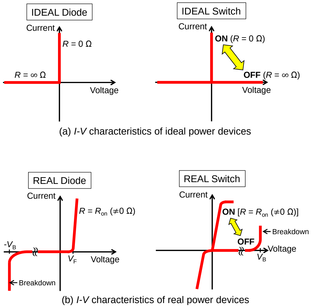
Figure 1.1: Schematic illustration of I - V characteristics of (a) ideal and (b) real diode and switch.
