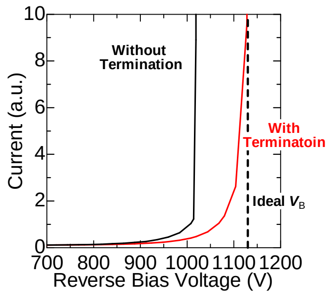
Figure 2.13: Simulated reverse I - V characteristics of PT diode with and without edge termination.
