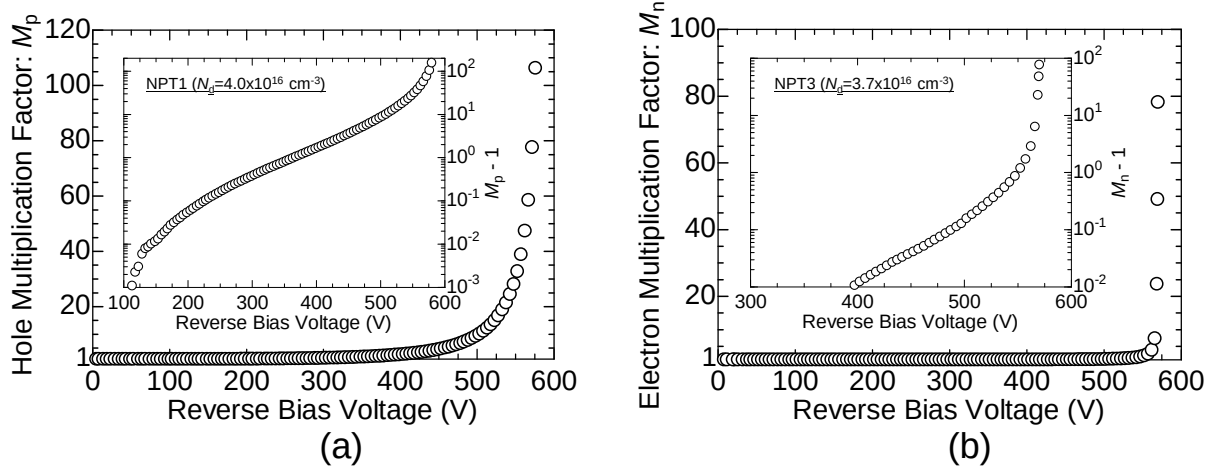
Figure 2.19: Reverse bias voltage dependence of multiplication factors. Inset shows the plot of M - 1 on a logarithmic scale. (a) NPT1: measurement of M_p . (b) NPT3: measurement of M_n .
