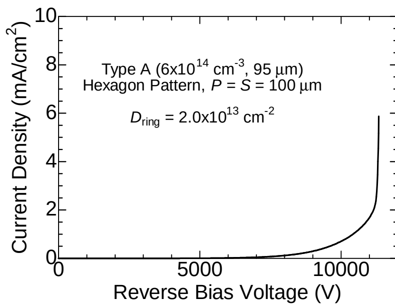
Figure 4.47: Reverse I - V characteristics of MPS diode with improved SM-JTE.
