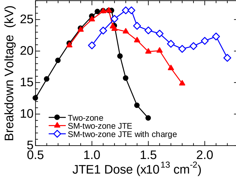
Figure 3.21: JTE1-dose dependence of breakdown voltage for SM-two-zone JTE taking account of the interface charge. Positive charge ( +2 \times 10^{12} \text{ cm}^{-2} ) at the \text{SiO}_2/\text{p-SiC} interface, and/or negative charge ( -1.4 \times 10^{12} \text{ cm}^{-2} ) at the \text{SiO}_2/\text{n-SiC} interface were assumed in the simulation.
