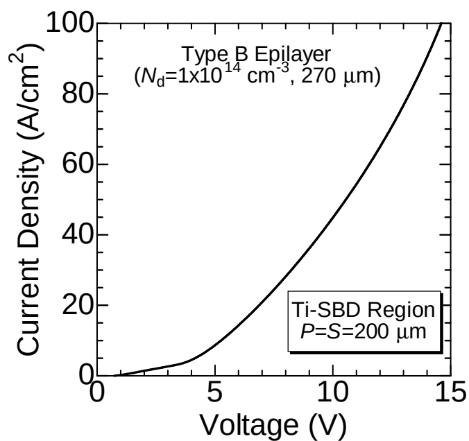
Figure 4.28: Forward I - V characteristics of MPS diode with Type B epilayer for P -width of 200 \mu\text{m} .
