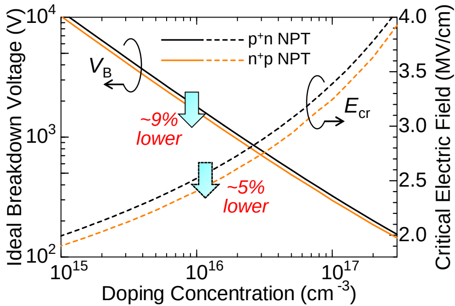
Figure 2.39: Doping concentration dependence of ideal breakdown voltage and critical electric field strength for p^+n (n-type blocking layer) and n^+p (p-type blocking layer) structures.
