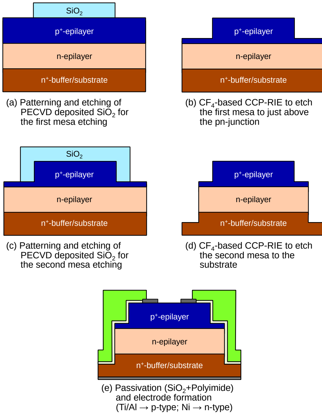
Figure 2.11: Schematic figure of the fabrication process of NPT4.
