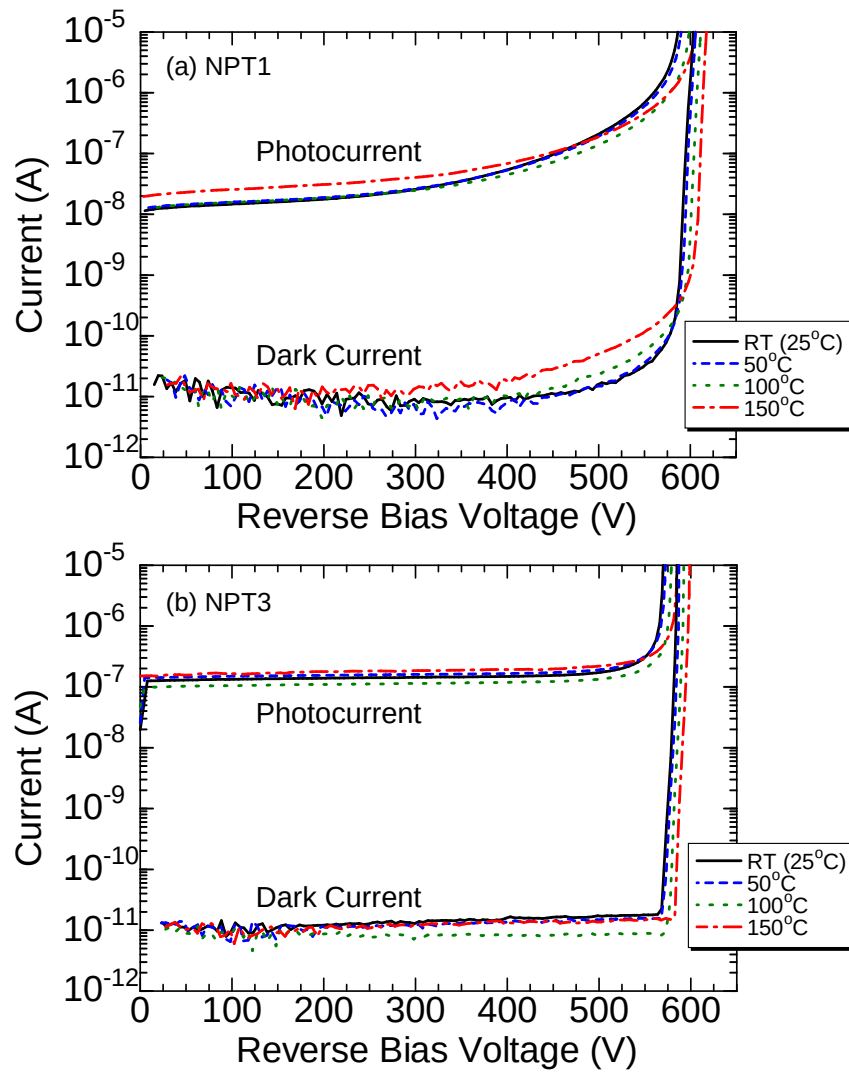
Figure 2.33: Dark and photo-current of (a) NPT1 and (b) NPT3 at room temperature and elevated temperatures up to 150°C.
