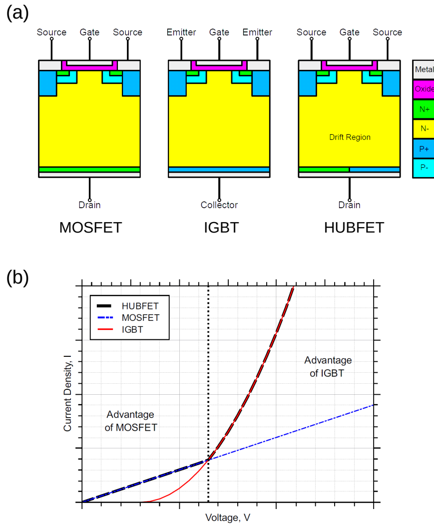
Figure 1.10: (a) Schematic cross section and (b) schematic illustration of forward I - V characteristics of MOSFET, IGBT, and HUBFET taken from [163].
