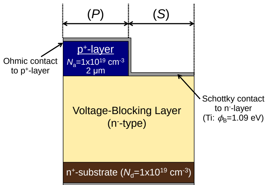
Figure 4.19: Schematic illustration of the mesa type MPS diode assumed in the simulation.
