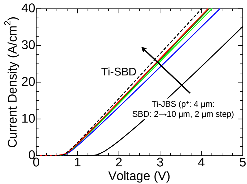
Figure 4.8: SBD-region width dependence of forward I - V characteristics while assuming a constant p^+ -region width of 4 \mu\text{m} .
