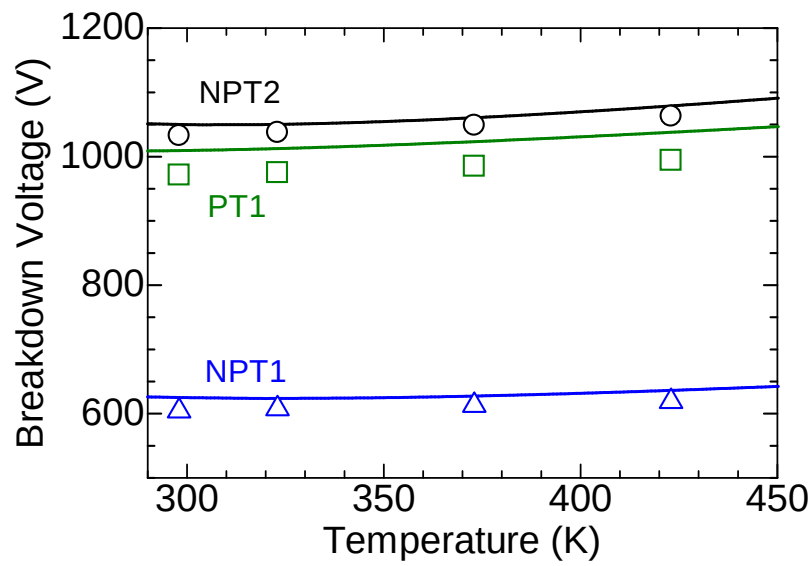
Figure 2.36: Temperature dependence of breakdown voltage for NPT1, NPT2, and PT1. Lines: simulated results using the temperature dependence of ionization coefficients obtained in this study.
