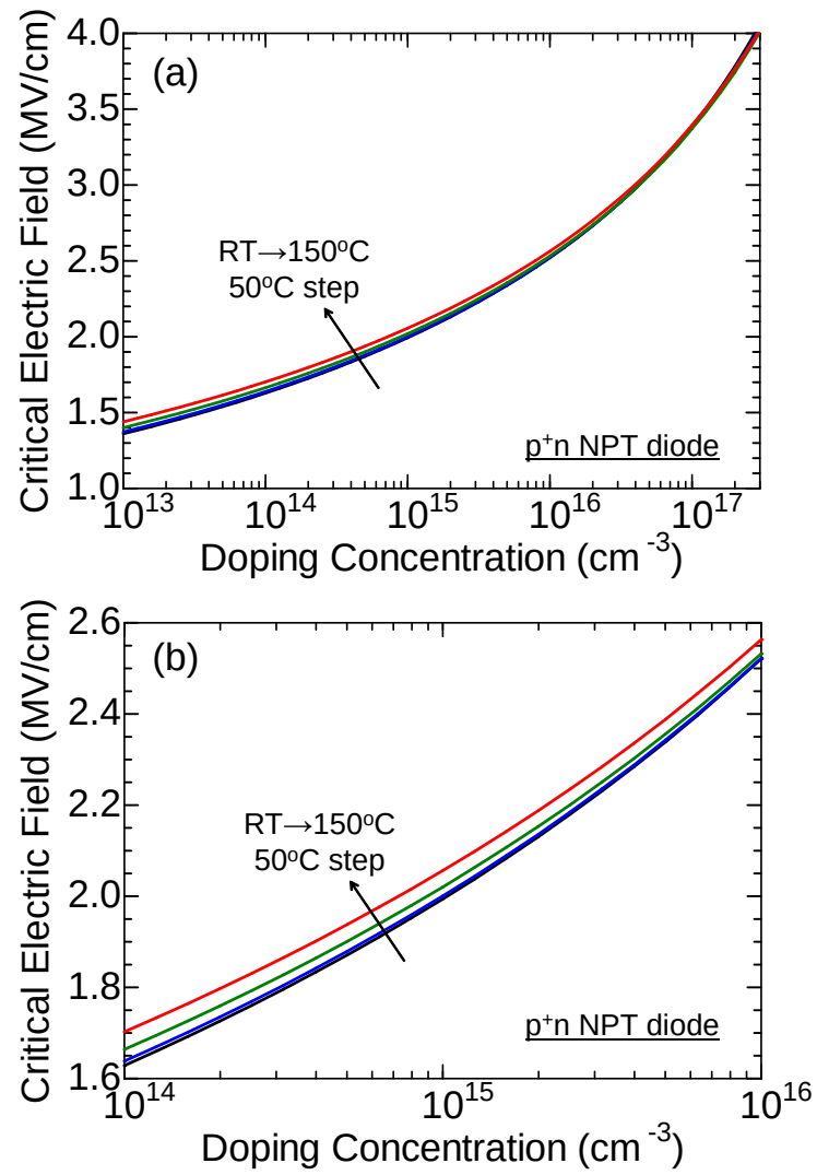
Figure 2.37: (a) Temperature dependence of critical electric field strength calculated for p + n NPT structures. An enlarged figure is shown in (b).
