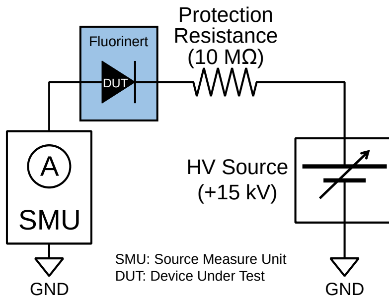
Figure 3.10: Schematic illustration of the custom-made ultrahigh-voltage DC measurement system used in this study.
