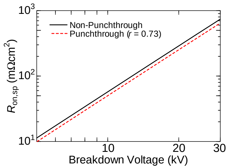
Figure 4.4: R_{ON} – BV relationship for NPT and PT with optimized ratio between PT and NPT thickness.
