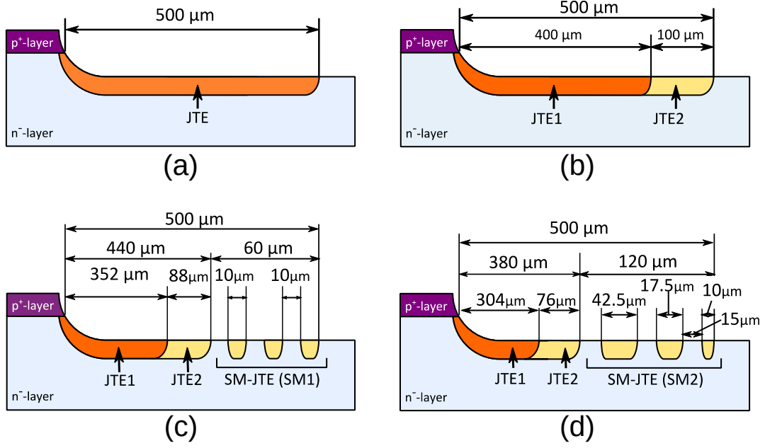
Figure 3.8: JTE structures fabricated in this study. Space-modulated JTEs were combined with the two-zone JTE while fixing the total JTE length to 500 \mu\text{m} , and dose ratio of 3 : 2. (a) Single-zone JTE. (b) Two-zone JTE. (c) Two-zone JTE + SM1. (d) Two-zone JTE + SM2.
