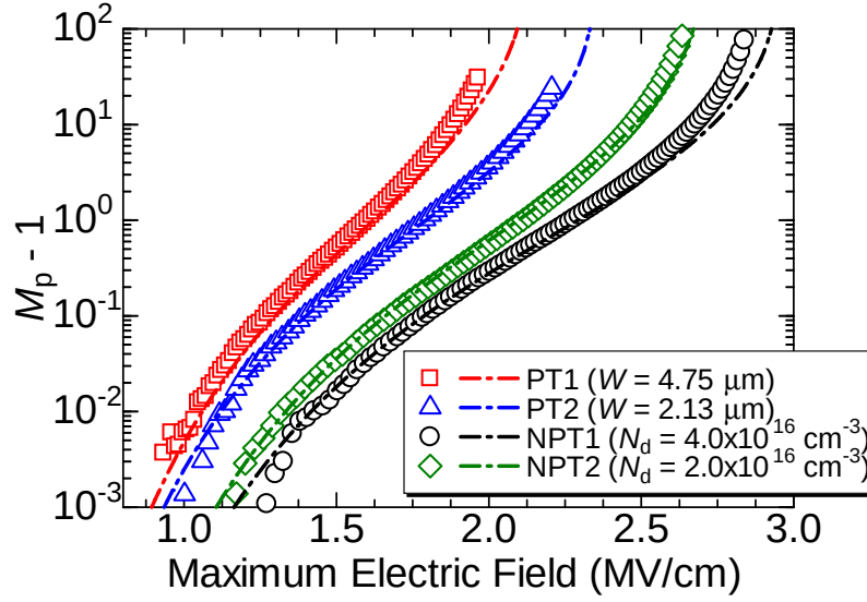
Figure 2.27: Maximum electric field dependence of M_p - 1 obtained from PT1–2 and NPT1–2. Here, symbols show the measurement results, and lines show the simulated M_p - 1 using ionization coefficients obtained in this study.
