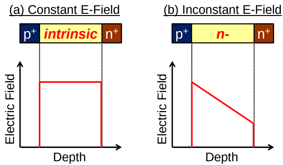
Figure 2.42: Difference of electric field distribution inside the depletion layer for PiN structure with different doping concentration of blocking layer.
