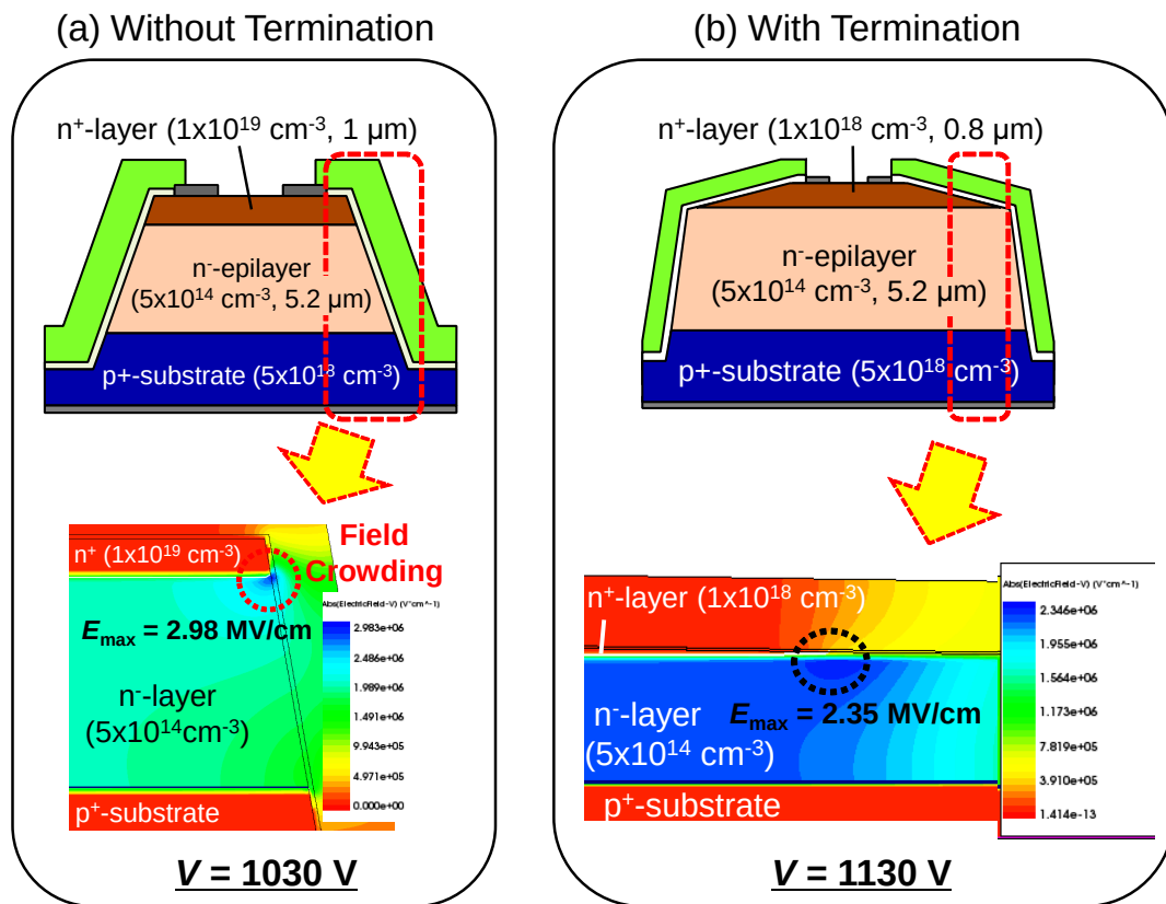
Figure 2.12: Simulated electric field distribution at breakdown voltage for a PT diode (a) without termination and (b) with termination.
