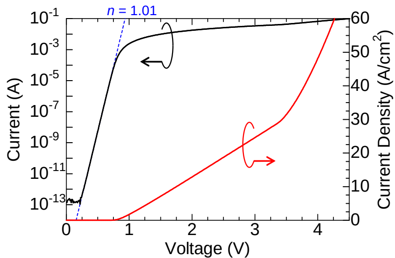
Figure 4.46: Forward I - V characteristics of an MPS diode having JBS region and P -width of 100\ \mu\text{m} .
