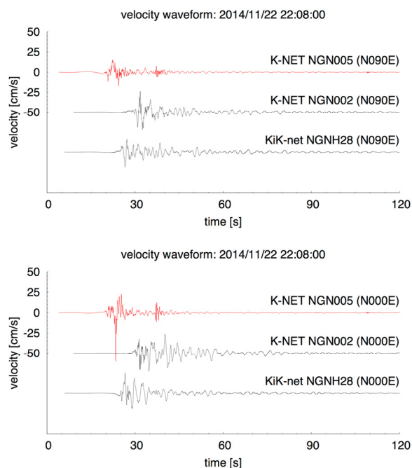
Fig.2 Velocity waveforms observed at K-NET NGN005, NGN002, and NGNH28.
