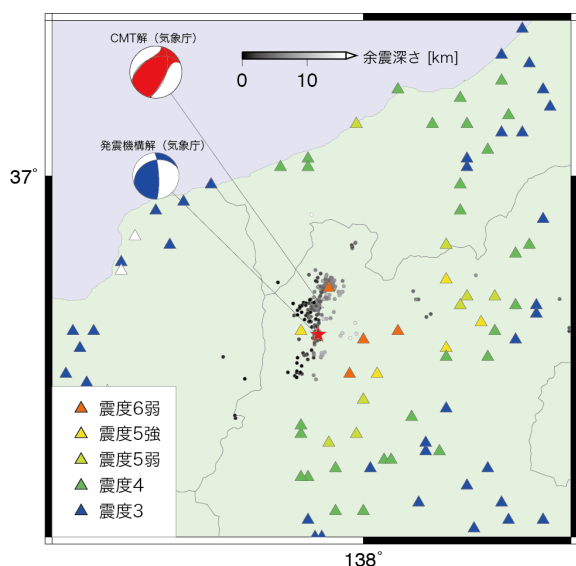
Fig.1 Hypocenter and aftershock distribution during the 2014 Northern Nagano earthquake. Triangles are JMA seismic intensity distribution.
