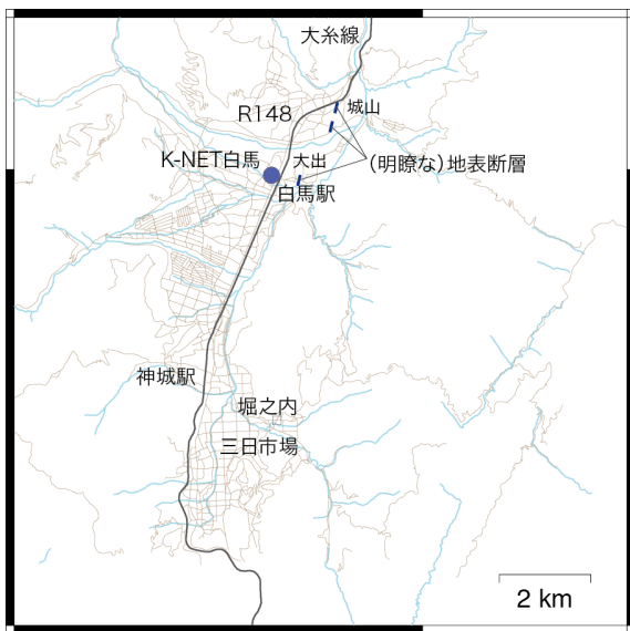
Fig.4 Location of K-NET NGN005 and damaged areas, Horinouchi and Mikka-Ichiba.
