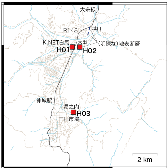
Fig.5 Location of aftershock recording sites.
