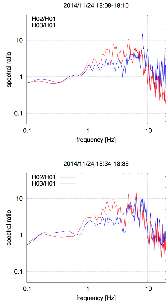
Fig.7 Spectral ratio of horizontal ground motions at H02 and H03 respect to H01.
