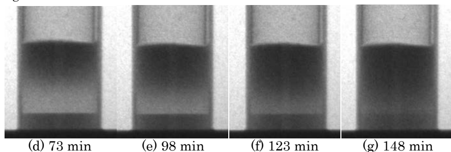
Fig. 2 Transient change in adsorption process.
