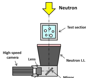
Fig. 1 Neutron imaging system with neutron image intensifier.
