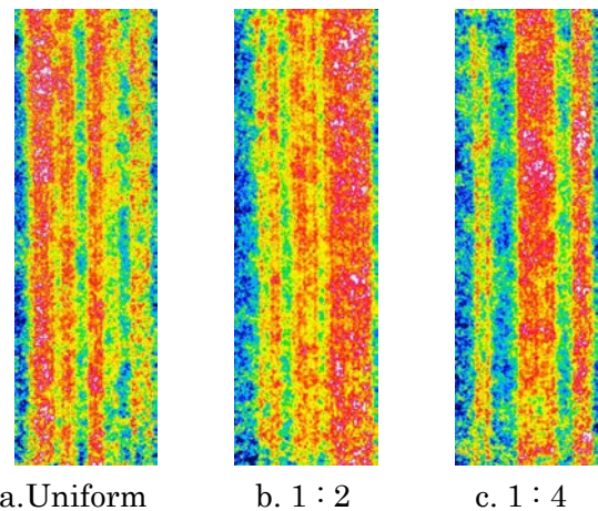
Fig.2 Example of the visualization results of void fraction x_{\text{eqave}}=0.188
