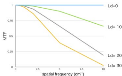
Figure 1: Typical shape of MTF according to the distance between sample and detector for a simple pinhole system.
