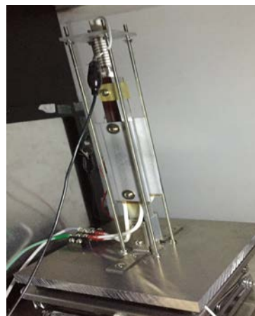
Figure 1 Photo of the apparatus.
