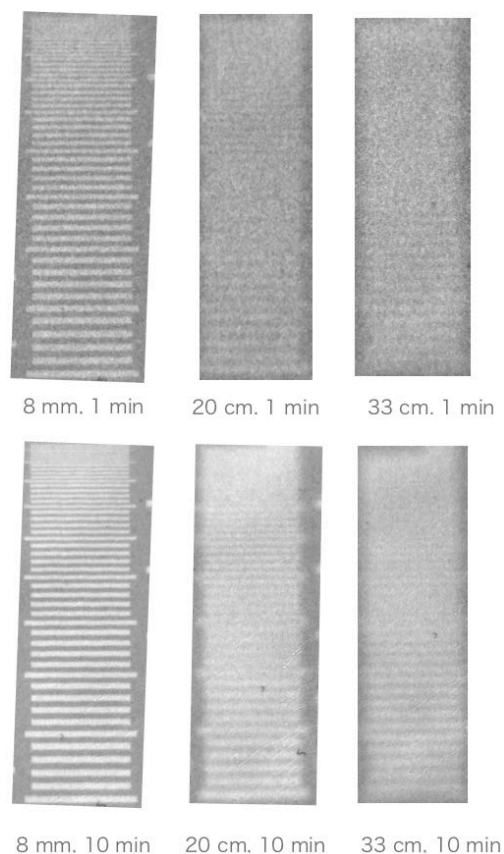
Figure 2: The transmission image of a standard indicator with various conditions. Not only the distance between sample and detector but also the measurement time affect the quality of image.
