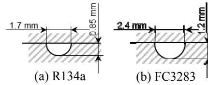
Fig.1 Channel cross-section
