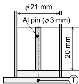
Fig. 1 Test cell
