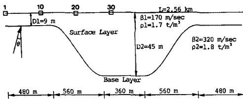
Fig. 4. 2-layered media model.
