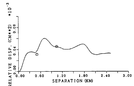
Fig. 24. Comparison of the mean squares of the relative displacements (thick line ; estimated value, o marks ; observation)
