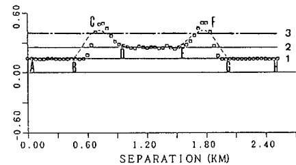
Fig. 16. Modeling of the mean powers. (2-layered media)
