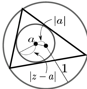
Figure 4: The equation (4) implies Chapple's formula.
