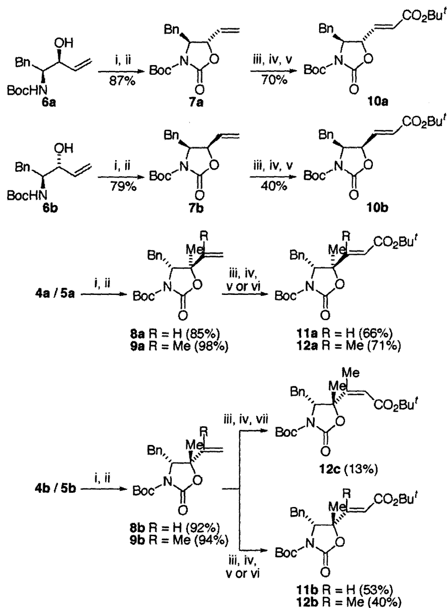
Scheme 4. Reagents: i , NaH, THF; ii , (Boc) 2 O; iii , O 3 gas, EtOAc or CH 2 Cl 2 ; iv , Me 2 S; v , (EtO) 2 P(O)CH 2 CO 2 Bu t , LiCl, (Pr t ) 2 NEt, MeCN; vi , Ph 3 P=CHCO 2 Bu t , CHCl 3 ; vii , Me 3 SiCH 2 CO 2 Bu t , (Cy) 2 NLi, THF.
