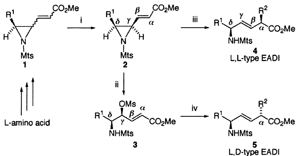
Scheme 1. R^1 , R^2 = alkyl; Ms = methanesulfonyl; Mts = 2,4,6-trimethylphenylsulfonyl. Reagents: i, \text{Pd}(\text{PPh}_3)_4 ; ii, MsOH in \text{CHCl}_3 ; iii, \text{R}^2\text{Cu}(\text{CN})\text{MgCl}\cdot 2\text{LiCl} ; iv, \text{R}^2\text{Cu}(\text{CN})\text{MgCl}\cdot \text{BF}_3 . D-Amino acids lead to D,D-type and D,L-type EADIs in the same way.
