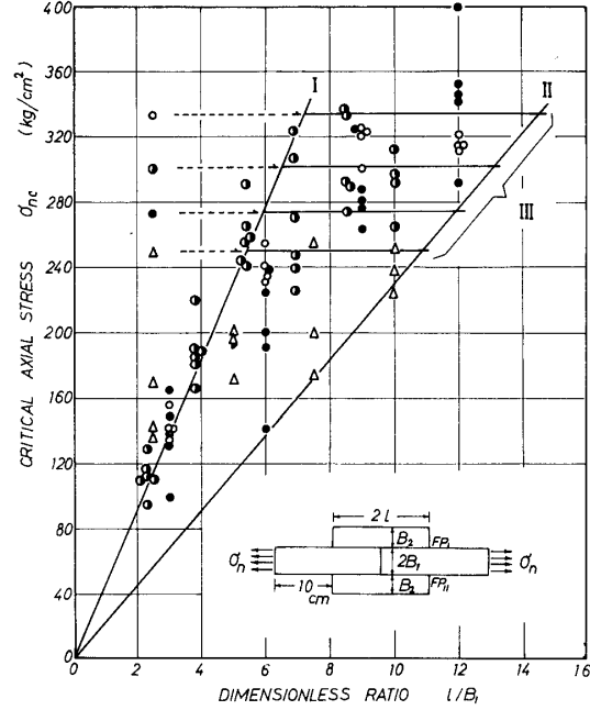
Fig. 13. Individual test result. Approximated linear relations between strength of double lap joints and aspect ratio l/B_1 (line-I and -II), and maximum strength of the joints (line-III). ○: B_1=1.0 , B_2=0.5 cm; ●: B_1=1.3 , B_2=0.6 cm; ●: B_1=B_2=1.0 cm; △: B_1=B_2=1.2 cm.
