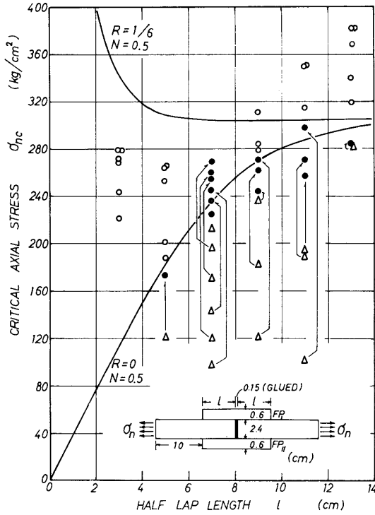
Fig. 12. Effect of stiffness of butt joint on the strength of double lap joints. Solid curves indicate strength predicted with eq. (14). ○: breakdown of whole specimen, ●: breakdown of specimen after a glued butt joint separation, △: partial separation at glued butt joint. Arrows indicate progresses from partial separation at glued butt joint to breakdown of whole specimen.
