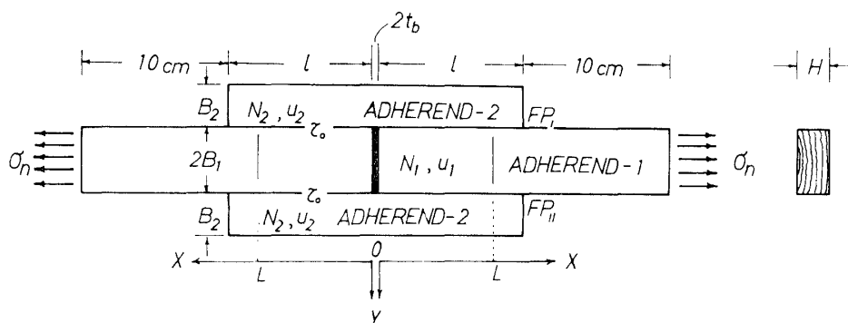
Fig. 1. Double lap joints specimen including a butt joint at the center. 2t_b is thickness of gap or glue line of the butt joint. Lines at x=L indicate the location of knifedge of the extensometer. Two corner points FP_I and FP_{II} are thought to be most critical for fracture initiation.
