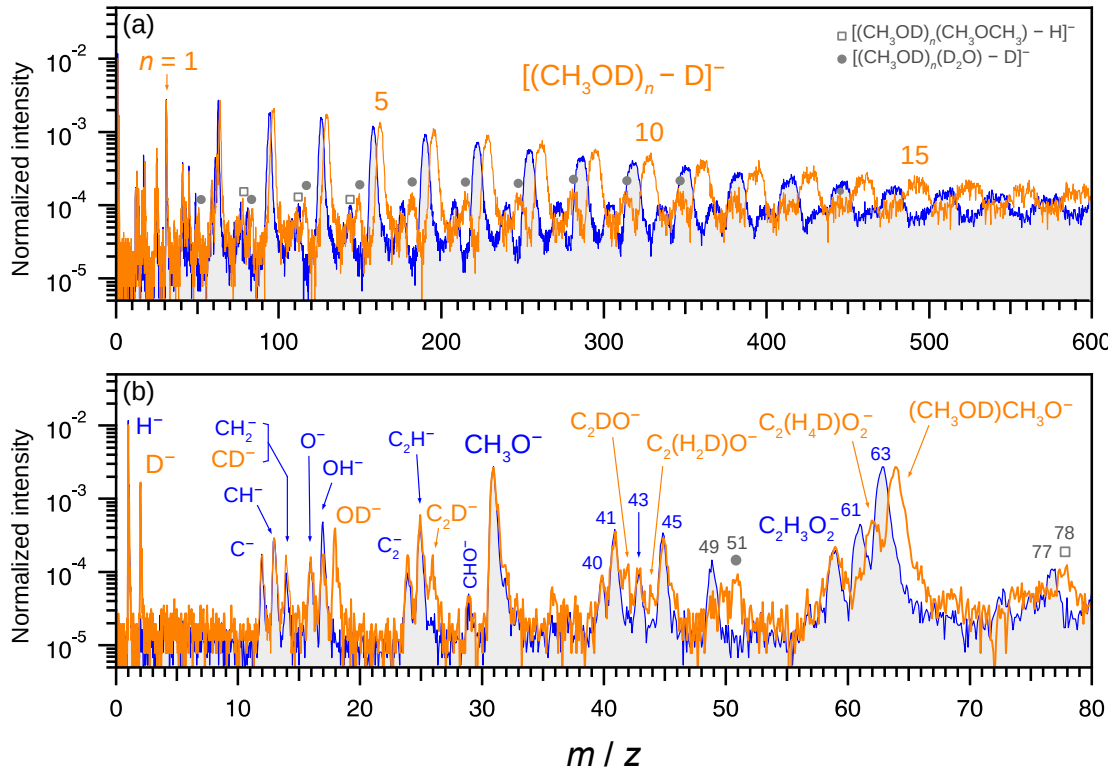
Figure 5. (a) Comparisons of mass spectra for negative secondary ions emitted from droplets of CH_3OD (orange line) and CH_3OH (blue line filled with gray). (b) Expanded mass spectra in the range of m/z < 80 . The vertical and horizontal axes are the same as in Figure 1.
