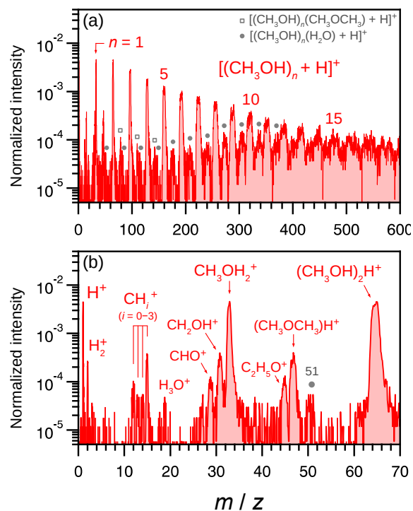
Figure 1. (a) Mass spectrum of the positive ions from CH_3OH droplets induced by 2.0-MeV C^{2+} . The vertical axis represents the counts divided by the number of start triggers. (b) Expanded mass spectrum in the range of m/z < 70 .
