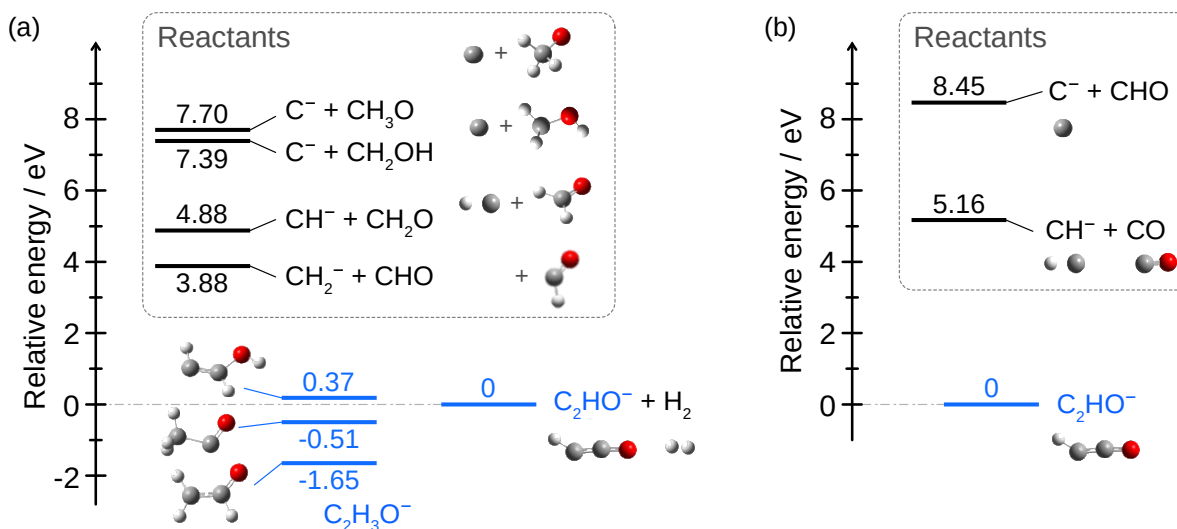
Figure 7. Energy levels regarding the association reactions into (a) \text{C}_2\text{H}_3\text{O}^- and (b) \text{C}_2\text{HO}^- .
