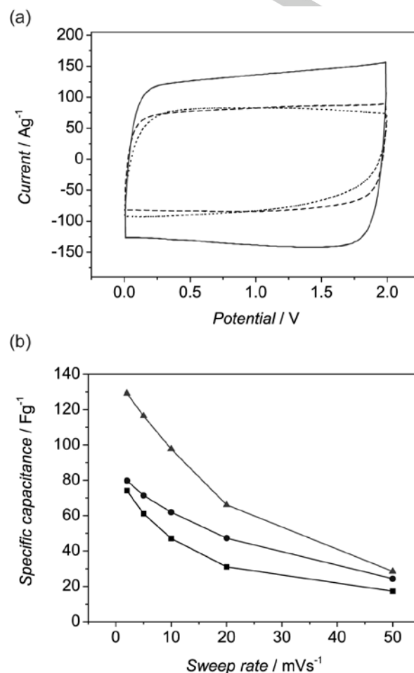
Figure 7. (a) Cyclic voltammograms at 2 \text{ mV s}^{-1} for CID-H-1000 (dot), CID- \text{NO}_2 -1000 (dash) and ZnNipdpe-1000 (solid line). (b) Specific capacitances of CID-H-1000 (squares), CID- \text{NO}_2 -1000 (circles) and ZnNipdpe-1000 (triangles) at different sweep rates.
