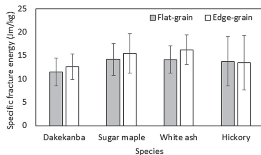
Fig. 9. Specific fracture energy collected at TrueSoG = 0 of dakekanba and bat materials in impact bending.
