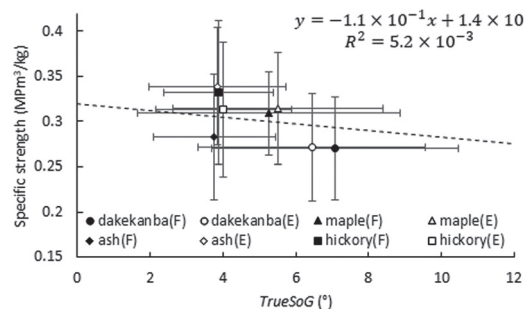
Fig. 6. Specific strength of bat-grip-like, cylindrical specimens in impact bending. F: flat-grain specimen, E: edge-grain specimen, error-bar: standard deviation.
