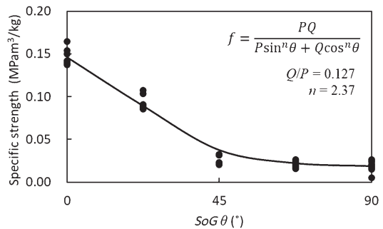
Fig. 3. Relationship between SoG and specific fracture strength.
