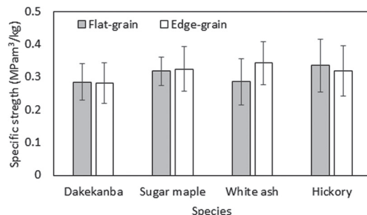
Fig. 8. Specific strength collected at TrueSoG = 0 of dakekanba and bat materials in impact bending.
