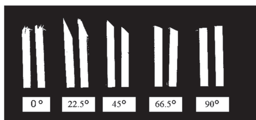
Fig. 5. Fracture surface of dakekanba small-specimens in impact bending tests.
