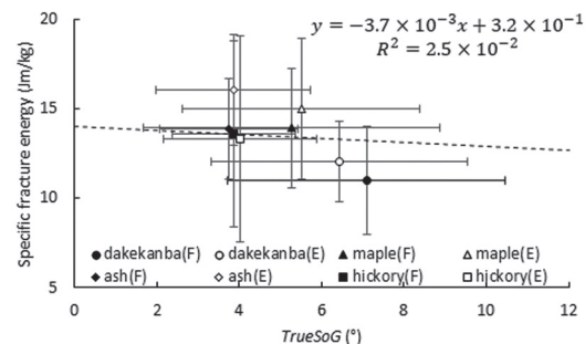
Fig. 7. Specific fracture energy of bat-grip-like, cylindrical specimens in impact bending. F: flat-grain specimen, E: edge-grain specimen, error-bar: standard deviation.
