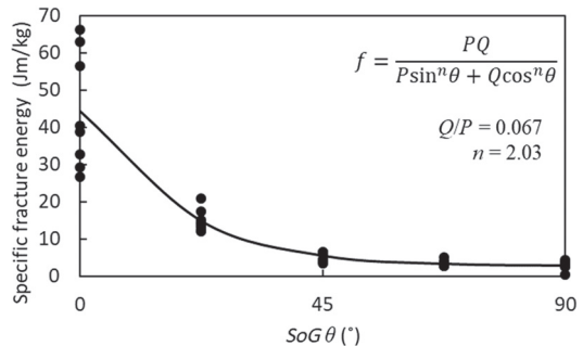
Fig. 4. Relationship between SoG and specific fracture energy.
