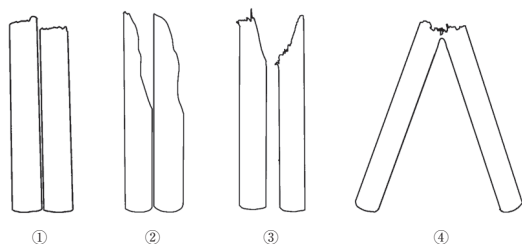
Fig. 10. Shapes of fracture surface of cylindrical specimens.
