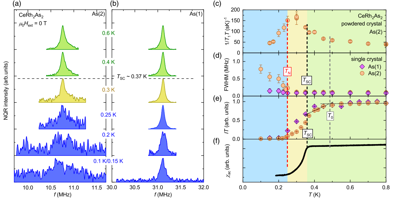
FIG. 2. Summary of the anomalies detected by NQR measurements. ^{75}\text{As} NQR spectrum of (a) As(2) and (b) As(1) sites at several temperatures in \text{CeRh}_2\text{As}_2 . Each spectrum is shifted to avoid overlapping. Temperature dependencies of (c) 1/T_1T (d) FWHM of NQR spectrum, (e) NQR intensity multiplied by temperature I(T)T of each As site, and (f) ac susceptibility. For comparison, I(T)T at each site is normalized by its value at 1.0 K. The characteristic temperatures T_N , T_{SC} , and T_0 are indicated by the dashed lines. The errors of the FWHM and IT are determined from the resolution of NQR signals.
