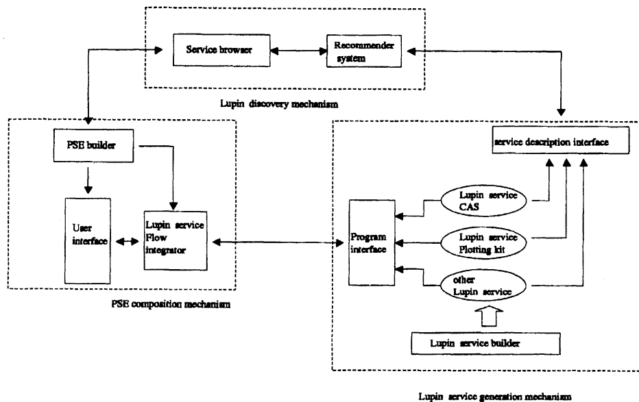
Figure 2: Lupin's conceptual architecture
