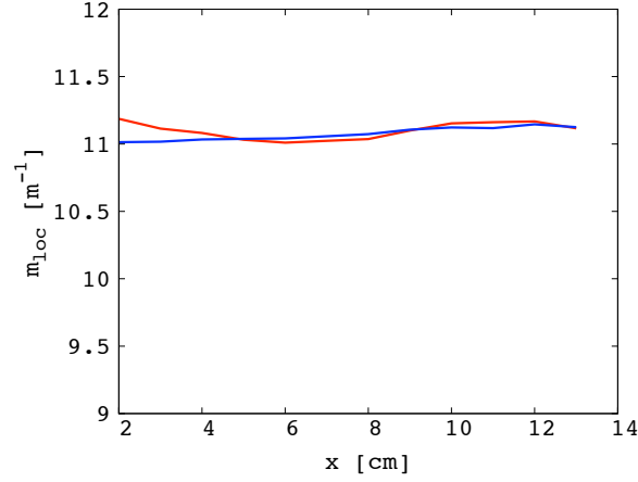
Figure 3.33: Comparison of local m -value in TOSCA map (blue) and in measured map (red) in the good field region.
