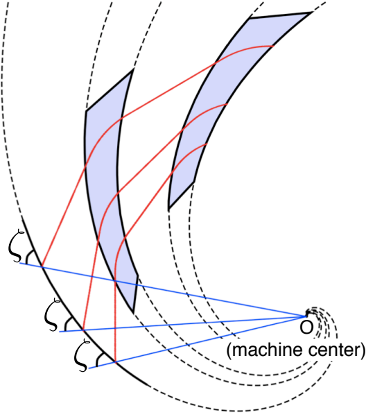
Figure 2.5: Spiral case.
