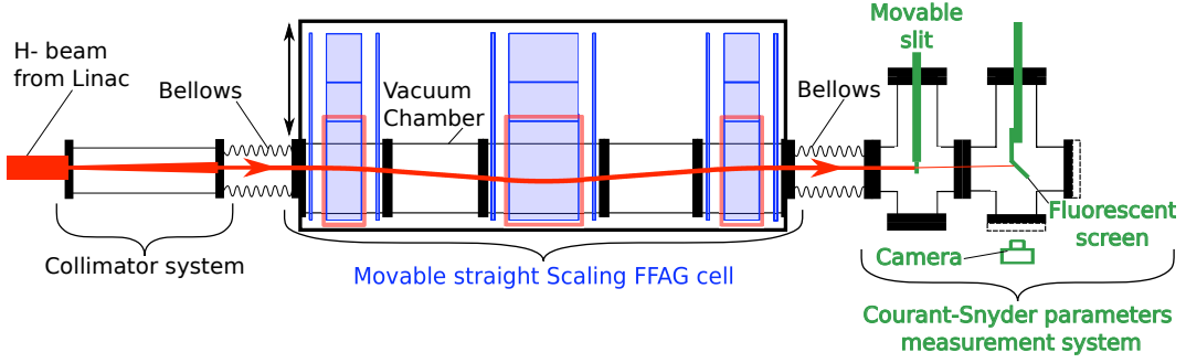
Figure 3.2: Schematic view from above of the experiment.
