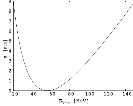
Figure 2.11: Mismatch of reference trajectories between circular cells and straight cells in 150 MeV FFAG ring example.
