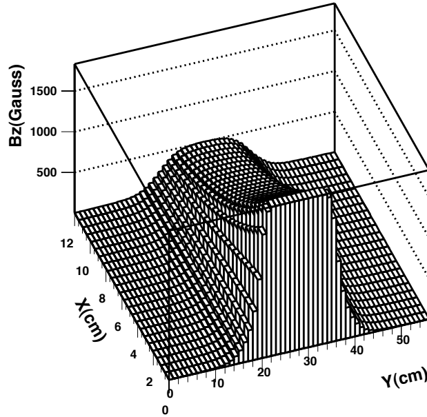
Figure 3.23: Field map of the magnet F 1 in the mid-plane.
