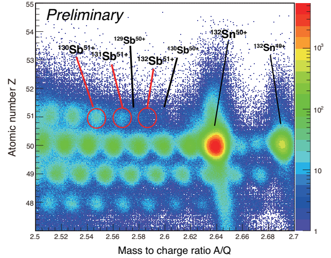
Figure 3. (Color online) A PID spectrum in the SAMURAI spectrometer for reacted events associated with the ^{132}\text{Sn} beam.
