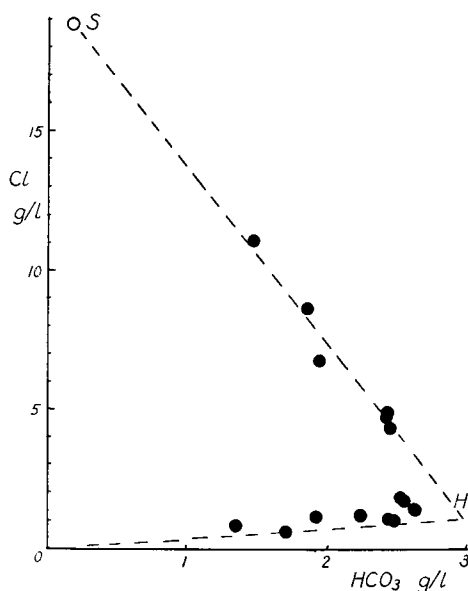
Fig. 8. Relation between \text{Cl}^- and \text{HCO}_3^- in Shirahama Hot Springs.
