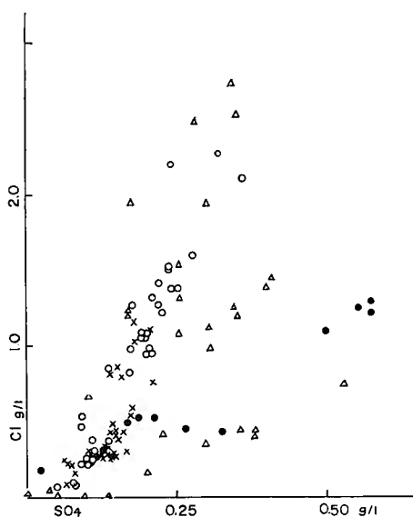
Fig. 3. Relation between \text{Cl}^- and \text{SO}_4^{2-} contents of hot spring waters in northern region of Beppu Spä. Marks in figure are the same as in Fig. 2.
