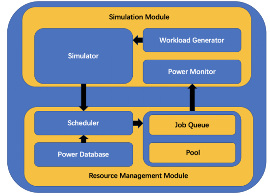
Fig. 1. Simulator architecture
