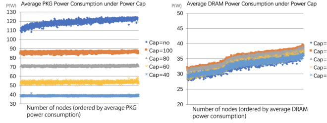
Fig. 6. Power consumption of HPCG under different power caps
