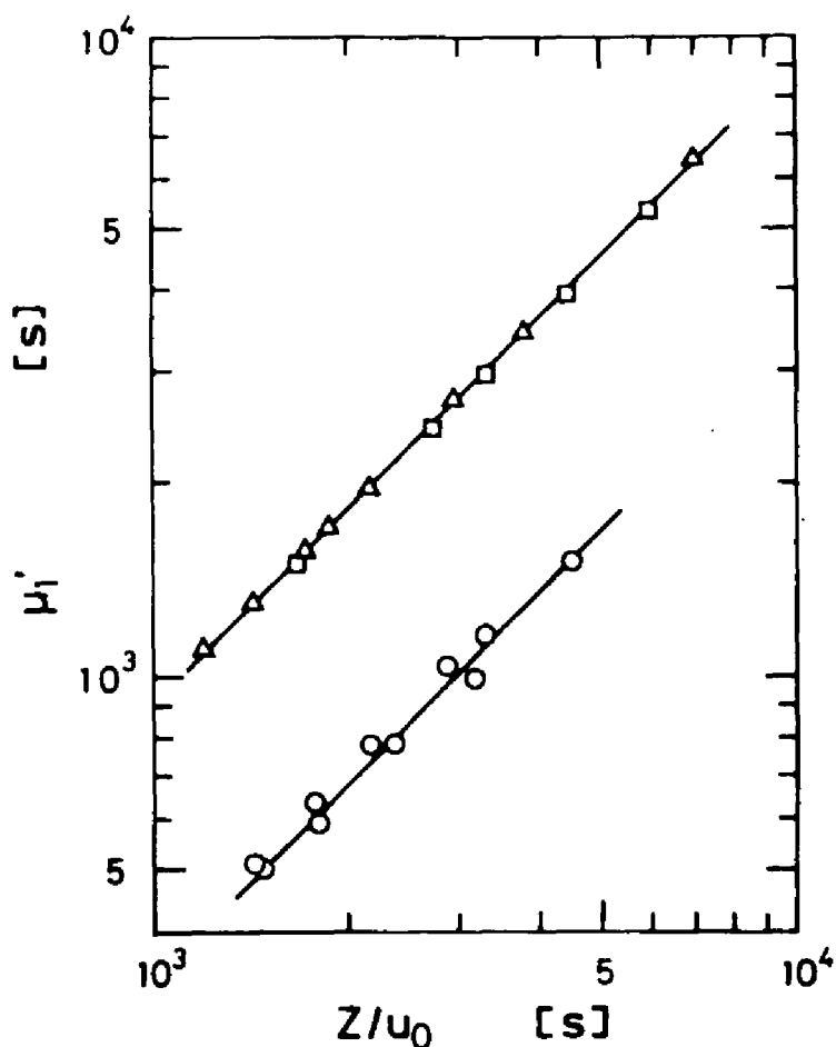
Fig. 6-3. Experimental relations between first-order statistical moment and Z/u_0 . Column size = 15.4 mm \phi X 383 mm. Sample volume applied was 0.5 ml. ( \circ ) 0.3% Blue Dextran; ( \square ) 0.01 mol/l sucrose; ( \triangle ) 0.01 mol/l glucose.
