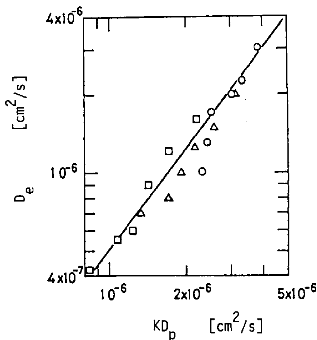
Fig. 1-7. Experimental relations between D_e and KD_p for various saccharides in acrylamide gels. The experimental data shown in Fig. 1-5a were employed.
