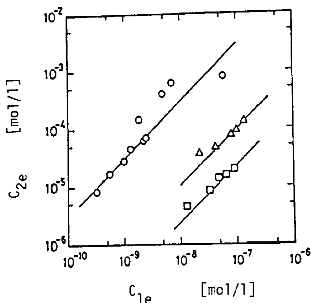
Fig. 5-1. Relation between C_{2e} and C_{1e} at pH 5.0 and 25°C. The C_{1e} and C_{2e} are the equilibrium glucoamylase concentration in outer solution and that in SP-Sephadex. ○, SP-Sephadex C-50 in 0.01 mol/l acetate buffer; □, C-50 in 0.05 mol/l and △, C-25 in 0.01 mol/l.
