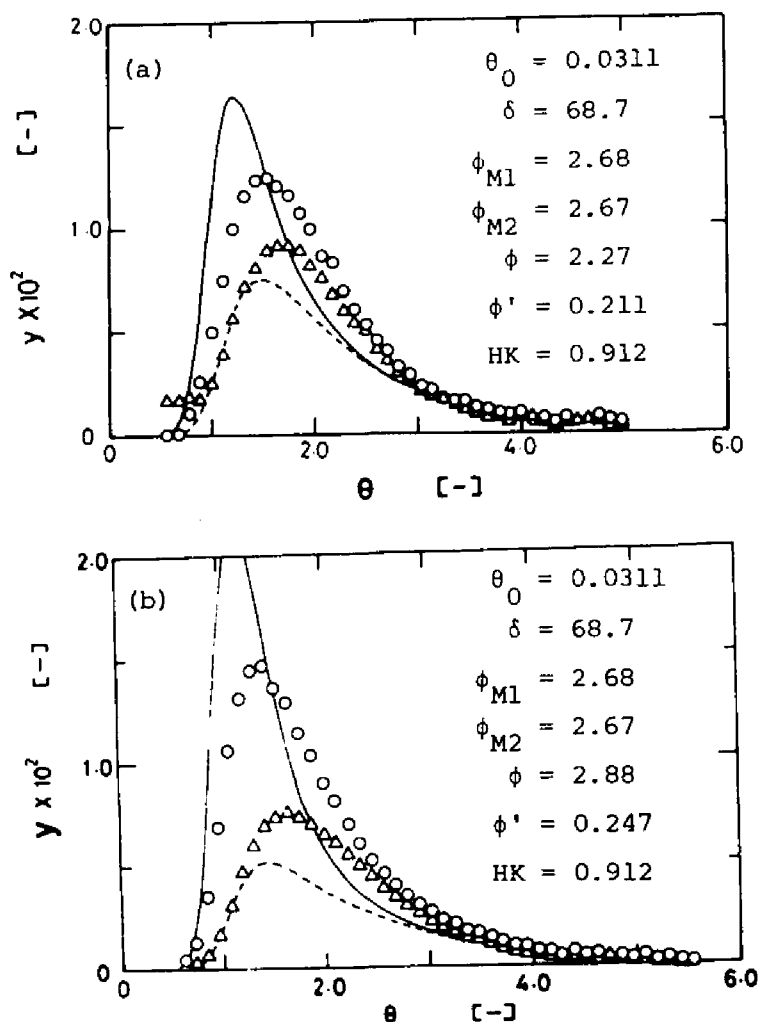
Fig. 7-1. (a) Elution profiles of glucose and fructose in an immobilized-glucose isomerase column in run 2. The symbols ( \bigcirc ) and ( \Delta ) correspond to glucose and fructose, respectively. The solid and broken curves were calculated for glucose and fructose according to the theory using the values of the dimensionless parameters listed in the figure. (b) Elution profiles of glucose and fructose obtained for run 4. The symbols are as shown in (a). The dimensionless parameters used for calculating the theoretical curves are listed in the figure.
