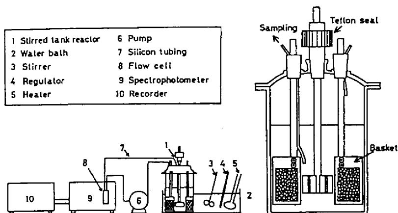
Fig. 3-1. Schematic representation of isothermal batch reactor including immobilized- \alpha -chymotrypsin particles.
