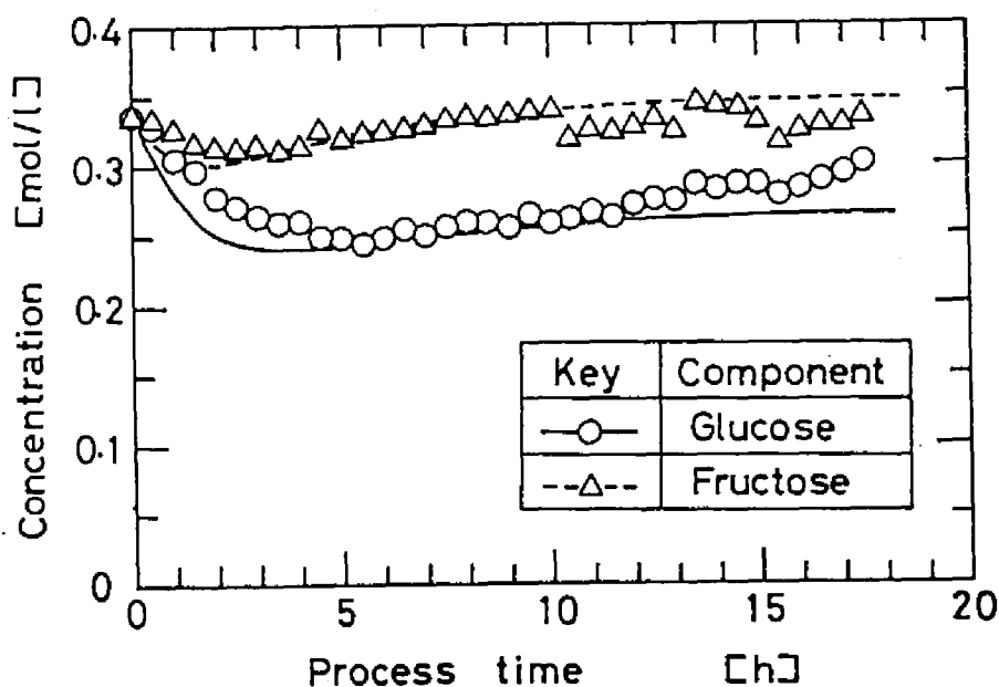
Fig. 12-6. Time courses of glucose and fructose concentrations in product stream in run R-7. The solid and broken curves were calculated for glucose and fructose, respectively, by using the intermitted moving-bed model.
