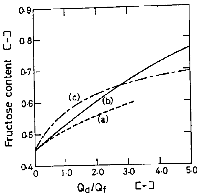
Fig. 13-4. Comparison of three processes for production of higher fructose syrup. Broken, solid, and dot-dash curves (curves (a), (b), and (c)) correspond with processes (a), (b), and (c) in Fig. 13-1. This figure shows that process (c) (the process proposed) requires the smallest amount of desorbent to produce higher fructose syrup with 45 to 65% fructose content.
