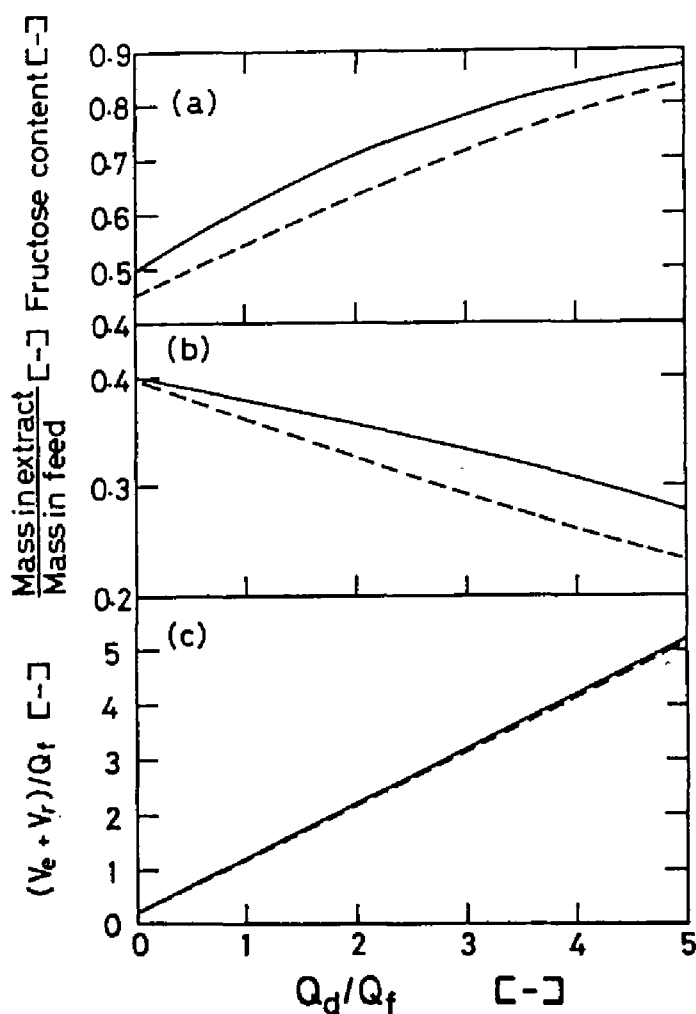
Fig. 13-12. Comparison of performance of the modified system including adsorption process and immobilized-glucose isomerase reaction with that of the simulated moving-bed adsorber. The solid and broken curves denote the modified system and the simulated moving-bed adsorber, respectively. (a) Fructose content in extract solution. (b) Ratio of mass in extract solution to that in feed solution. (c) ratio of amount of water evaporated per unit time to the volumetric flow rate of feed solution. The standard conditions for comparison are shown in Table 13-3.
