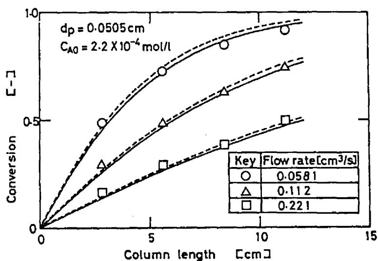
Fig. 3-9. Comparison of experimentally obtained concentration profiles in tubular reactor with profiles predicted by using the parameters estimated by method II. The solid and broken curves were calculated with and without consideration of film mass transfer resistance.
