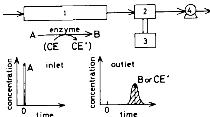
Fig. II-1. Schematic representation of analysis based on a pulse response in an immobilized-enzyme column. A denotes the substrate, which is undetectable in its original form and the concentration of which is unknown, and B is the detectable product. CE is a coenzyme of undetectable form and CE' is one of detectable form. Concentration of the substrate A is determined from the intensity of the elution profile, such as the peak height or the area under the curve of product or CE'. 1, Immobilized-enzyme column; 2, detector; 3, recorder; 4, constant-feeding pump.
