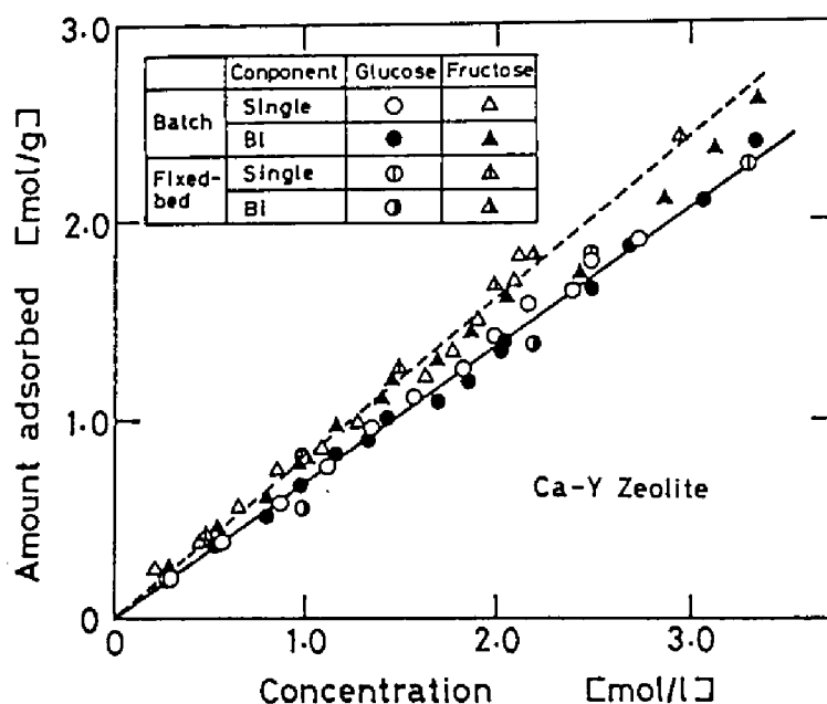
Fig. 10-4. Adsorption isotherms of glucose and fructose on Y zeolite ( \text{Ca}^{2+} form) at 50^{\circ}\text{C} . The amounts of glucose and fructose adsorbed were estimated by using both the batch desorption method and the analysis of breakthrough curves in fixed-bed adsorber. As a solvent, 0.02 \text{ mol/l} Tris-HCl buffer containing 0.01 \text{ mol/l} magnesium sulfate was used.
