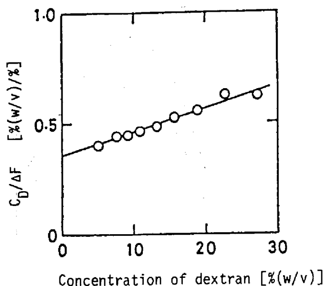
Fig. 4-7. Plot of C_D/\Delta F versus Concentration of dextran for fluorescence titration of glucoamylase with dextran at pH 4.5 and 25°C. Glucoamylase concentration, 1.33 \times 10^{-6} mol/l; wavelength of excitation, 285 nm; wavelength of emission, 340 nm.
