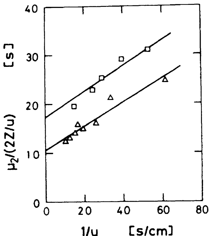
Fig. 6-4. Experimental relations between second-order central moment and 1/u . ( \square ) 0.01 mol/l sucrose; ( \triangle ) 0.01 mol/l glucose.
