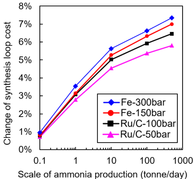
Fig. 8. The sensitivities of synthesis loop cost when energy price increases by 10% (i.e., the case that the energy price increased from 0.0683 USD/kWh to 0.07513 USD/kWh).
