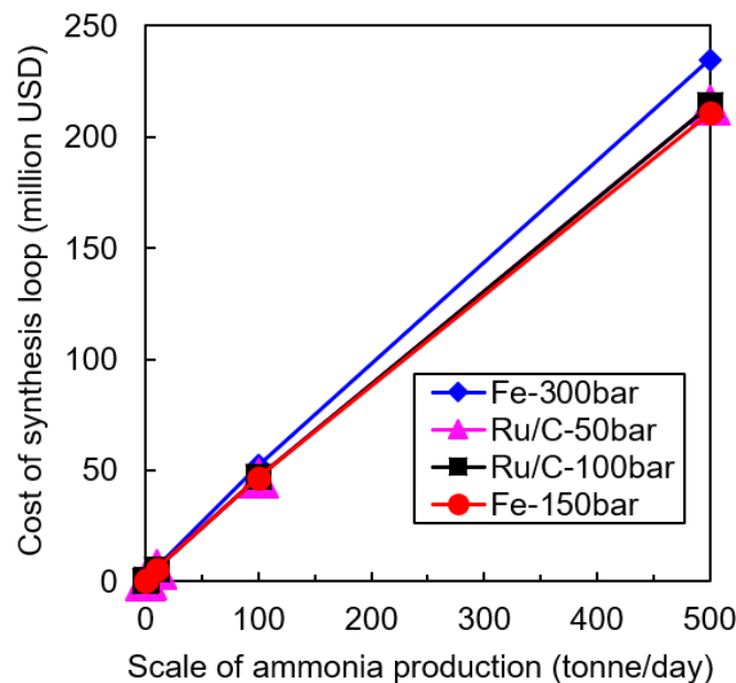
295 Fig. 5 The total cost of the ammonia synthesis loop against the production scale.
