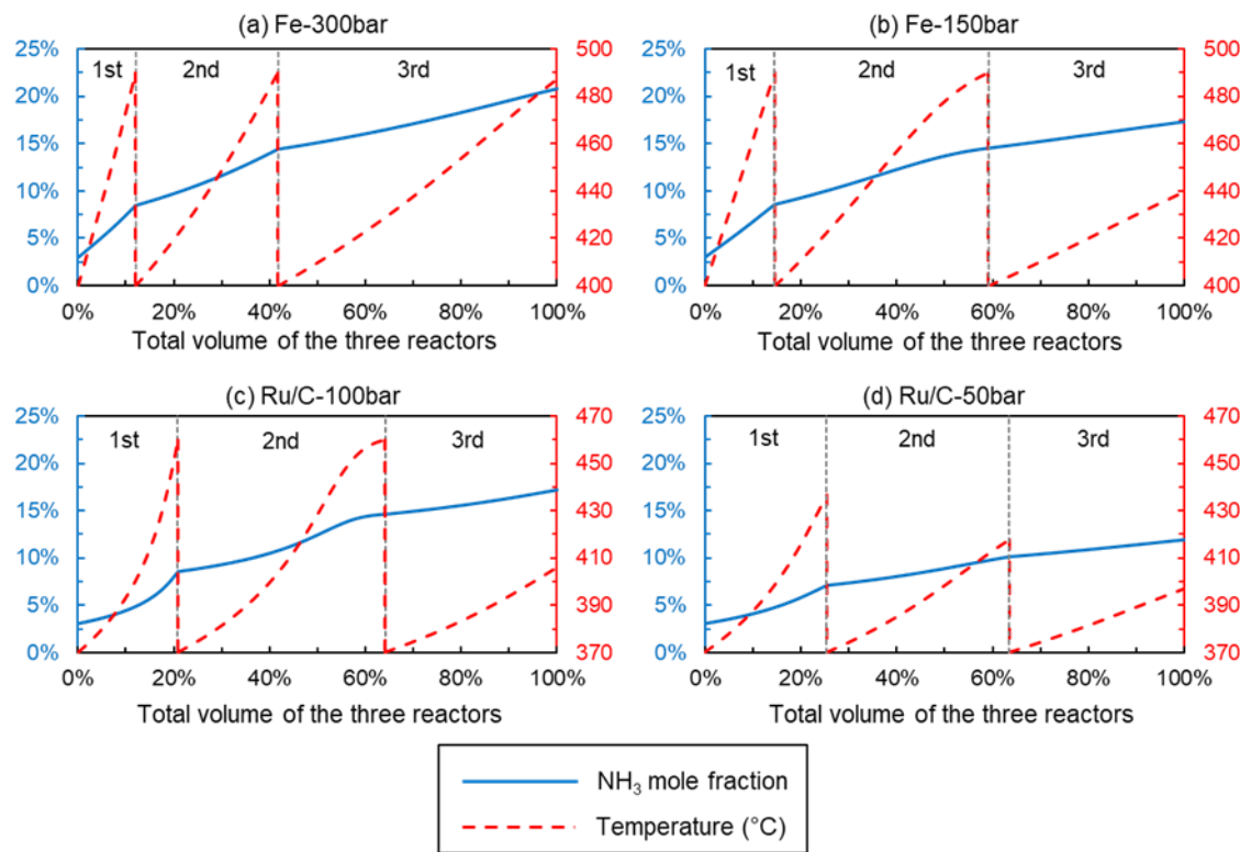
Fig. 4. NH 3 concentration and temperature change in the simulated three-bed reactor system in the ammonia synthesis loops, (a) Fe-300bar, (b) Fe-150bar, (c) Ru/C-100bar, (d) Ru/C-50bar.
