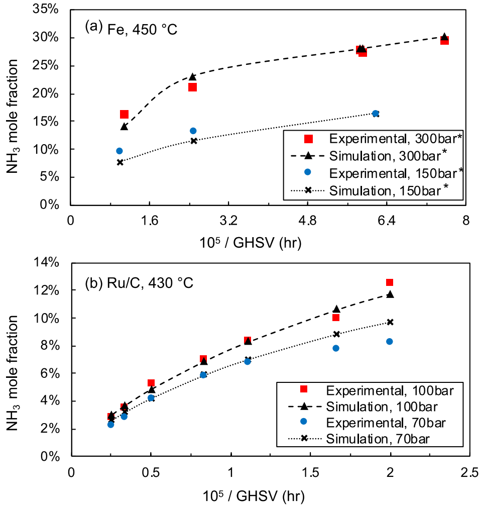
Fig. 3. Comparison of the experimental data with the reactor simulation results of a single pass over a reactor, (a) for Fe at T = 450\text{ }^{\circ}\text{C} , *P = 304\text{ bar} ( =300\text{ atm} ) and 152\text{ bar} ( =150\text{ atm} ), and \text{H}_2/\text{N}_2 = 3.0 [52], (b) for Ru/C T = 430\text{ }^{\circ}\text{C} , P = 100\text{ bar} and 70\text{ bar} , and \text{H}_2/\text{N}_2 = 3.0 [53].
