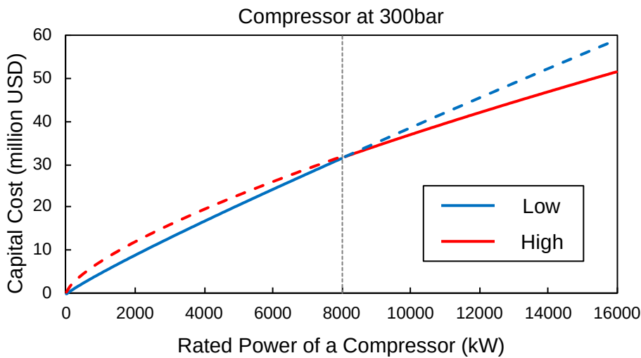
Fig. B.1. The capital cost of a compressor by two types of parameters.
