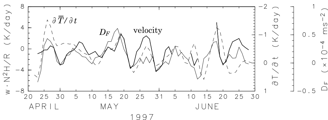
Figure 5. Vertical velocity estimated by the \text{N}_2\text{O} 0.1 ppmv isoline at \sim 600 – 500 K ( \sim 23 – 20 km; thick line). D_F at 10 hPa ( \sim 30 km) and 70^\circ\text{S} in geographical latitude (thin line). \partial \bar{T}/\partial t at 46.4 hPa ( \sim 20 km) from UKMO temperature averaged in 90^\circ – 70^\circ\text{S} in geographical latitude (dashed thin line: the axis is reversed). A 3-day running mean is applied to the vertical velocity and \partial \bar{T}/\partial t , and a 5-day running mean is applied to D_F .
