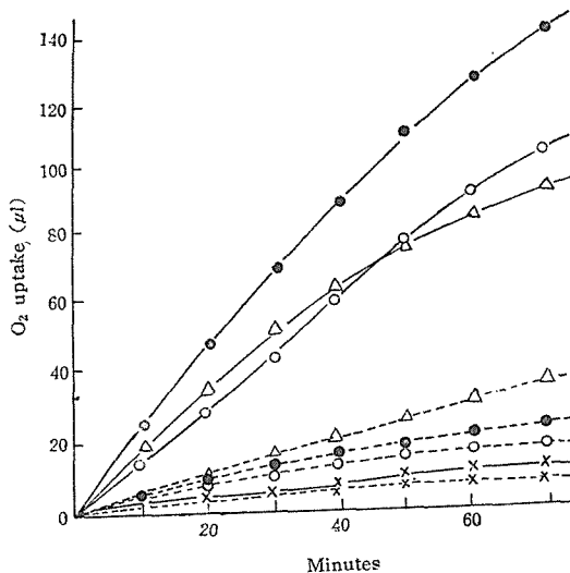
Fig. 2. Effect of pyocyanine on respiration of cell autolysate. Experimental method and material were the same as in Table 2. (···●···) Glucose, (—●—) glucose plus pyocyanine, (···○···) lactate, (—○—) lactate plus pyocyanine, (···△···) succinate, (—△—) succinate plus pyocyanine, (···×···) glycerol, (—×—) glycerol plus pyocyanine.
