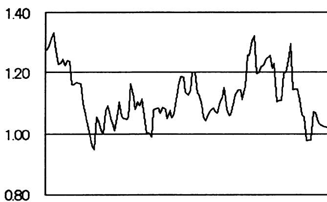
Fig.4.7: A sample path in the case of \alpha = 0.7 , \delta = 0.58 , and \rho = 0.0009
