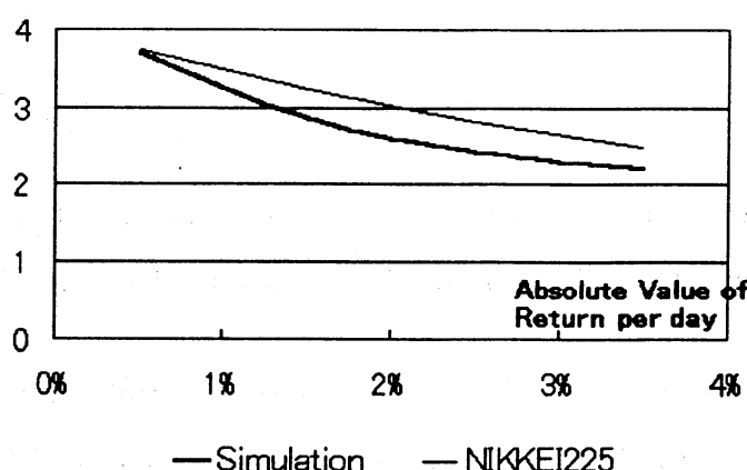
Fig.4.8: The log of the p.d.f. in the case of \alpha = 0.7 , \delta = 0.58 , and \rho = 0.0009
