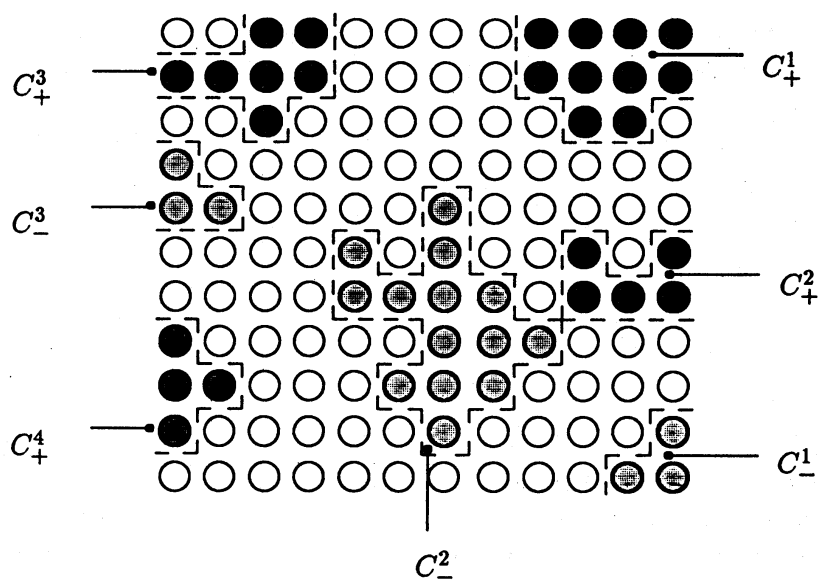
Fig.2.4: The Stauffer-Penna model
