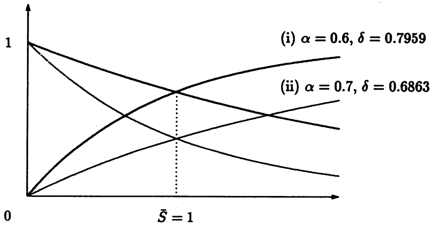
Fig.4.3: p^u and p^d in the case of Fig.4.2 (i) and (ii)
