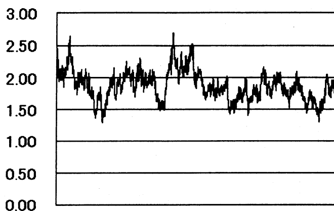
Fig.4.4: A sample path in the case of \alpha = 1.6 , \delta = 0.030 , and \rho = 0.015
