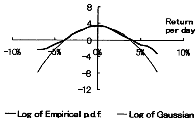
Fig.1.2: The log of the empirical p.d.f. for NIKKEI 225 returns per day
