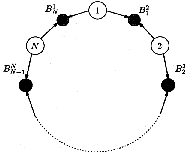
Fig.3.1: The S^1 network structure of the market
