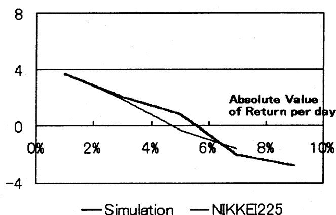
Fig.4.5: The log of the p.d.f. in the case of \alpha = 1.6 , \delta = 0.030 , and \rho = 0.015
