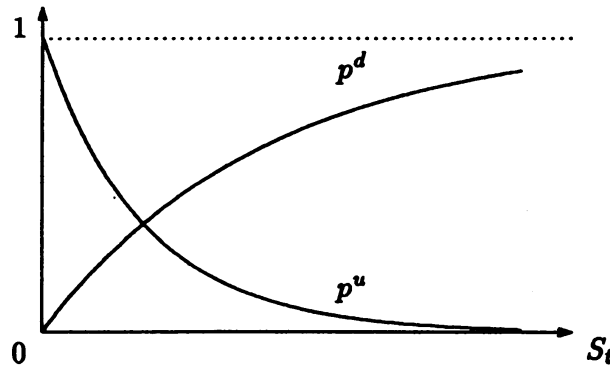
Fig.3.2: The influence rates of bull and bear order
