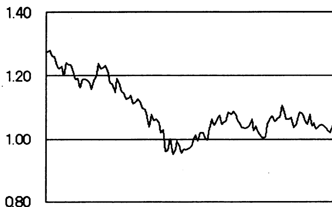
Fig.4.6: NIKKEI 225 from Jul.2001 to Dec.2001
