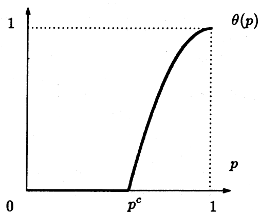
Fig.2.3: The percolation probability
