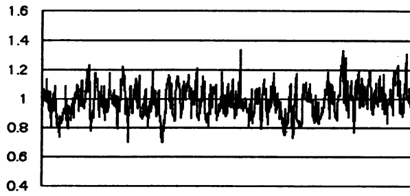
(ii) \alpha = 0.7, \delta = 0.6863, \rho = 0.5, N = 441
