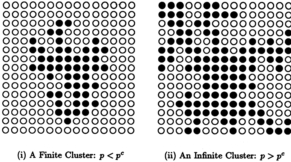
Fig.2.2: The phase transition in percolation
