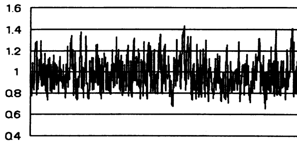
(i) \alpha = 0.6, \delta = 0.7959, \rho = 0.5, N = 441
