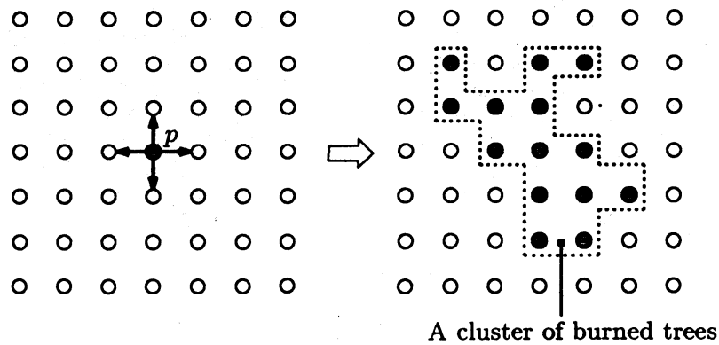
Fig.2.1: Percolation of a forest fire
