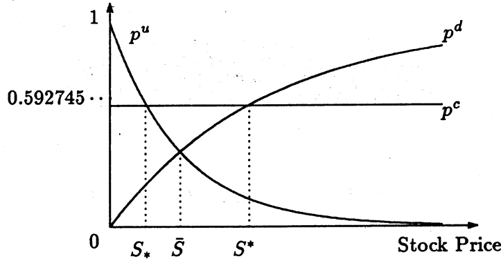
Fig.4.1: The floor and ceiling for S
