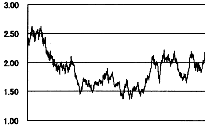
Fig.3.4: A sample path of S in the case of \alpha = 1.4 , \delta = 0.44 , \rho = 0.008 , N = 21
