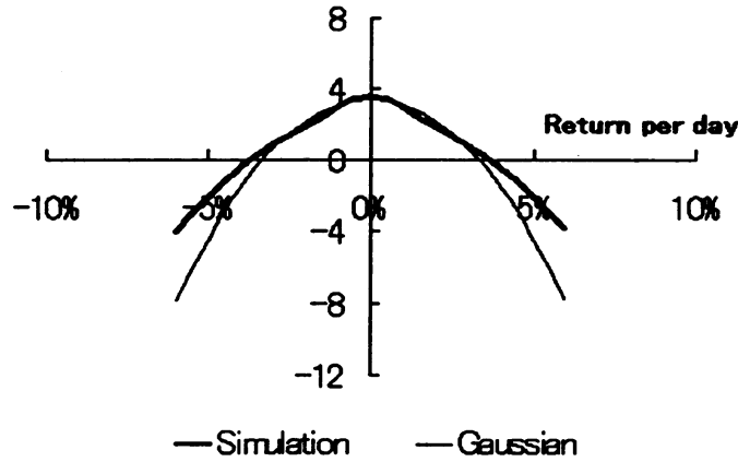
Fig.3.5: The log of the p.d.f. for the returns of S in Fig.3.4
