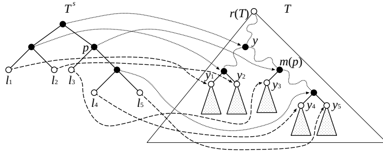
Figure 3: Example of a skeleton tree T^s and a mapping m . Dotted arrows represent m(p) , and dashed arrows represent the resulting mapping between leaves of T^s and \{y_1, \dots, y_D\} , where D = 5 in this example.
