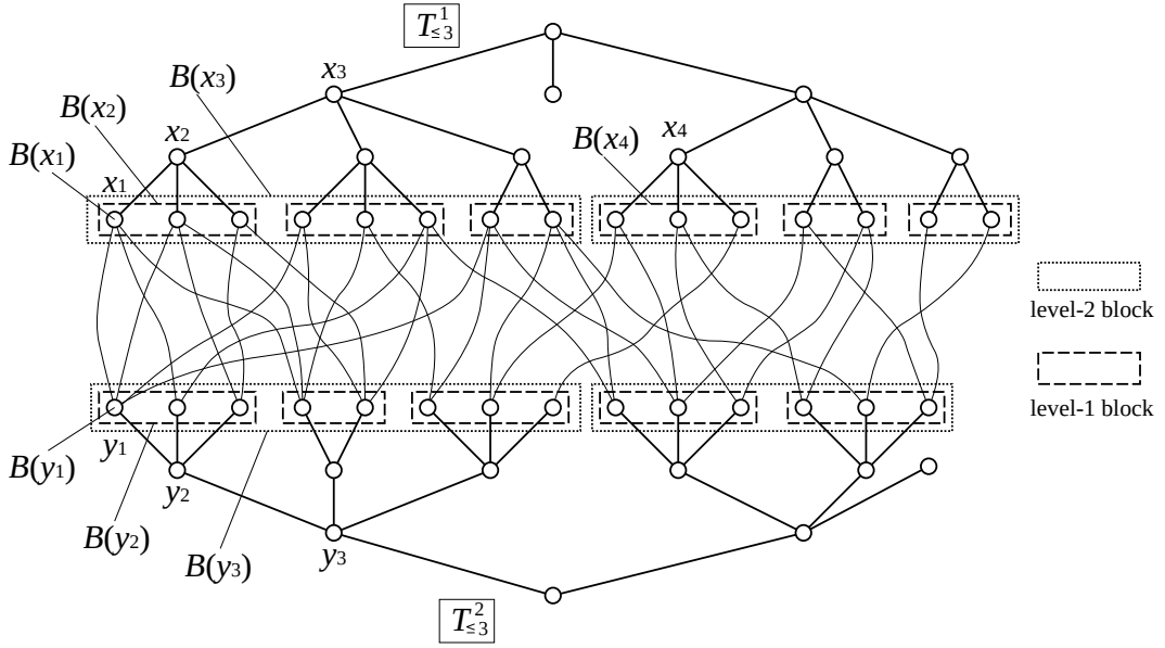
Figure 7: Illustration for degree constraints in CandPairs(T_{\leq 3}^1, T_{\leq 3}^2) . In this example, \deg(B(x_1), B(y_2), P) = 2 , \deg(B(x_1), B(y_3), P) = 3 , \deg(B(x_2), B(y_1), P) = 2 , \deg(B(x_2), B(y_2), P) = 5 , \deg(B(x_2), B(y_3), P) = 8 , \deg(B(x_3), B(y_3), P) = 17 , \deg(B(x_4), B(y_2), P) = 0 , and \deg(B(x_4), B(y_3), P) = 2 , where curved edges denote those in the current P . Note that this figure does not illustrate the procedure itself.
