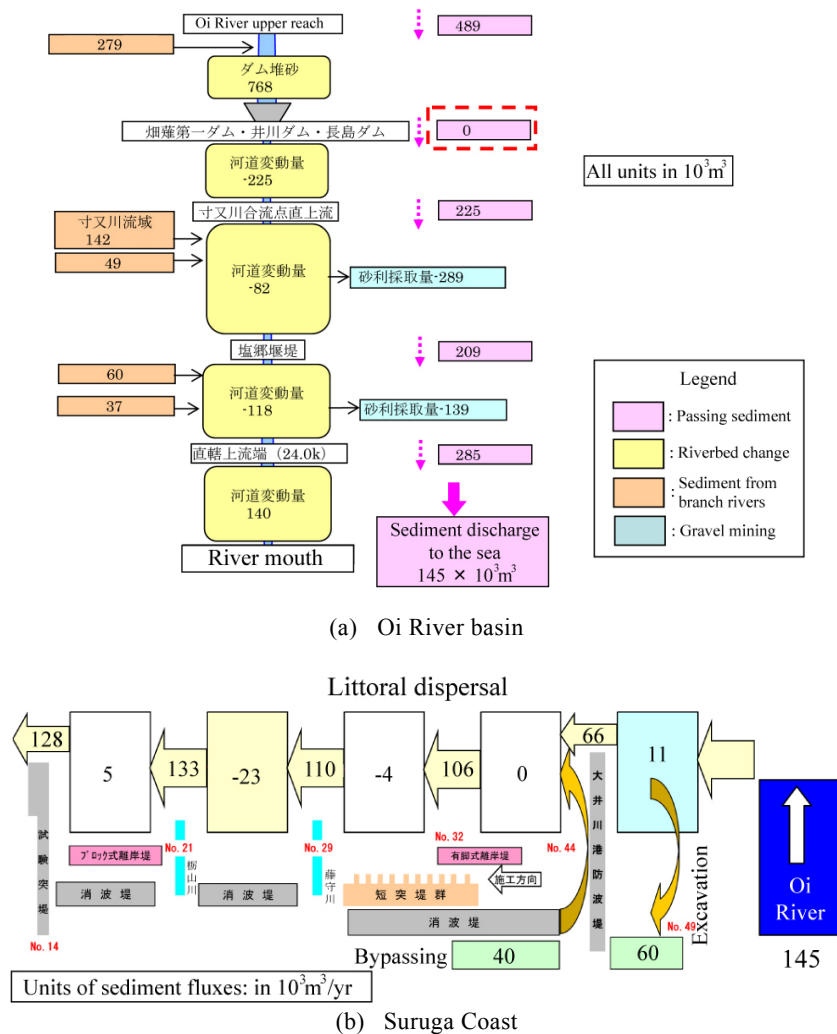
Fig. 11 Sediment routing system linking Oi River basin with Suruga coast (adapted from MLIT, 2009)
