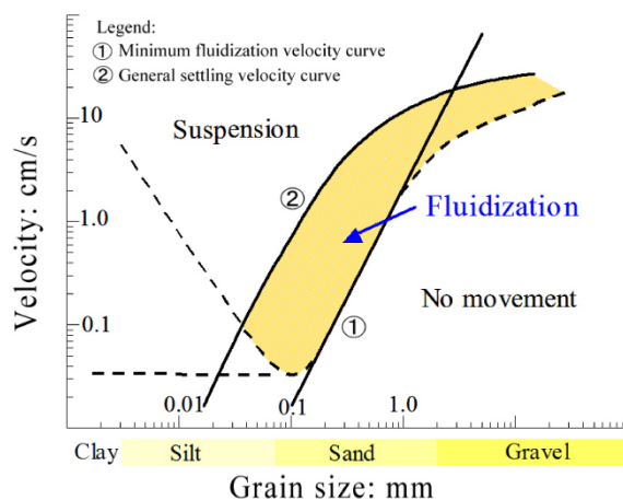
Fig. 12 Variations of critical velocities with grain size (adapted from Lowe, 1975)
