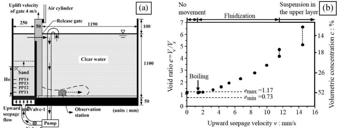
Fig. 13 Changes in states of soil with increasing upward seepage velocity (Amiruddin et al. , 2006)
