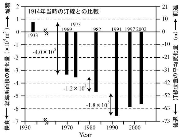
Fig. 18 Long-term changes of beach area
