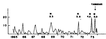
Fig. 10 Monthly numbers of earthquakes in an area of 35 km \times 30 km centering around the Yamasaki earthquake in Sept., 1973.
