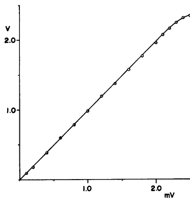
Fig. 18 Linearity of telemetric transmission system. Abscissa and ordinate denote input from seismometer to pre-amplifier and output from transmission system, respectively.
