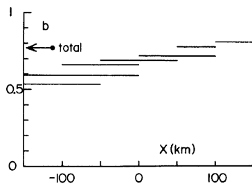
Fig. 3. Regional variation of the b-value in Gutenberg-Richter's relation. (after Oike) x = 0 corresponds to 134^{\circ}30'E .
