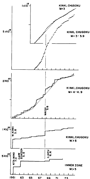
Fig. 4. Cumulative graphs of seismic energy released in several magnitude levels. Upper two graphs are due to observations by the Tottori Microearthquake Observatory, and the others by the Japan Meteorological Agency.
