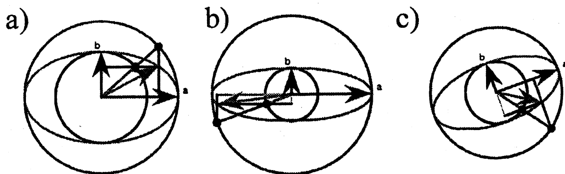
Figure 3: Polar angle parameter description an ellipse: a) polar angle in first quadrant, b) polar angle in third quadrant with change of |b| , c) changing the semi-axis.
