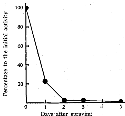
Fig. 4. Change of radioactivity on and in rice plant after spraying.
