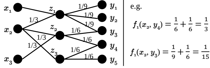
Figure 3.3: An example: calculation of Probability heuristic values of one-to-one candidates of x_2
