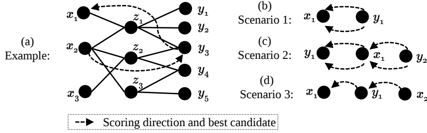
Figure 3.5: Inconstancy and three basic scenarios in best candidate selection during bi-directional scoring. Note that x and y used in sub figures (b), (c) and (d) are not relevant to one in (a)
