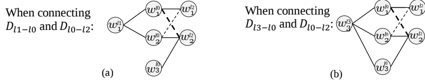
Figure 5.1: Different weights can be obtained for an edge from different combinations of input dictionaries; for the same edge e(w_1^{l0}, w_2^{l2}) two different weights are obtained
