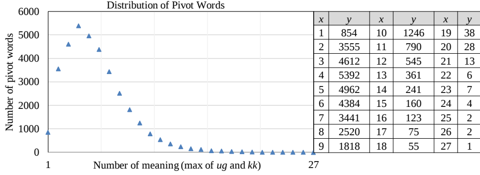
Figure 4.5: Quantity distribution of pivot words over the number of meanings, which implies the availability of relatively large number of ambiguous words in the pivot language.
