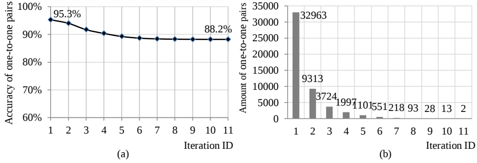
Figure 3.6: Evaluation details of the iterations I: (a) Correlation between iteration and accuracy of accumulated one-to-one pairs; (b) Correlation between iteration and amount of one-to-one pairs induced at each iteration
