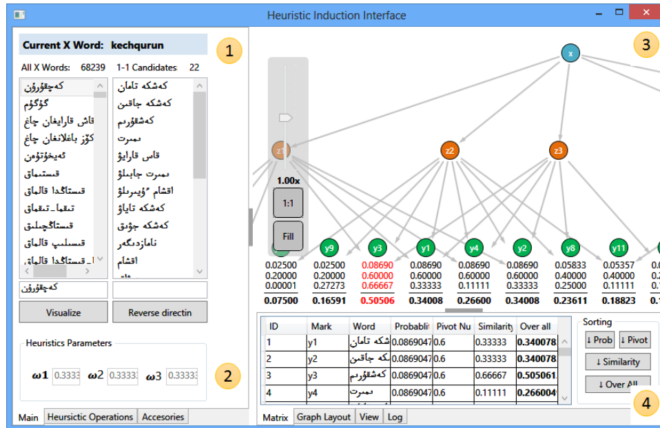
Figure 6.1: A screen-shot of the tool of heuristic framework. (1) An area to display words in the target languages of output dictionary. (2) An area to setup weights of the heuristics. Notice that the experimental tool only allows three heuristics to be defined. (3) An area to display transgraph where all the candidates of given word and their structures are displayed. (4) Result of details of the scoring where detailed scores of each heuristics and candidates are provided.
