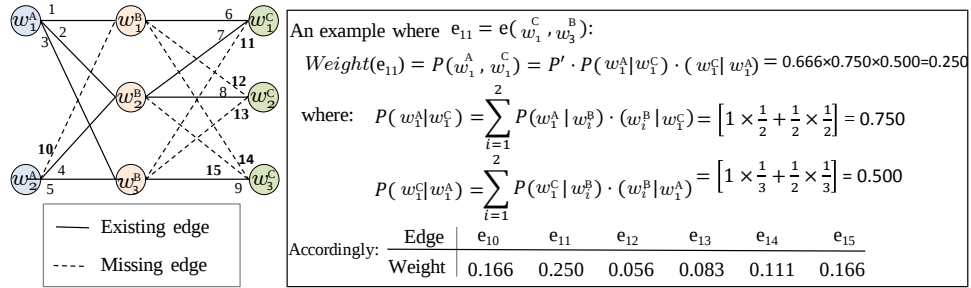
Figure 4.1: A transgraph with possible missing edges and their weights. Note that dotted lines represent the missing edges, e_{10} \sim e_{15} ; P(w_i^{l_1} | w_j^{l_2}) is the probability that w_i^{l_1} is the translation of w_j^{l_2} ; P' is the maximum probability of w_i^A or w_j^C having a one-to-one equivalent in a transgraph
