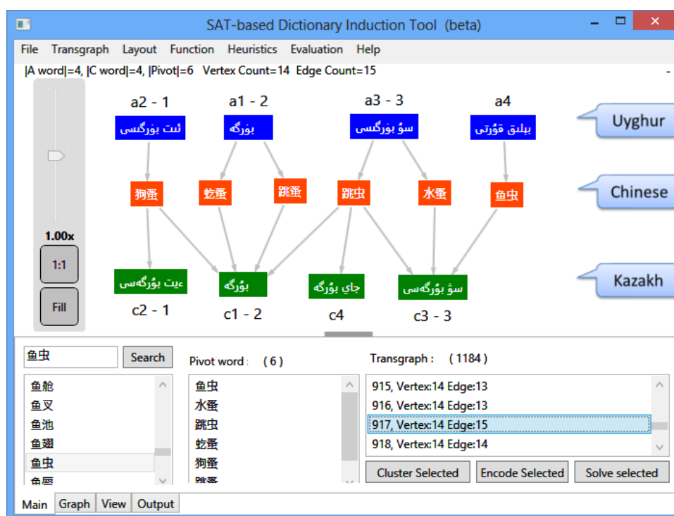
Figure 6.2: A screen-shot: evaluation of a transgraph with 14 vertices, which resulted in three one-to-one pairs with full precision and 75% recall.
