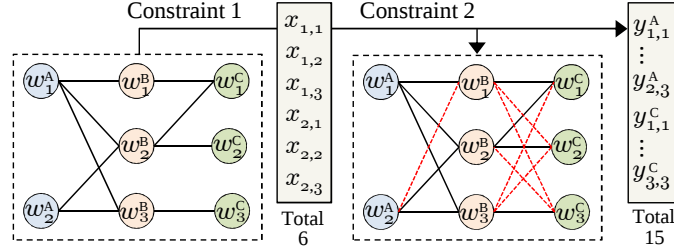
Figure 4.2: The process of creating variables for a transgraph
