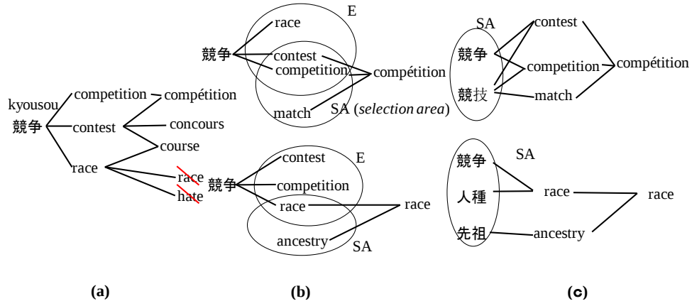
Figure 2.1: Example for Inverse Consultation method: (a) Equivalence candidates (ECs) for Japanese word “Kyouousou”; (b) One time inverse consultation ( IC_1 ); (c) Two times inverse consultation ( IC_2 ).
