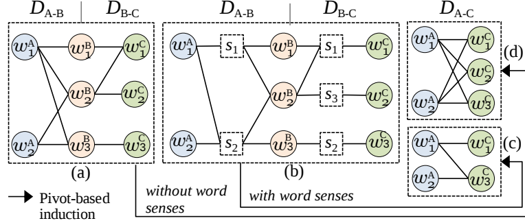
Figure 1.1: Pivot-based bilingual dictionary induction and ambiguity problem
