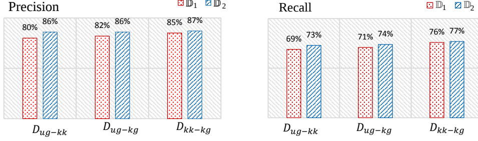
Figure 5.2: Precision and recall comparison for the cases of two and three input dictionaries
