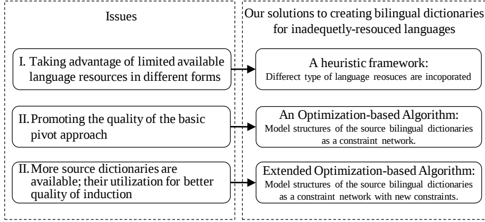
Figure 1.2: Overview of solutions to creating bilingual dictionaries for low-resource languages
