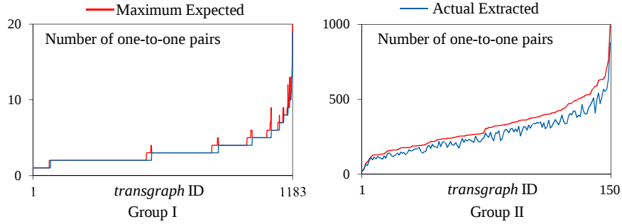
Figure 4.6: Distribution of number of maximum expected and actual extracted one-to-one pairs among ordered transgraphs in Group I & II
