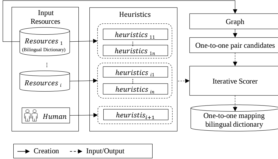
Figure 3.2: Heuristic framework for dictionary induction
