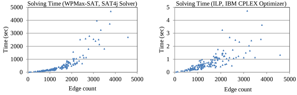
Figure 4.7: Distribution of solving time of 150 transgraphs with Max-SAT and ILP formalizations
