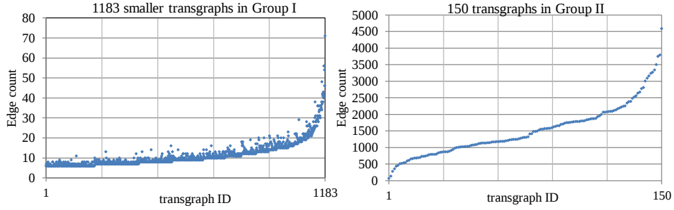
Figure 4.4: Distribution of transgraphs in Group I and Group II, which are ordered by size
