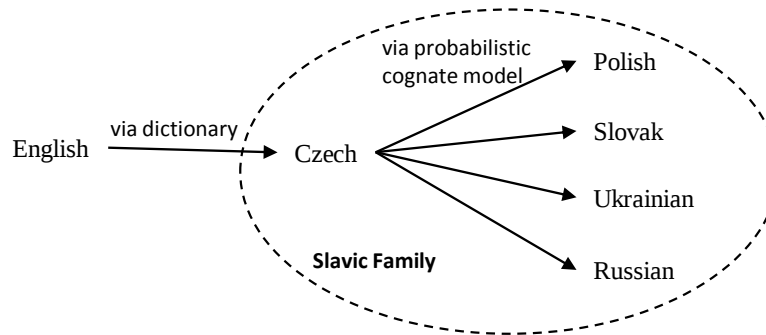
Figure 2.2: An example of bilingual dictionary induction using a pivot language
