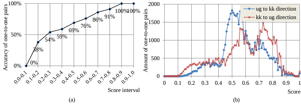
Figure 3.7: Evaluation details of the iterations II: (a) Correlation between Score Intervals and accuracy of accumulated one-to-one pairs; (b) Correlation between Score Intervals and amount of one-to-one pairs induced at each iteration
