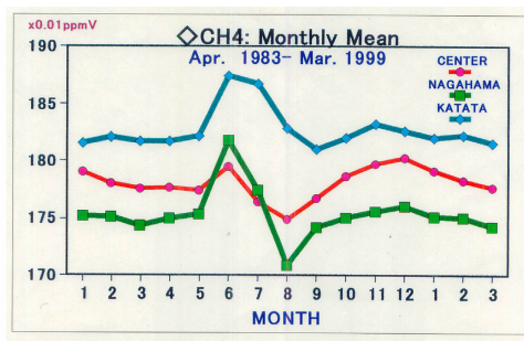
Fig. 10 Annual variation of monthly mean CH 4 at three observation sites averaged for the fiscal years 1983-1999: CENTER (Zeze, Otsu-shi), NAGAHAMA (Nagahama-shi), KATATA (Katata, Otsu-shi)
