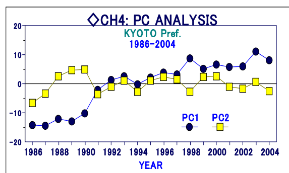
Fig. 15 Year-to-year variation of score of 1st and 2nd principal components of EOF analysis of the 1986-2004 fiscal year mean CH 4 concentration [岩嶋・森山(2007)の Fig. 20]
