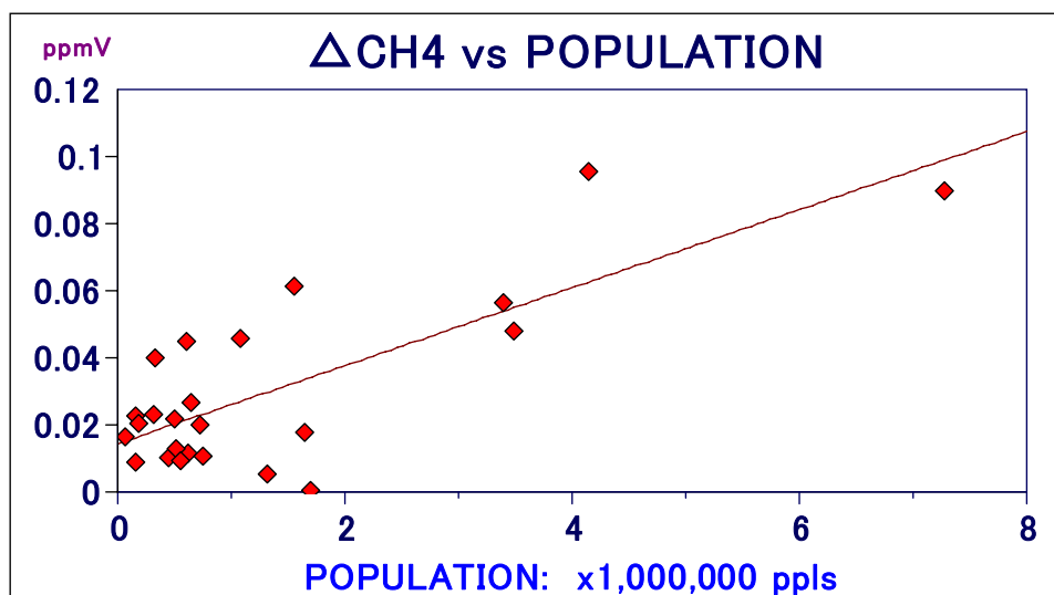
Fig. 18 Difference between \text{CH}_4 concentrations at central part and suburbs of 24 metropolises in foreign countries (Amsterdam, Zurich, Vienna, London, Edinburgh, Glasgow, Uppsala, Raykjavik, Vancouver, Victoria, Winnipeg, Ottawa, Quebec, Brisbane, Melbourne, Sydney, Berlin, Hamburg, Munich, Frankfurt, Helsinki, Oslo, Stockholm, Copenhagen): Ordinate and abscissa denote the difference of \text{CH}_4 concentrations at central part and suburbs of the cities, and population of the cities respectively.
