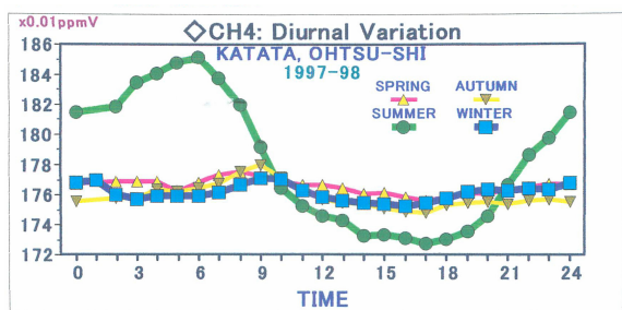
Fig. 8 Seasonal mean diurnal variation of CH 4 concentration at Katata (Honkato, Otsu-shi, Shiga-ken) [岩嶋ら(2004)の Fig. 11]
