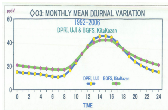
Fig. 1 Diurnal variation of the O 3 concentration observed at a) Uji (DPRI) and b) Kitakazan (BGFS; Yamashina-ku, Kyoto-shi) averaged during the years 1992-2006
