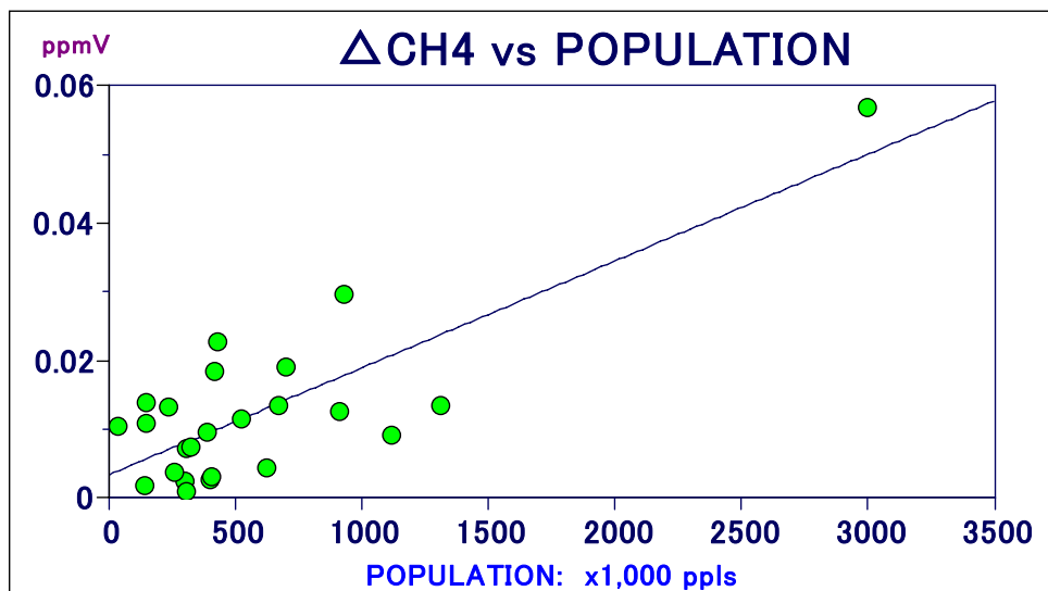
Fig. 17 Difference between \text{CH}_4 concentrations at central part and suburbs of 24 large cities in Japan (Sapporo, Hakodate, Sendai, Niiigata, Takasaki, Shizuoka, Hiroshima, Miyazaki, Okayama, Ogaki, Gifu, Chiba, Sakaiminato, Yonagao, Tottori, Naha, Kumamoto, Nagasaki, Fukuyama, Kurashiki, Wakayama, Tokushima, Kochi, Fukuoka): Ordinate and abscissa denote the difference of \text{CH}_4 concentrations at central part and suburbs of the cities, and population of the cities respectively.
