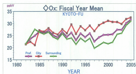
Fig. 7 Year-to-year variation of Ox for all area, the city area and the suburbs
