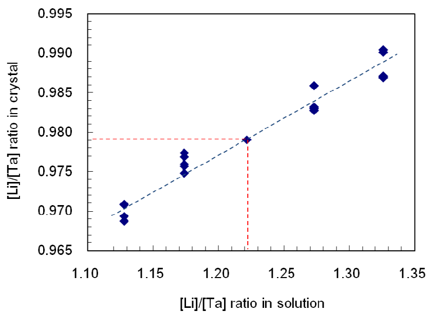
Fig. 3.6 Relationship between the [Li]/[Ta] ratios of the solution and the resultant crystals.
