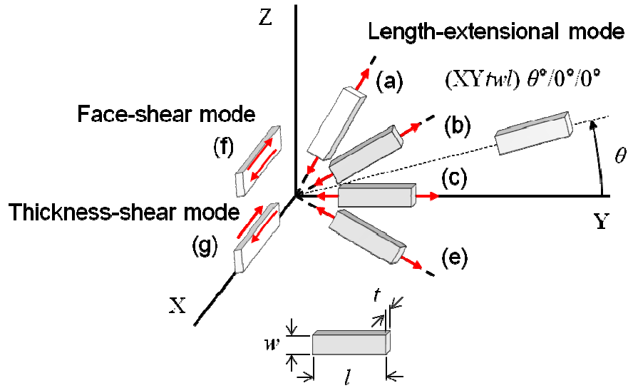
Fig. 2.4 Shapes and orientations of crystals for the investigation of material constants. Notation of (XYtwl) \theta^\circ/0^\circ/0^\circ follows the definition in Ref. [12].
