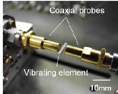
Fig. 2.5 Coaxial probes for measuring impedance characteristics.
