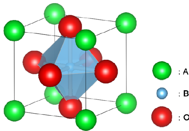
Fig. 1 Schematic illustration of the perovskite ABO_3 structure. The crystal structure was drawn with VESTA 3 [63].
