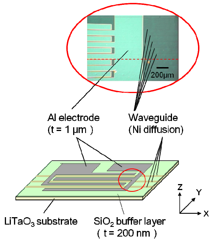
Fig. 3.20 Schematic configuration of the polarization modulator
