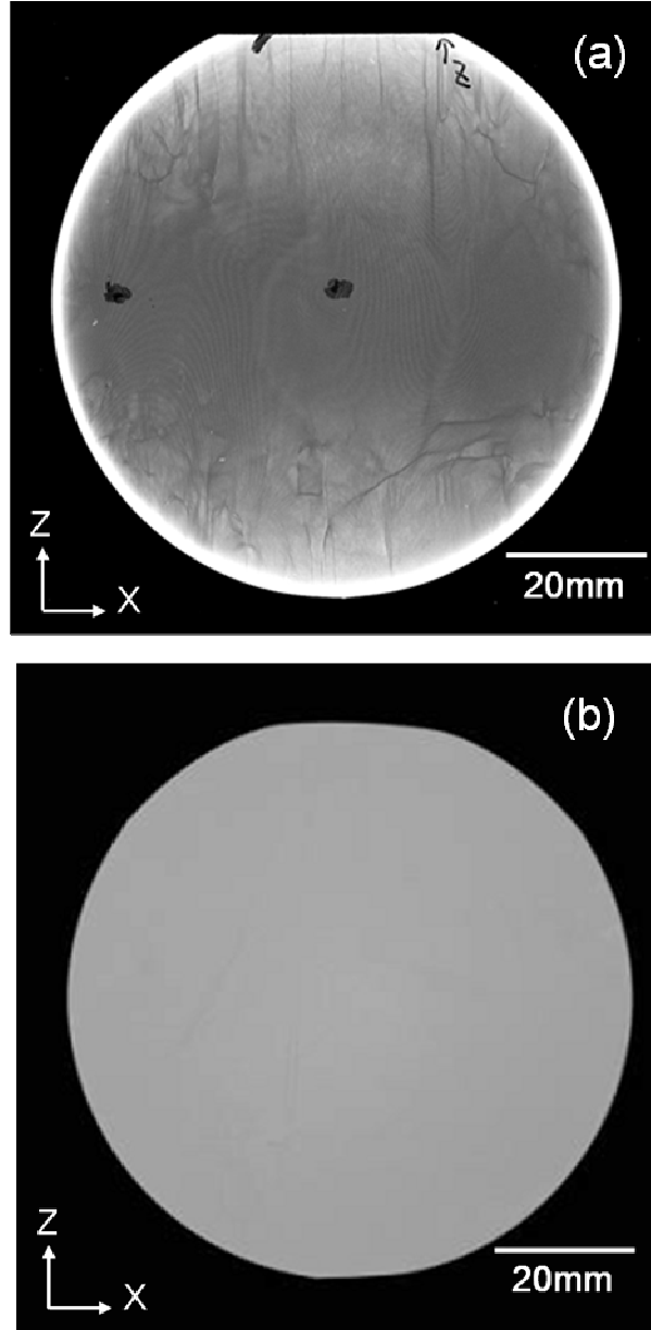
Fig. 3.12 Cross-nicol images of the zero-birefringence LiTaO 3 wafers cut from the body part of the boule: (a) crystal grown at the early stage and (b) crystal grown under optimized conditions.
