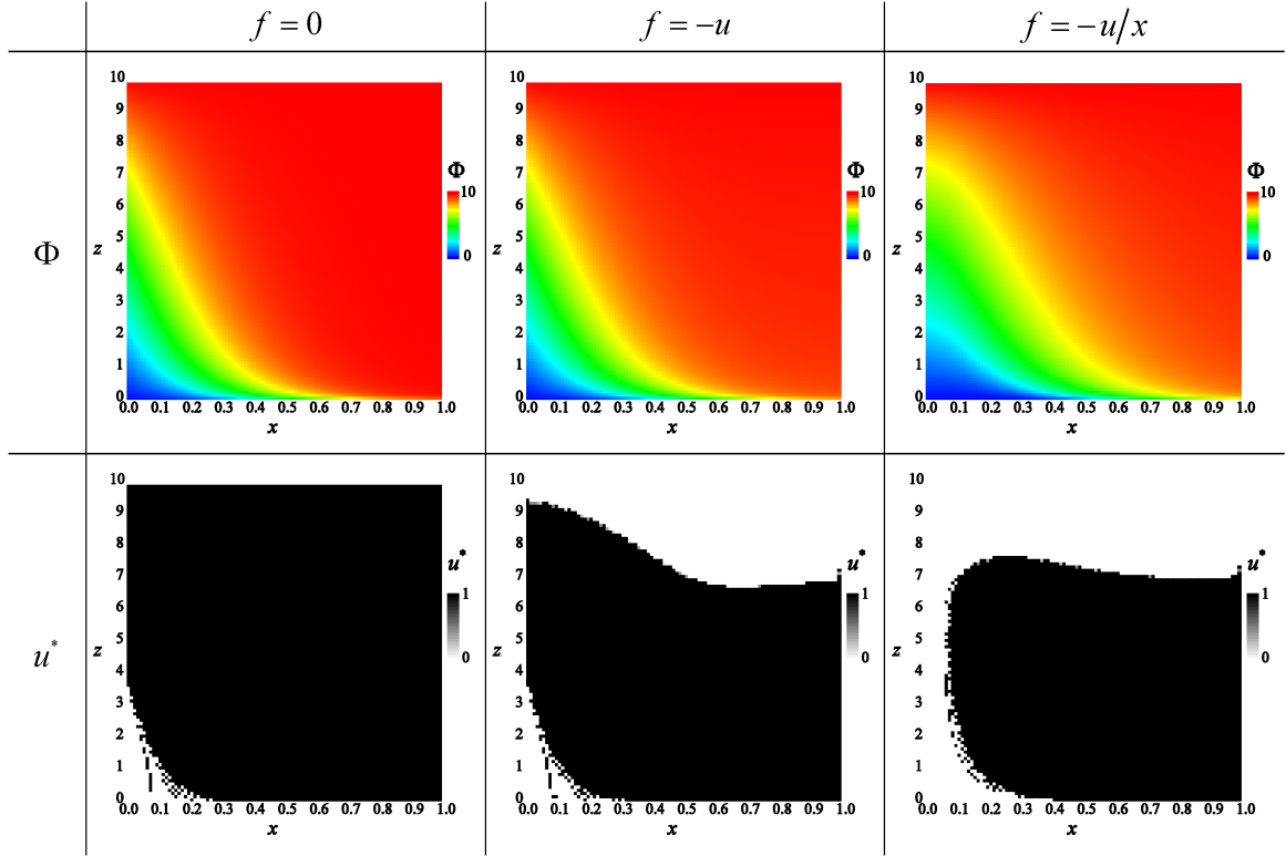
Fig. 2 Computed \Phi and u^* for different benefit functions at t = 0
