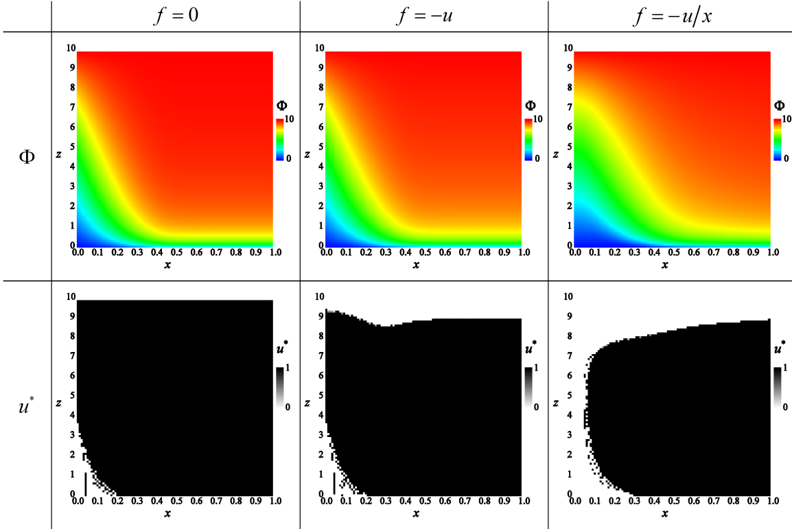
Fig. 4 Computed \Phi and u^* for different benefit functions at t = 60
