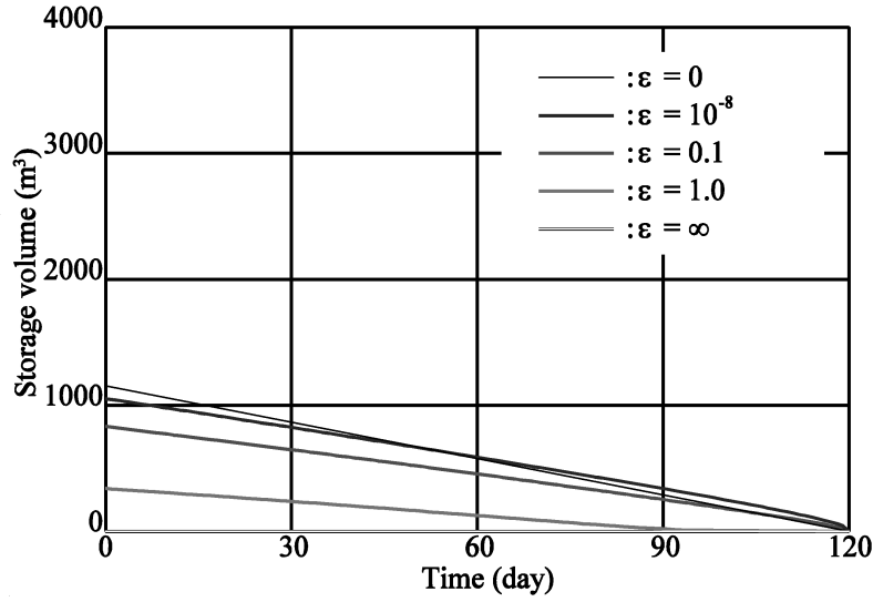
Fig. 1 The rule curves for different \varepsilon values (Unami et al. 2015)
