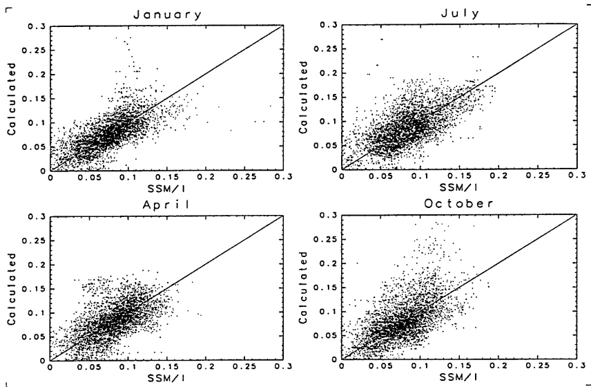
Fig. 3 Correlation of liquid water path between SSM/I Database and calculated (Unit: \text{kg}/\text{m}^2 )
