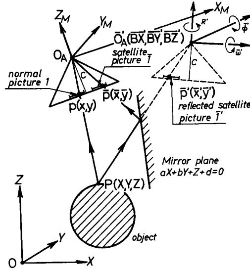
Fig. 4 The orientation problem of a stereopair of normal and satellite pictures 1 and \bar{I} for the case of using a camera and a plane mirror. The six exterior orientation parameters ( \bar{\omega}' , \bar{\phi}' , \bar{\kappa}' , \bar{B}\bar{X}' , \bar{B}\bar{Y}' , \bar{B}\bar{Z}' ) of the reflected satellite picture \bar{I}' are newly defined with respect to the model space coordinate system ( X_M , Y_M , Z_M ).
