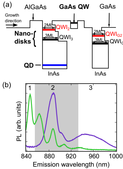
FIG. 1. (Color online) (a) Conduction-band diagram of sample structure. Growth proceeds from left to right. On top of a GaAs substrate, an InAs/AlGaAs layer with shallow 2 ML nanodisk states ( \text{QWI}_2 , red), 3 ML nanodisk states ( \text{QWI}_3 , black) and deep QD states (blue) was grown. Then a GaAs QW was inserted for upconverted PL measurements. The top consists of an InAs/GaAs layer with the intermediate 2 ( \text{QWI}_{G2} ) and 3 ML ( \text{QWI}_{G3} ) nanodisk states indicated in red and black, respectively. (b) Stokes \mu\text{PL} spectra at selected points for excitation at 835 nm. Regions 1 and 3 correspond to spectral regions containing \text{QWI}_2 and QD states, respectively. Region 2 is explained in the text. The peak assignments are summarized in Table I.
